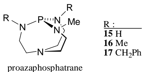
Figure 1.32 : Structures des proazaphosphatranes 15-17
