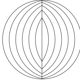
FIGURE 4.2 – Level sets of the z function
