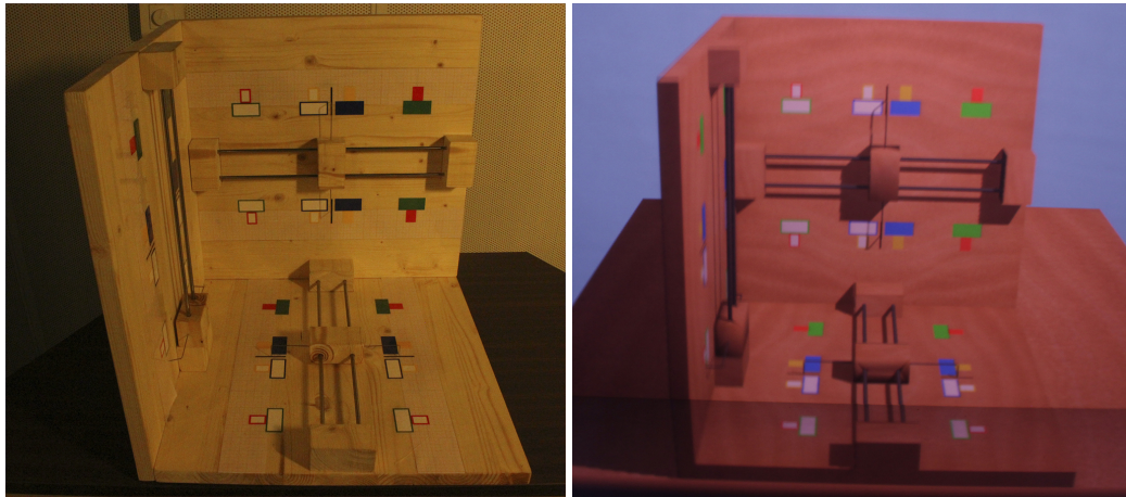
Figure 5.6: 1 degree of freedom translations. Left: physical device. Right: virtual device.
