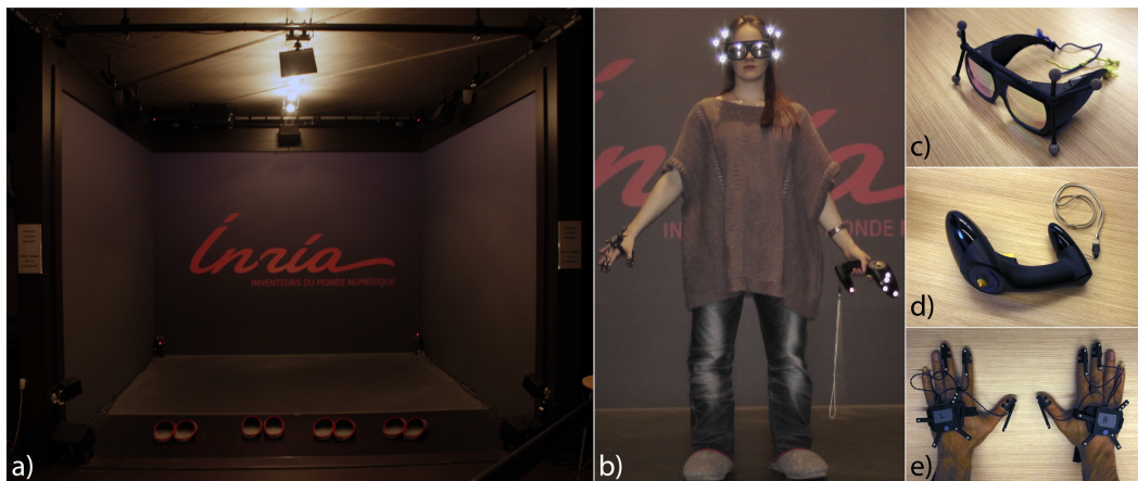
Figure 3.1: Experimental setup. The four-sided immersive cube is shown in a) with eight infrared cameras and surround sound. In the middle, b) a user wears the tracked input devices which are: c) Infitec glasses with frame, d) ART flystick and e) ART finger tracking gloves.
