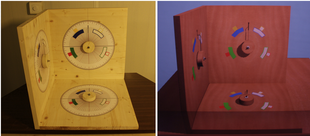
Figure 5.8: 1 degree of freedom rotations. Left: physical device. Right: virtual device.
