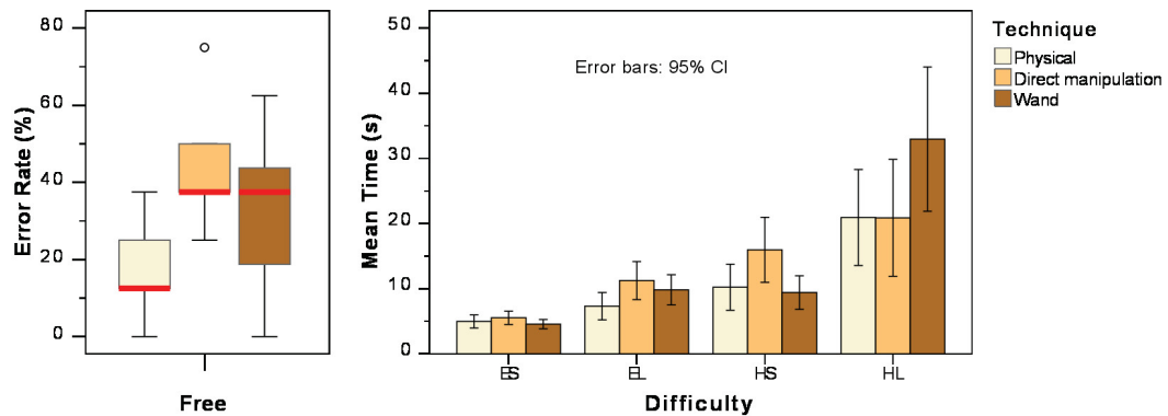
Figure 5.20: Performance results for the free movement task. Left: error rate. Right: completion time.
