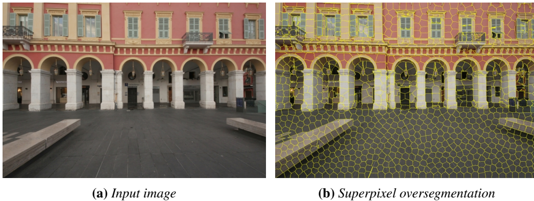
Figure 6.4: Superpixel oversegmentation.
