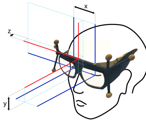
Figure 4.10: The position of the user's eyes is calibrated in the three dimensions.
