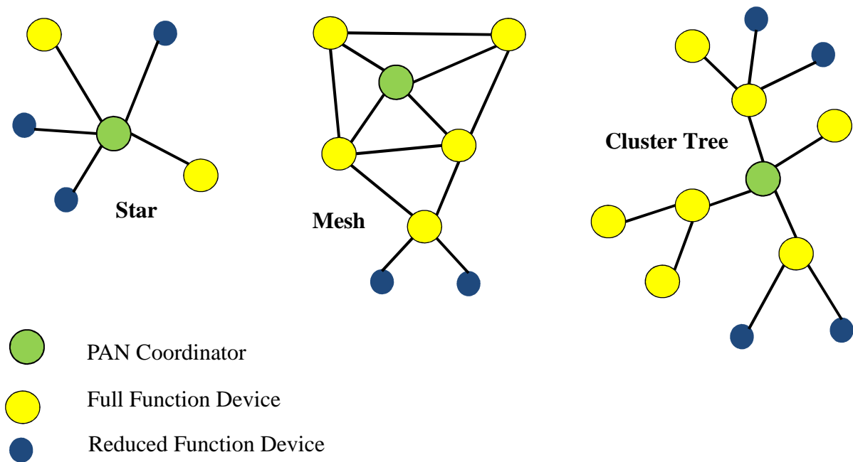
Figure 10. ZigBee topologies
