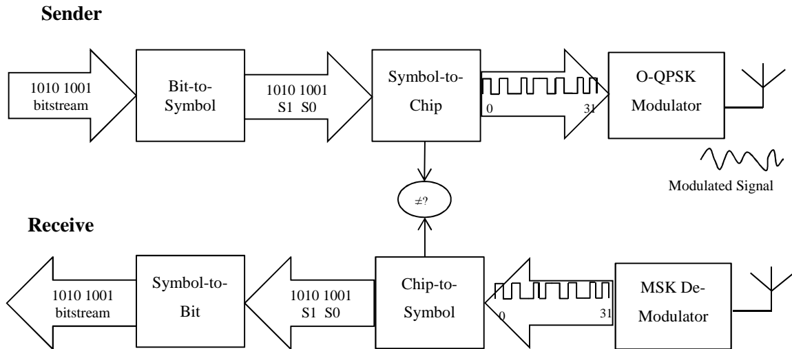
Figure 4. Modulation and spreading functions for the O-QPSK PHYs
