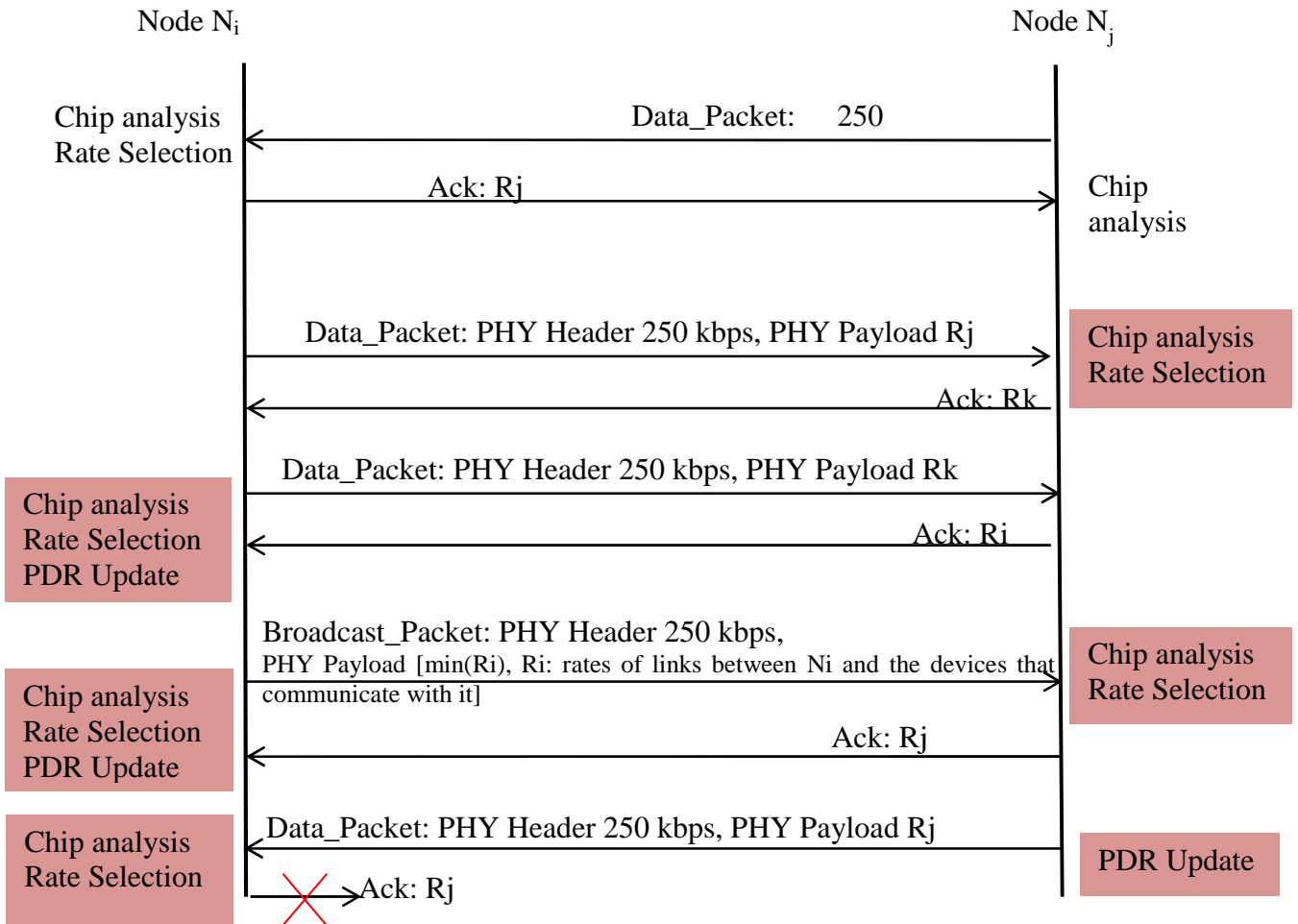
Figure 51. Data rate adaptation during packet exchange
