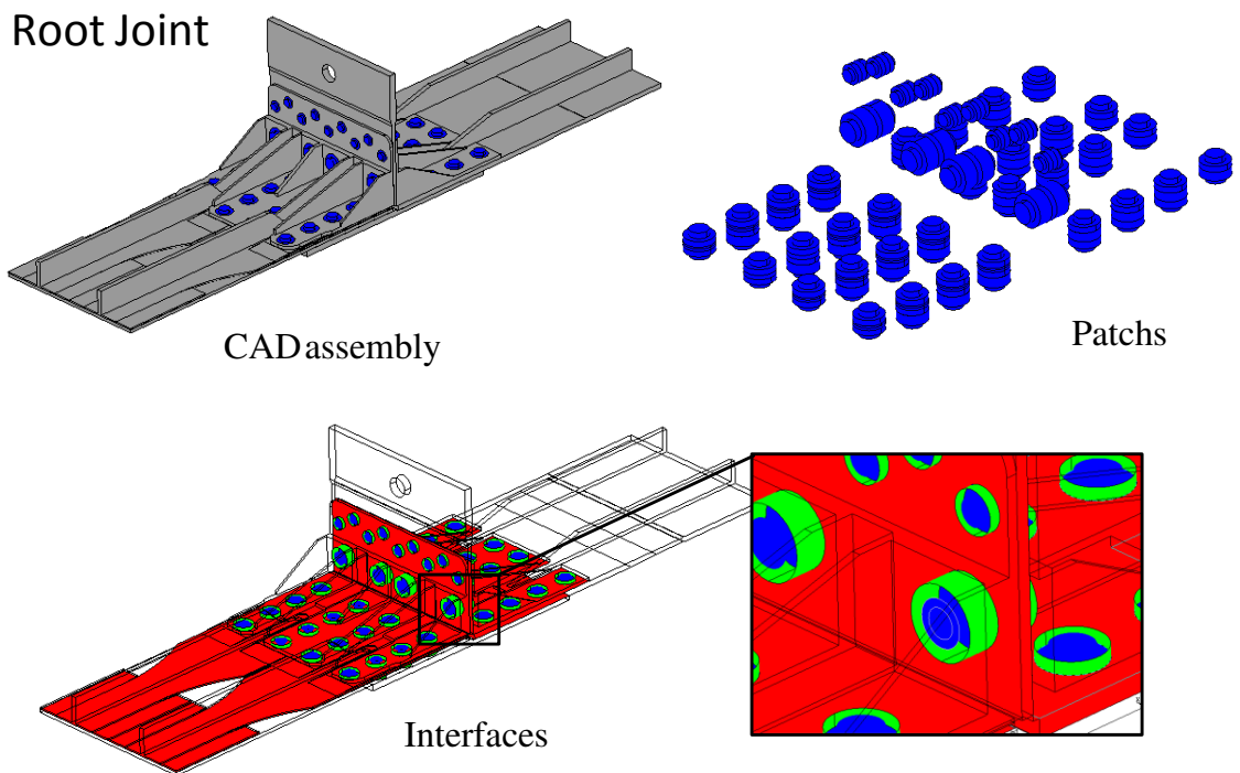
Figure D.5: Illustration of the STEP export of the full Root Joint assembly.
