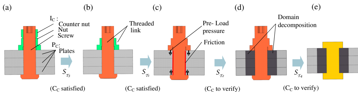
Figure 6.10: Compatibility conditions ( C_C ) of shape transformations S_{\mathcal{T}} applied to T . (a) through (e) are different configurations of C_C addressed in Section 6.3.3.
