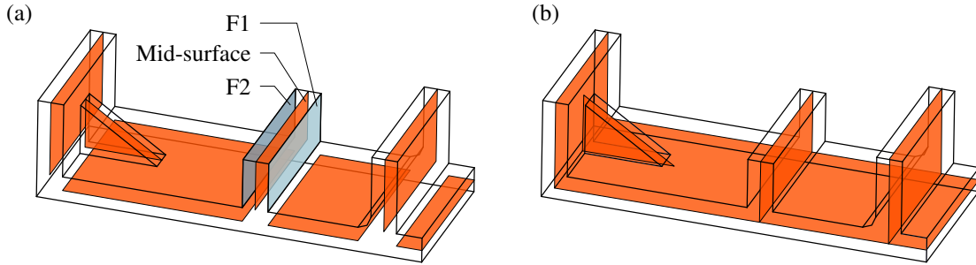
Figure 2.7: Illustration of mid-surface abstraction [Rez96], (a) creation of mid-surfaces from face-pairs, (b) connection of mid-surfaces to generate a fully idealized model.
