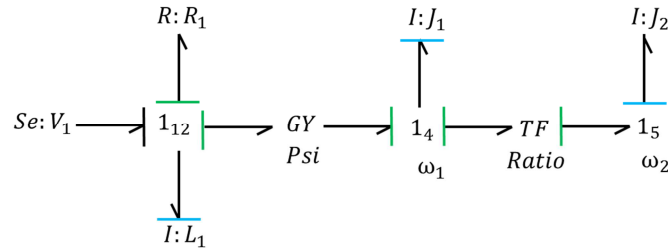
Figure 79. Bond graph causal obtenu au second tour
