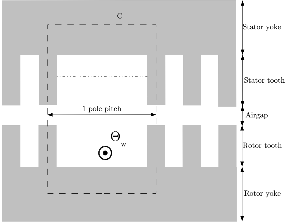
Figure 2.1: Magnetic circuit
