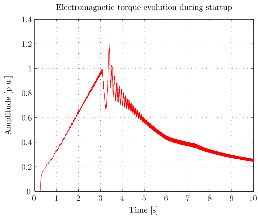
Figure 5.61: Startup: Electromagnetic torque
