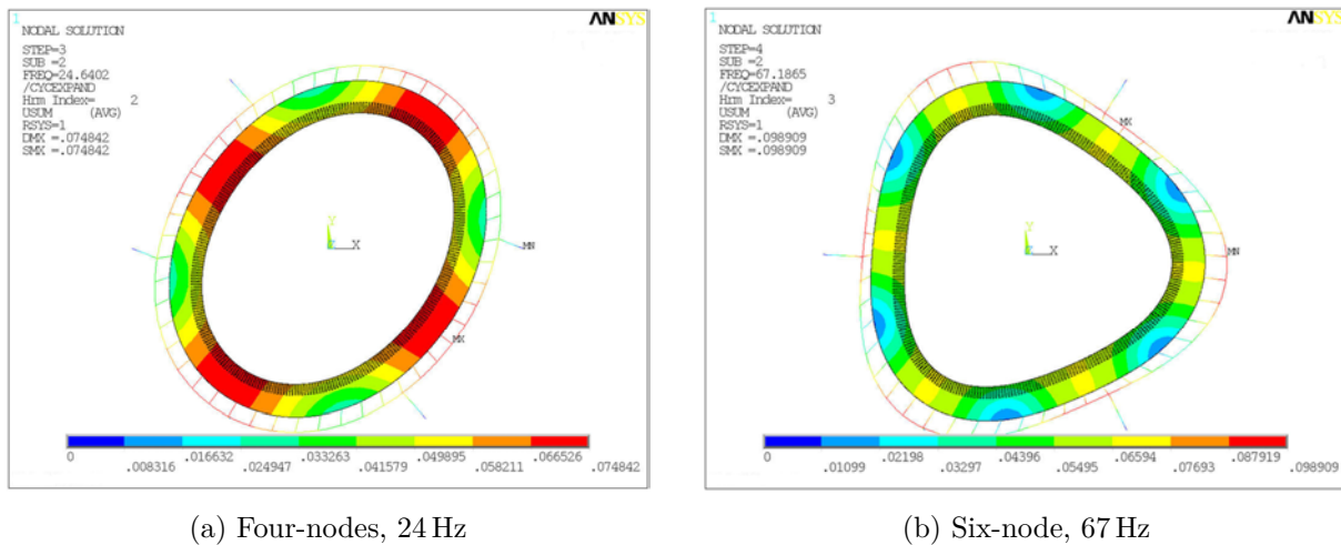
Figure 5.26: Examples stator structure eigen-modes [Car12b]
