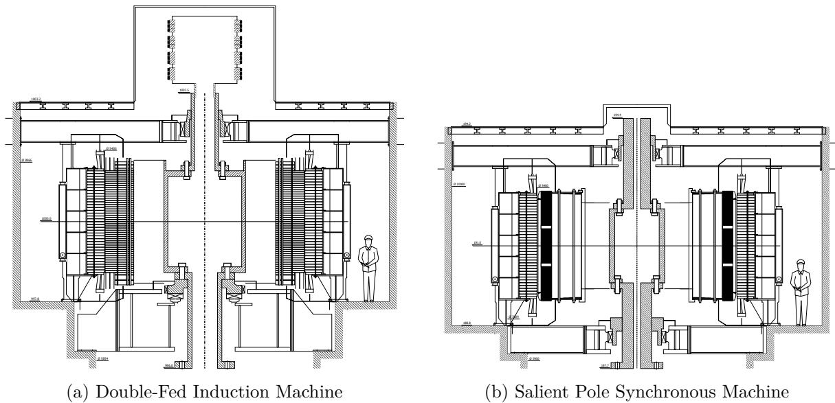
Figure 1.16: Longitudinal section of the two machines (from Alstom design tool)
