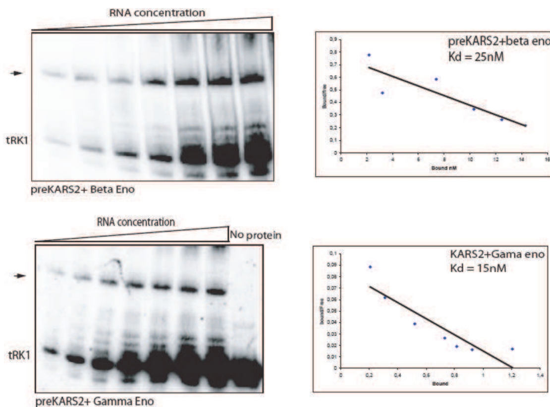
Figure 19: Interaction between labeled tRK1 and preKARS2 in the absence or presence of human enolases. Interaction of ^{32}\text{P} -labeled tRK1 (2-30 nM) with preKARS2 (0.8 μM) in the absence or presence of human enolases (1 μM) using electrophoretic mobility shift assay. (A) Scatchard plot determination of preKARS2-tRK1 complex in the absence of enolases. (B) Scatchard plot determination of preKARS2-tRK1 complex in the presence of different isoforms of human enolases (1 μM). The RNA in complex with protein was separated from unbound RNA by native gel electrophoresis. The bottom band corresponds to the free RNA species; RNA-protein complex is shown with an arrow.
