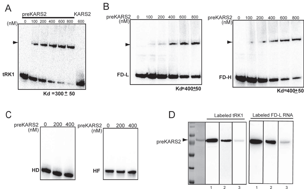
Figure 2. Interaction of the purified KARS2 and preKARS2 proteins with RNAs tested by EMSA. After incubation of ^{32} P-labeled tRK1 (A), FD-L and FD-H RNAs (B) or the truncated HD and HF RNAs (C) with increasing concentrations of the recombinant proteins (indicated above the panels, in nM), the complex formation was visualized by autoradiography. In each assay, the bottom band corresponds to the free RNA species, the RNA-protein complex is marked with an arrowhead. The deduced dissociation constants ( K_d ) for each RNA are given at the bottom of the panel (in nM). A representative of at least three independent experiments is shown for each RNA. (D) North-Western hybridization. Membrane stripes, containing equal amounts of preKARS2, were incubated with labeled RNAs (indicated above). Lane 1, no competitor added; lane 2, hybridization in the presence of 30\times molar excess of nonspecific competitor (rRNA E. coli ); lane 3, hybridization in the presence of 10\times molar excess of nonlabeled RNA FD-R. Left panel represents the membrane stained with Ponceau Red. doi:10.1371/journal.pone.0066228.g002
