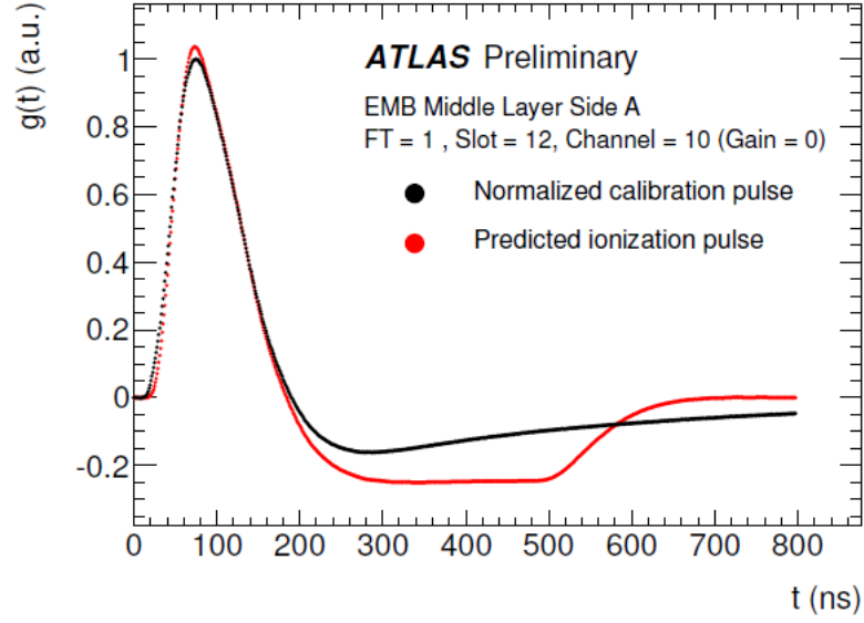
Figure 3.6: Comparison between the calibration (black) and physics pulse (red) for a middle cell in the EM barrel [42].
