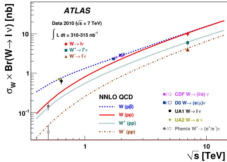
Figure 1.9: Measured values of W cross-sections at TeVatron, Sp\bar{p}S , RHIC and ATLAS experiments compared to the NNLO prediction as a function of the centre of mass energy [27].
