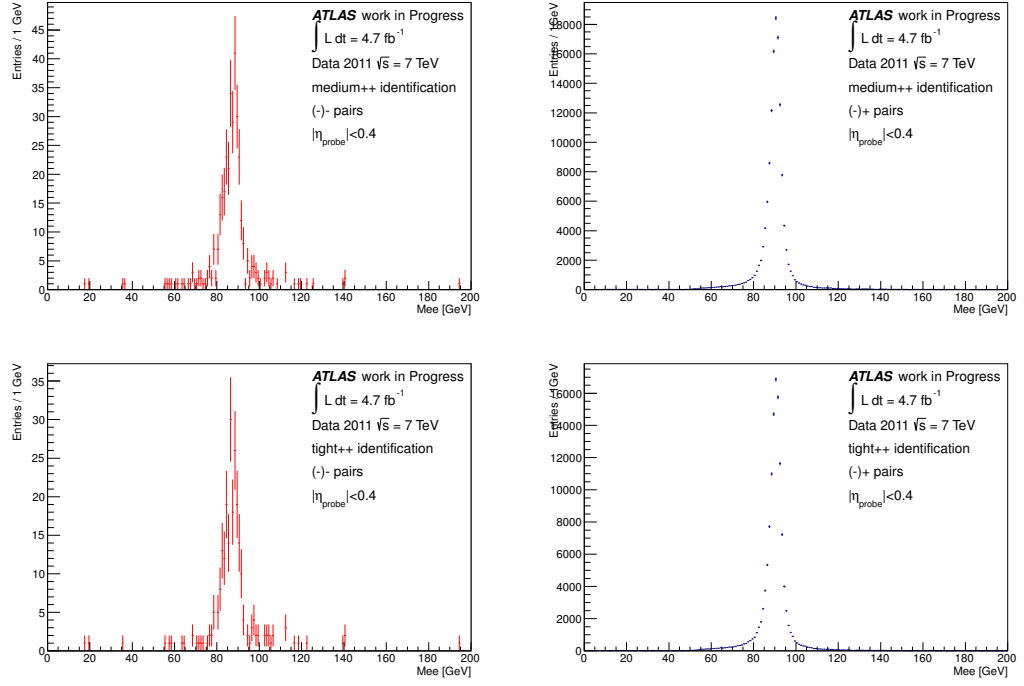
Figure 4.8: Top row: The tag-probe mass distribution for probe electrons* passing the medium++ identification level with |\eta_{\text{probe}}| < 0.4 is shown for SS pairs (tag electron, probe electron) in the left plot and for OS pairs (tag electron, probe positron) in the right plot; Bottom row: Same distributions for probe electrons* satisfying the tight++ identification requirements. The shoulder seen at \sim 60 GeV is caused by the kinematic cuts applied on the electron* selection.
