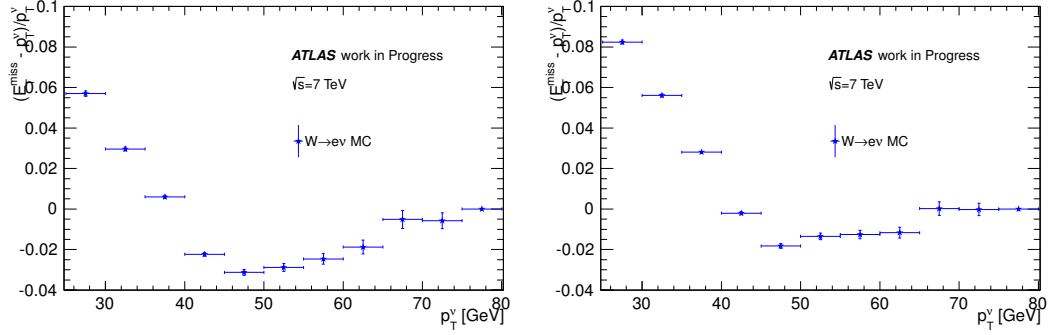
Figure 4.26: E_T^{\text{miss}} linearity as a function of p_T^{\nu} measured on W \rightarrow e\nu events. The left plot represents low pile-up conditions while the right plot high pile-up conditions. The linearity of E_T^{\text{miss}} is shifted to higher values for high pile-up conditions.
