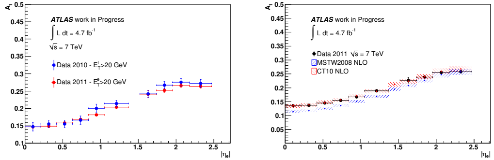
Figure 6.15: Left: W charge asymmetry measured using the 2010 (blue) and 2011 (red) data respectively extrapolated to the same fiducial region. The 2010 measurement represents the combined electron and muon asymmetry measurements while the 2011 analysis includes only the electron measurement. Right: Comparison of the 2011 measurement to the theoretical prediction of MC@NLO using the MSTW2008 and CT10 PDFs at NLO.
