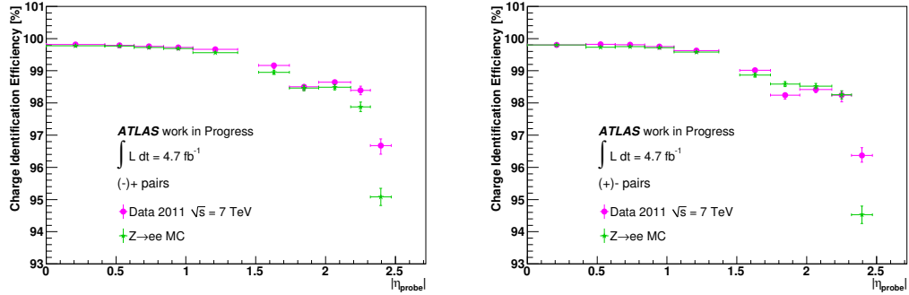
Figure 4.20: Plots showing the data - Monte Carlo comparison at tight++ level for (a) charge identification using (-)+ pairs [the brackets indicate the sign of the tag]; (b) charge identification using (+)- pairs.
