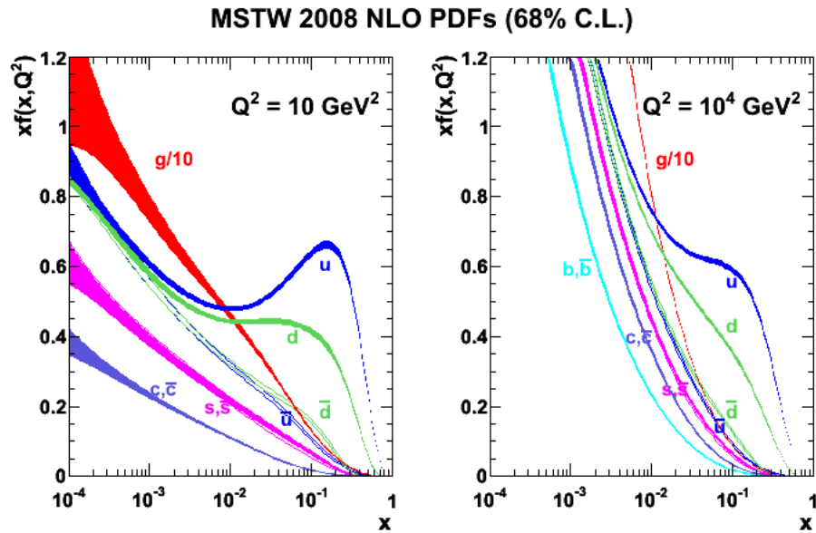
Figure 1.6: Parton distribution functions of the proton at next-to-leading order (NLO) for two different scales Q^2 as predicted by the MSTW collaboration. The band represents the 68% confidence level [15].
