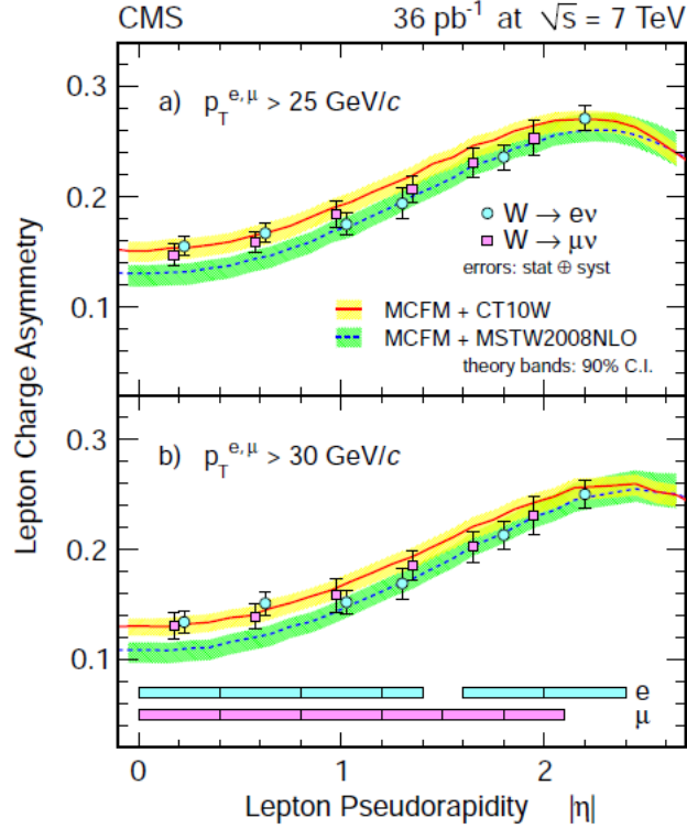
Figure 6.16: CMS results showing the comparison of the measured lepton charge asymmetry to different PDF models for lepton p_T > 25 GeV/c ( top ) and lepton p_T > 30 GeV/c ( bottom ). The error bars include both statistical and systematic uncertainties. The PDF uncertainty band is corresponding to the 90% confidence interval (C.I.). The bin width for each data point is shown by the filled bars on the bottom. The data points are placed at the centre of pseudorapidity bins, except that for display purposes the first three data points are shifted +0.025 ( -0.025 ) for electrons (muons) [59].
