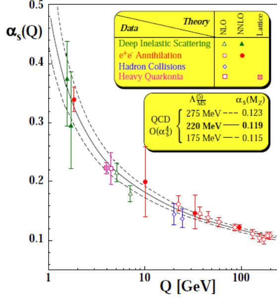
Figure 1.2: Measurements of the strong coupling constant \alpha_s as a function of the energy scale from a number of different experiments [6].
