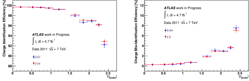
Figure 4.13: Left plot: Comparison between charge identification (OS measurement) for electrons (blue) and positrons (red) passing the loose++ identification; Right plot: Charge misidentification (SS measurement) for electrons and positrons at loose++ level.
