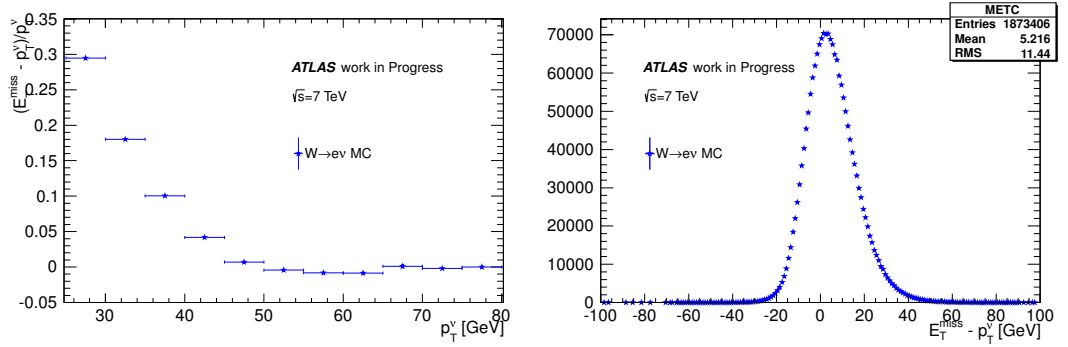
Figure 4.27: E_T^{\text{miss}} linearity (left) and resolution (right) after a selection including electron, E_T^{\text{miss}} and m_T^W requirements. Compared to Fig. 4.25 it is evident that the E_T^{\text{miss}} linearity is highly affected by the additional selection criteria. This is also seen in the right plot where the mean of the distribution is also shifted. The resolution of the E_T^{\text{miss}} is not significantly affected.
