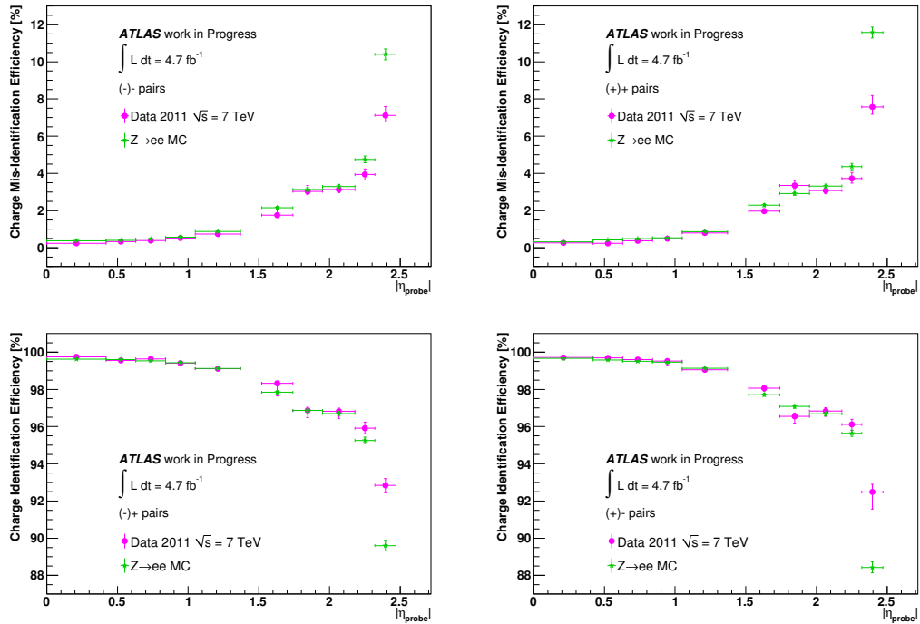
Figure 4.11: Plots showing the data - Monte Carlo comparison at track quality level for (a) charge misidentification using (-) pairs [the brackets indicate the sign of the tag]; (b) charge misidentification using (+) pairs; (c) charge identification using (-)+ pairs; (d) charge identification using (+)- pairs.
