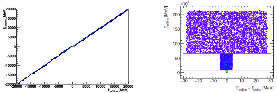
Figure 3.7: Example of validation plots from events generated by the DspTest code. E_{\text{online}} is the cell energy computed by emulating the DSP response and E_{\text{offline}} the energy computed with full precision.
