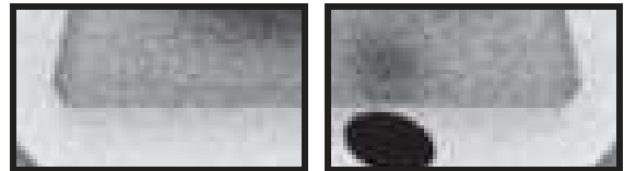
FIGURE F.9 – A dielectric glass plate ( n = 1.5 ) with isotropic Beckmann roughness ( \alpha = 0.8 ) on all faces (with the Smith masking function).
