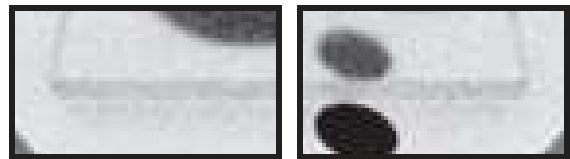
FIGURE F.12 – A dielectric glass plate ( n = 1.5 ) with isotropic GGX roughness ( \alpha = 0.1 ) on all faces (with the Smith masking function).
