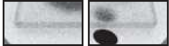
FIGURE F.8 – A dielectric glass plate ( n = 1.5 ) with isotropic Beckmann roughness ( \alpha = 0.4 ) on all faces (with the Smith masking function).
