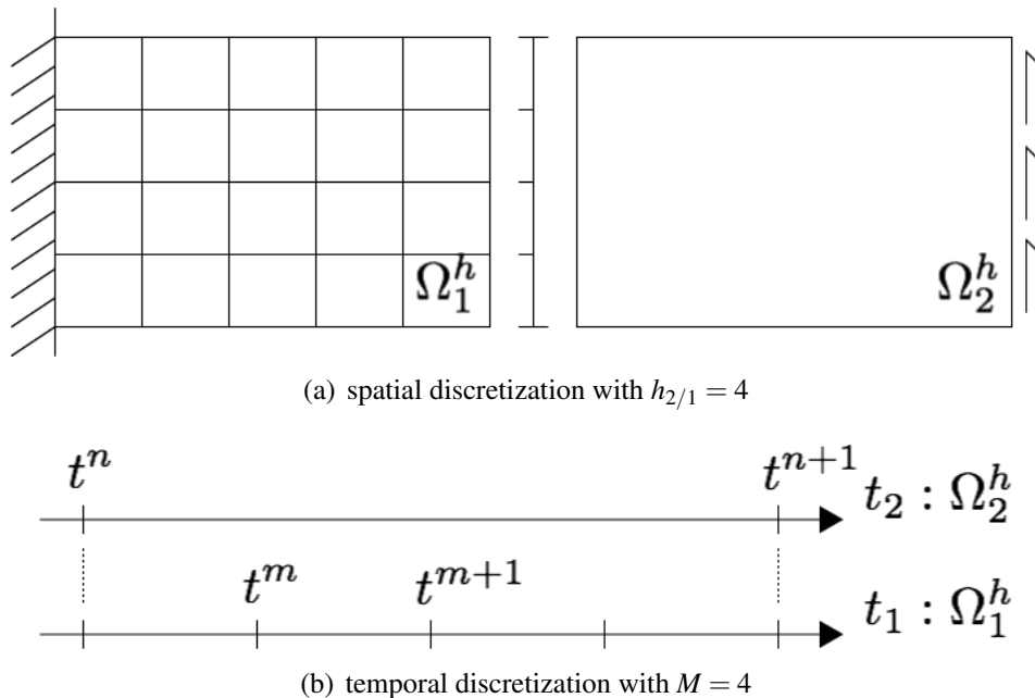
Figure 2.2: Discretization for non-overlapping Domain Decomposition.
