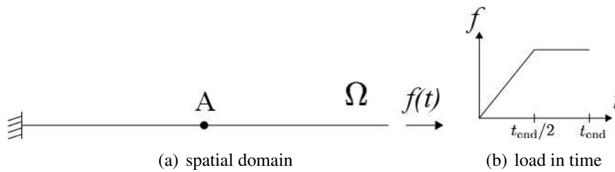
Figure C.1: Truss test example: boundary conditions, load and monitored location A.
