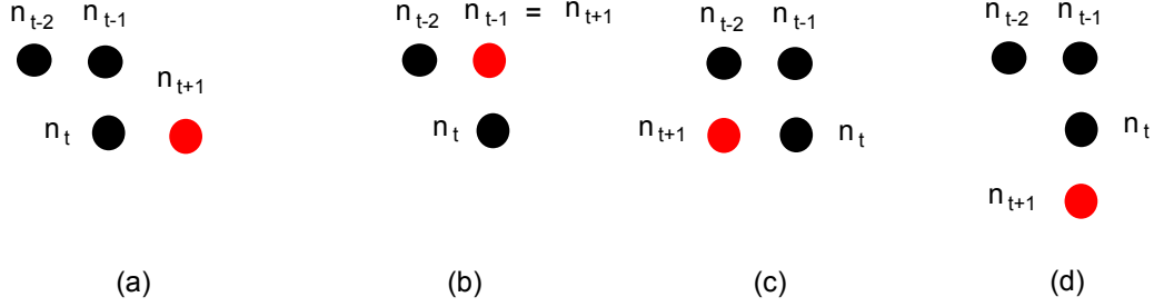
Figure 7.7: The 4 possible positions of n_{t+1} for the configuration present in Figure 7.4 (b).
