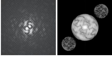
Fig. 1. Intensity of the speckle field (simulation) in the focal plane of an SCC ( left ) and its Fourier transform ( right ) for monochromatic light.
