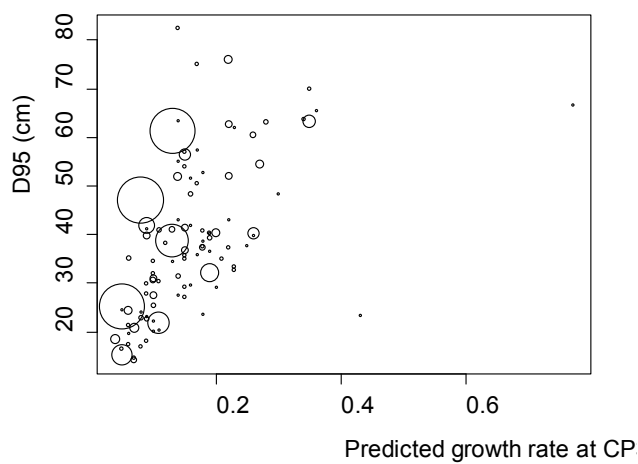
Figure 18. Relationship between predicted growth rate at CP3 (cm.y -1 ) and species D95 (cm) at the Paracou experimental site. Symbol size is proportional to species abundance.
