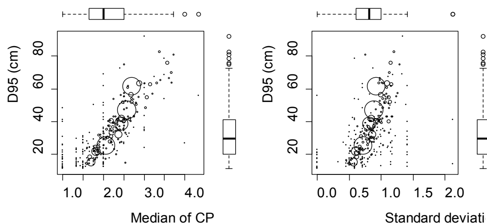
Figure 14. Relationship between species median and standard deviation values for CP and species D95 (cm) at the Paracou experimental site. Symbol size is proportional to species abundance. For 28 of the 282 species (10%) and 5409 of the 13510 trees (40%), the DBH or log DBH model parameter was significantly (significance level=5%) different from the species mean species (Table 13 en annexe).
