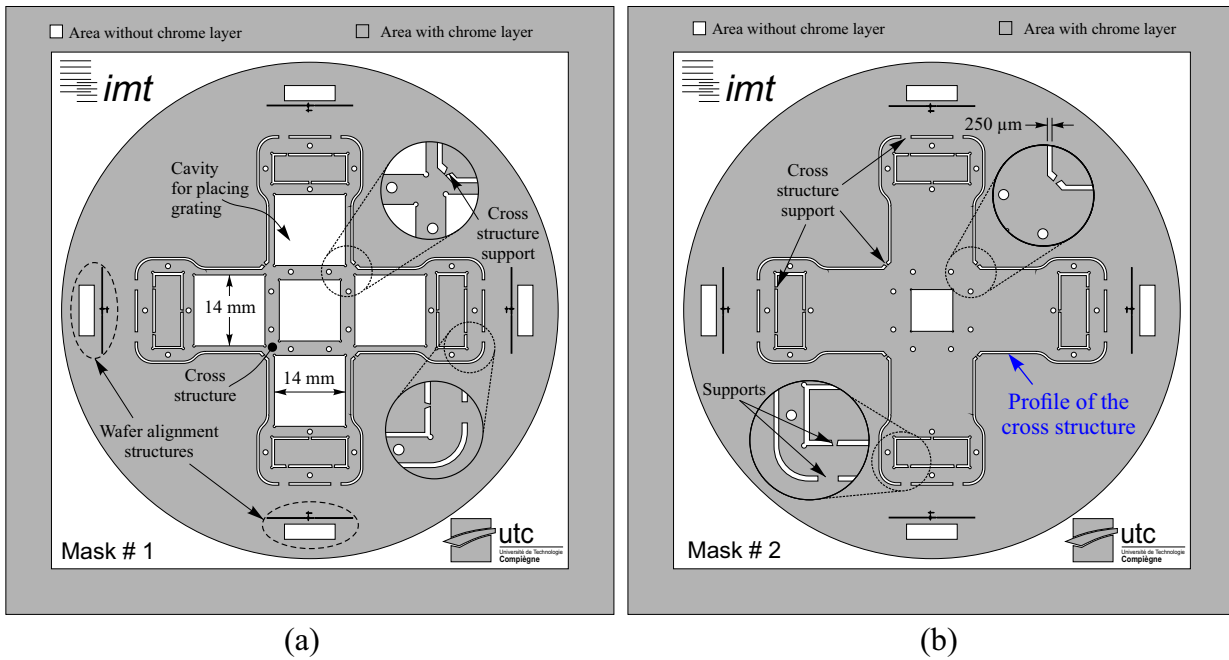
FIGURE 5.2: Design layout of the (a) top side mask (b) bottom side mask
