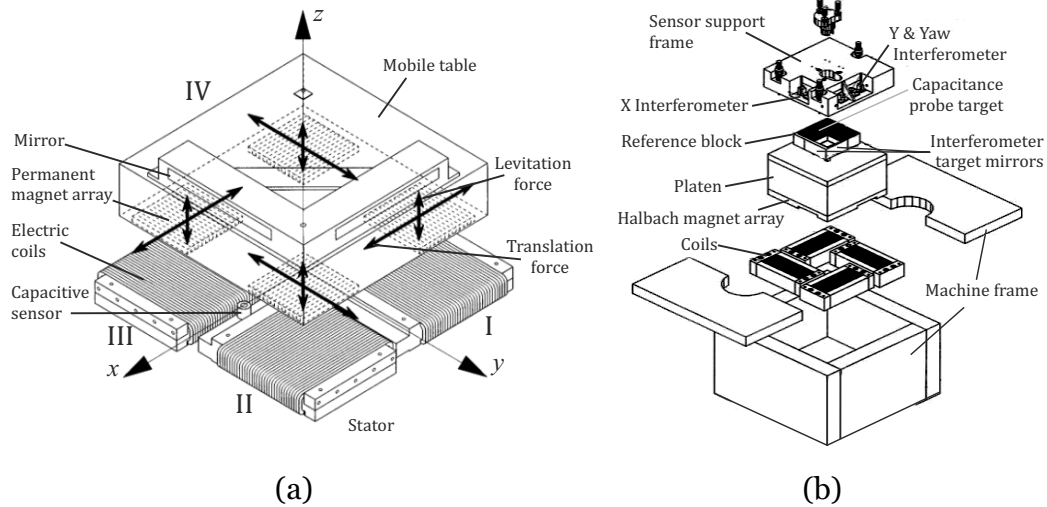
FIGURE 1.25: Maglev positioning systems developed by (a) Trumper et al. , [Trum 98] (b) Holmes et al. , [Holm 00]
