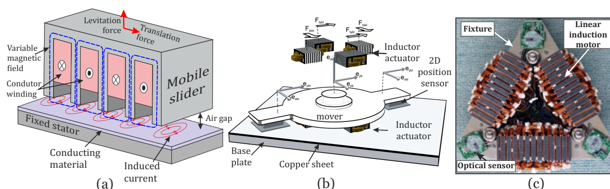
FIGURE 1.19: (a) LIA principle (b) Dittrich et al. , [Ditt 06] (c) Kumagai et al. , [Kuma 12]
