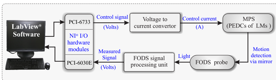
FIGURE 3.18: Schematic layout of the experiment
