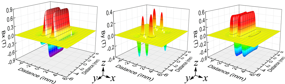
FIGURE 2.16: Reduction of single PM into equivalent current distribution
