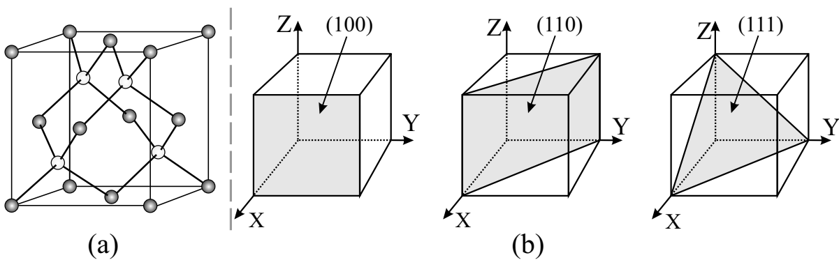
FIGURE 4.15: (a) FCC structure of the silicon (b) Different crystallographic planes in silicon crystal [Rive 04]
