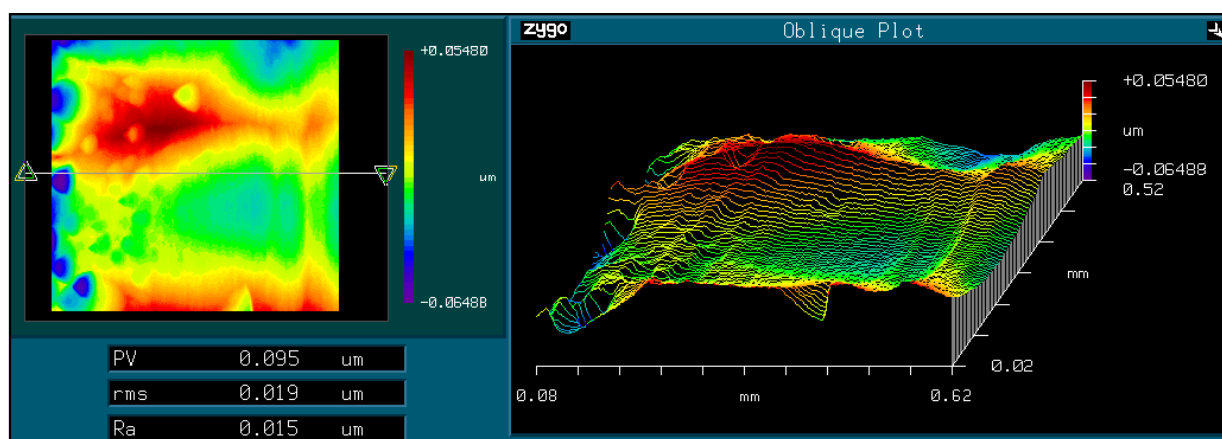
FIGURE 4.23: An image of a single measurement zone on the gold coated silicon grating step measured using Zygo™200 interferometer machine
