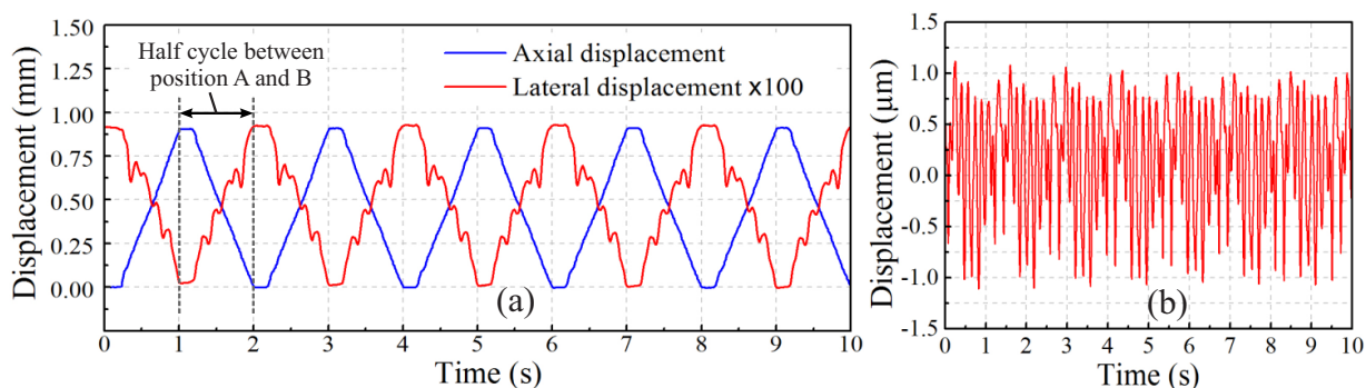
FIGURE 3.24: Rectitude of the MPS in linear motion (a) Axial and lateral displacement (b) Real lateral displacement
