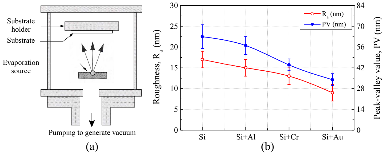
FIGURE 4.31: (a) Evaporation process in vacuum [Dani 04] (b) R_a and PV values with different metal coating
