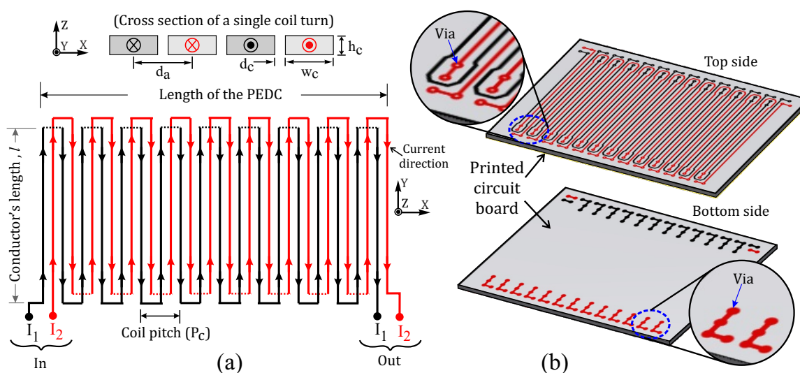
FIGURE 2.7: (a) Two phase coil and cross sectional view (b) PCB model of a PEDC
