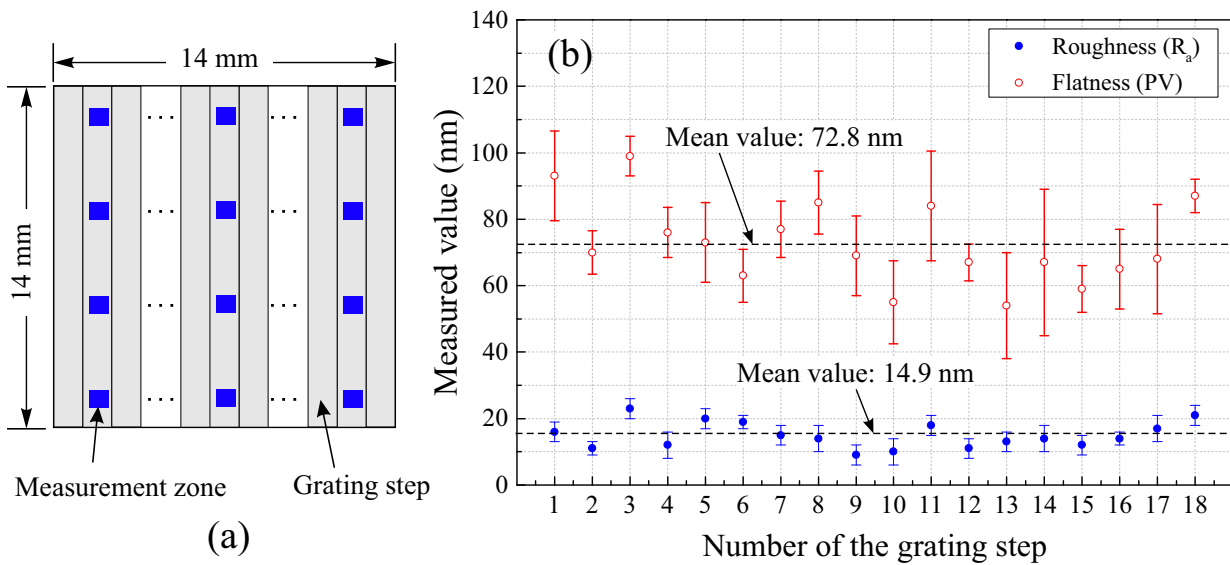
FIGURE 4.24: (a) Measurement zones (b) R_a and PV values over each grating step
