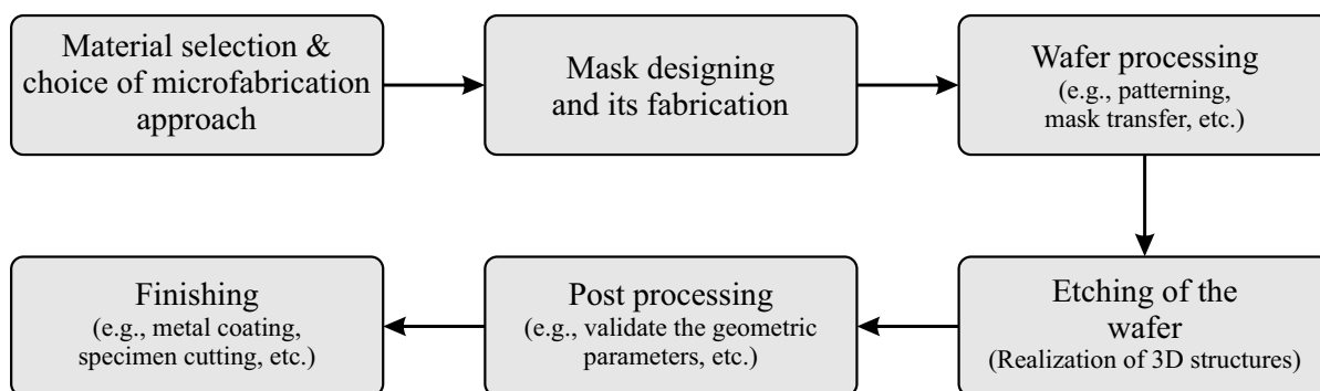
FIGURE 4.13: Schematic layout of the overall microfabrication process
