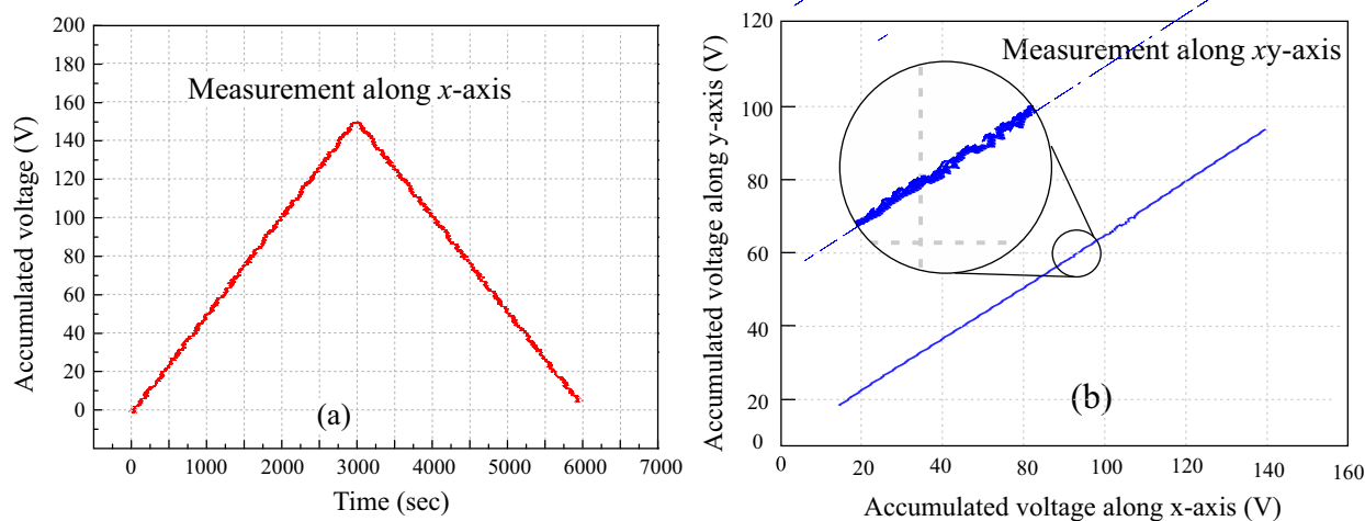
FIGURE 5.10: Open loop response along x -axis and y -axis
