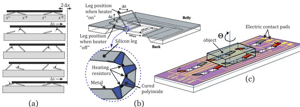
FIGURE 1.12: (a) Actuation principle (b) Single silicon leg (c) Micro conveyor [Ebef 00]
