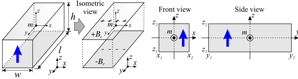
FIGURE 2.14: Reduction of a single PM to equivalent magnetic charge distribution and its 2D representation in reference frame
