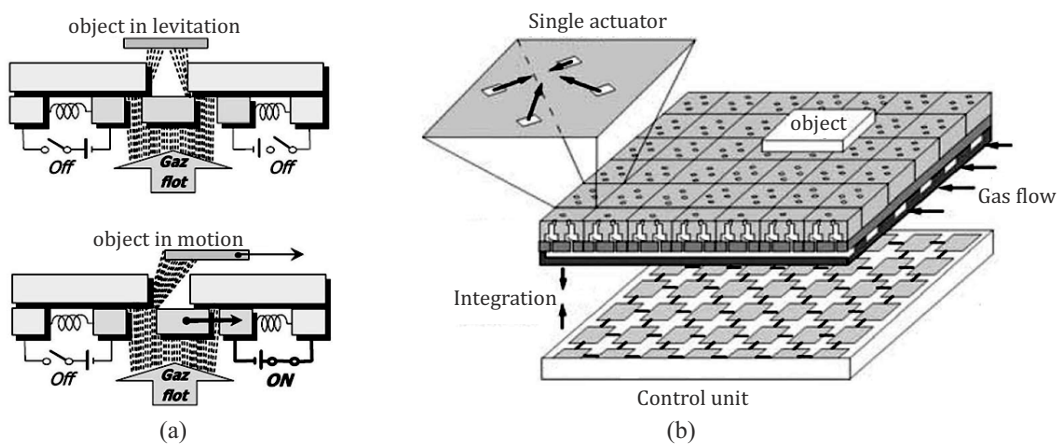
FIGURE 1.13: Distributed conveyance system [Chap 04] (a) Object in levitation and motion states (b) MEMS actuators assembly
