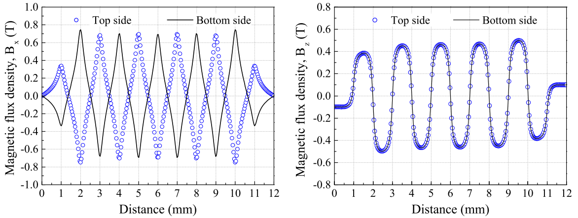
FIGURE 2.5: Magnetic flux density on both sides of the NS array at an air gap d=170 \mu\text{m}
