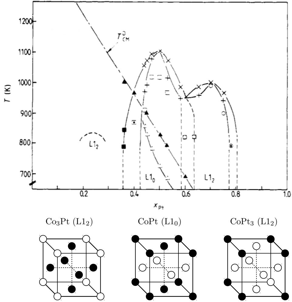
Figure 1: High-temperature magnetic and chemical phase diagram of the CoPt system [8]. Example L1_2 ( Co_3Pt , CoPt_3 ) and L1_0 ( CoPt ) structures are shown below.
