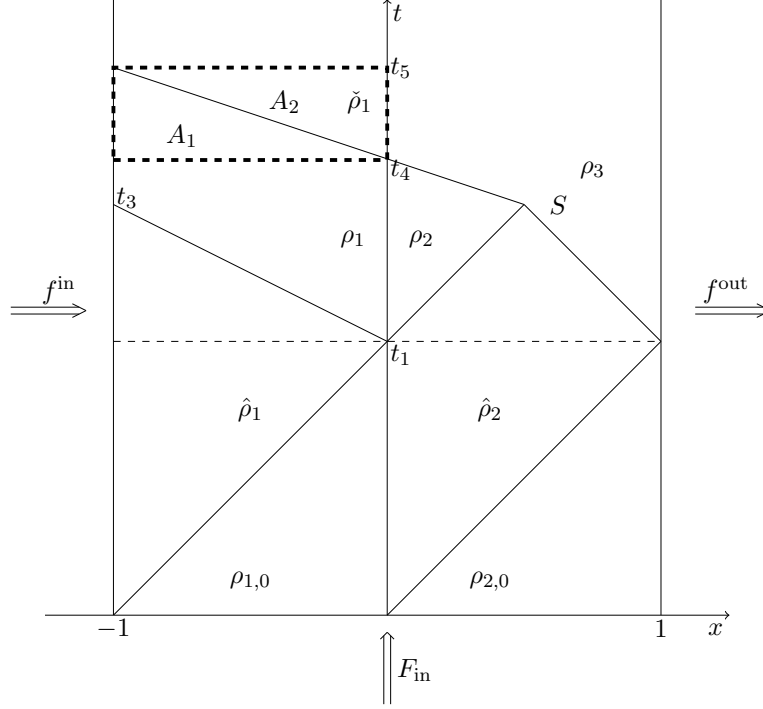
Figure 4.4.17: Area of integration in the case P < P_1 .
