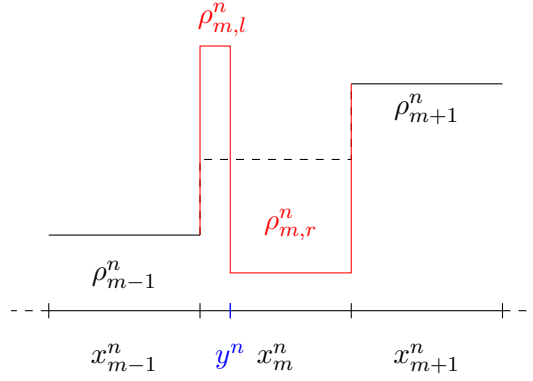
Figure 2.6.1: Reconstruction of a non-classical shock.
