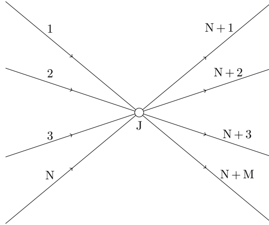
Figure 1.2.4: An example of a graph representing a road junction.
