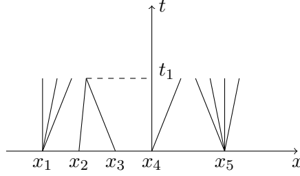
Figure 1.1.6: Construction of approximate solutions constructed by the wave front tracking up to the first time of interaction.
