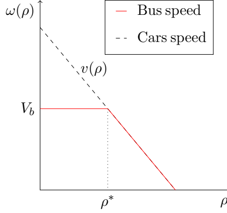
Figure 2.1.2: Bus and cars speed.
