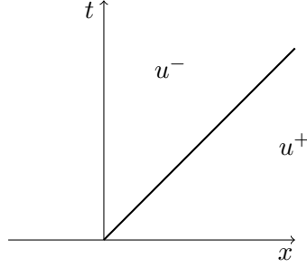
Figure 1.1.5: An example of shock wave.
