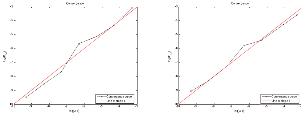
(a) Classical and non-classical shock - Case I (b) Rarefaction and non-classical shock - Case II
