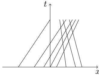
Figure 1.1.2: Intersection of characteristics.
