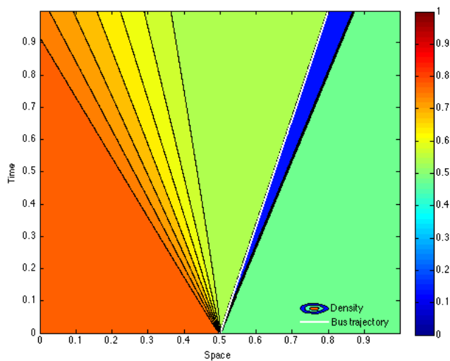
Figure 2.7.4: Density and bus trajectory in a x - t plane corresponding to initial data (2.7.3) and a mesh grid of 500 points.
