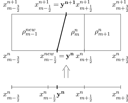
Figure 2.5.1: Local shifting of a grid point when \left| x_{m+\frac{1}{2}}^n - y^n \right| > \frac{h_m^n}{2} .
