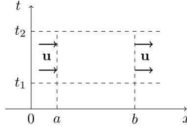
Figure 1.1.1: Flow across two points.
