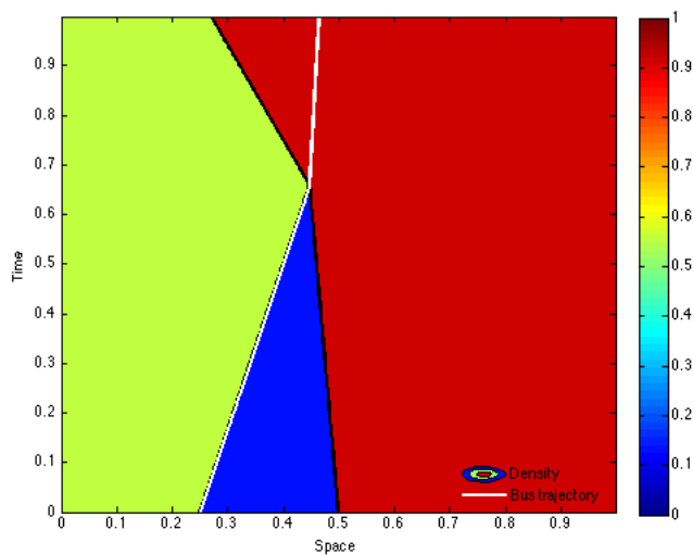
Figure 2.7.8: Density and bus trajectory in a x - t plane corresponding to initial data (2.7.5) and a mesh grid of 500 points.
