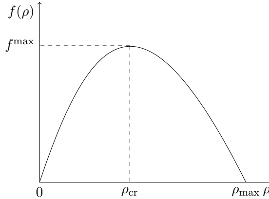
Figure 3.2.2: Flux function of equation (3.2.1).
