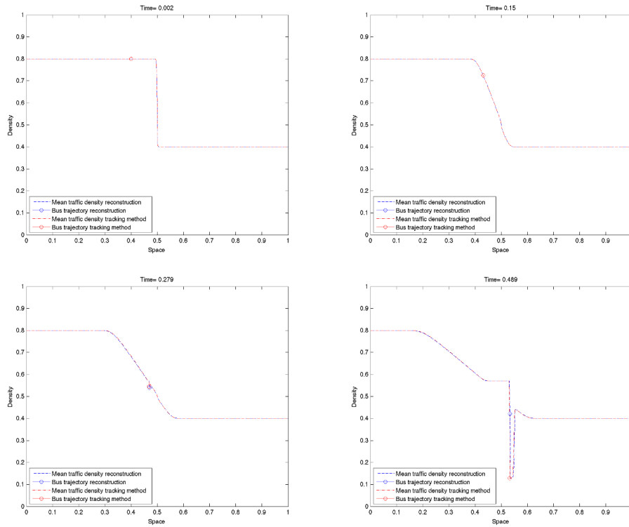
Figure 2.7.5: Evolution of the density at different times corresponding to initial data (2.7.4) and a mesh grid of 500 points.
