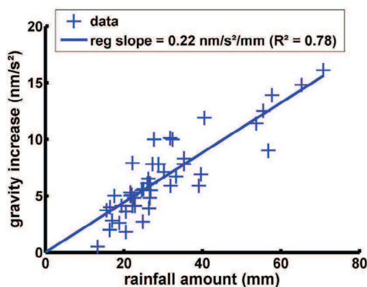
Fig. 9. Rainfall admittance.
