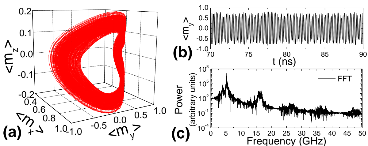
Figure 2.12: Simulation at B = 32.5 mT and J = -6 \times 10^{11} A/m 2 . (a) Mean magnetisation trajectory. (b) Time trace of \langle m_y \rangle . (c) Fourier spectrum.
