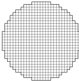
Figure 1.5: Finite difference mesh of a circular sample. The regular grid results in a rough border.
