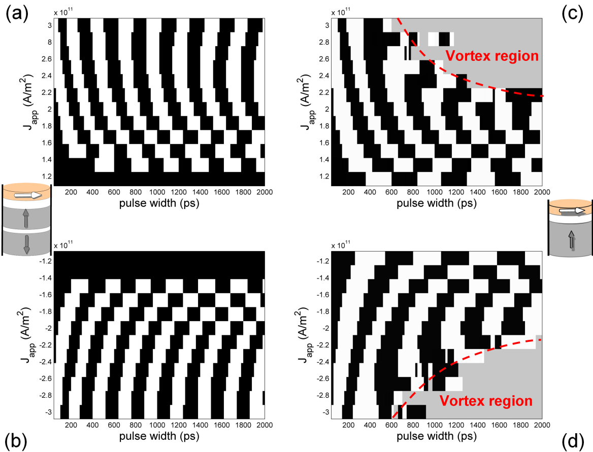
Figure 4.9: Switching diagrams obtained with FD micromagnetic simulations. Black: no switching. White: switching. Grey: the final state is a vortex. (a) J > 0 , no \text{Pol}_\perp stray field. (b) J < 0 , no \text{Pol}_\perp stray field. (c) J > 0 , stray field applied. (d) J < 0 , stray field applied.
