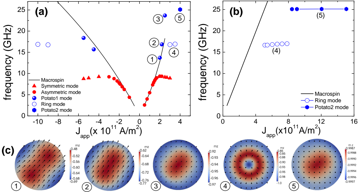
Figure 3.9: (a) Frequency versus current density of the micromagnetic simulations (symbols) and macrospin simulations (black line). Simulations performed with an angle-dependent g(\theta, \eta) function. (b) Simulations performed with a constant g(\theta) function. Only some simulations starting from out-of-plane state are presented. The obtained states correspond to the "ring mode" and "potato 2 mode". (c) Micromagnetic configurations of potato 1 mode (1,2,3), ring mode (4), and potato 2 mode (5).
