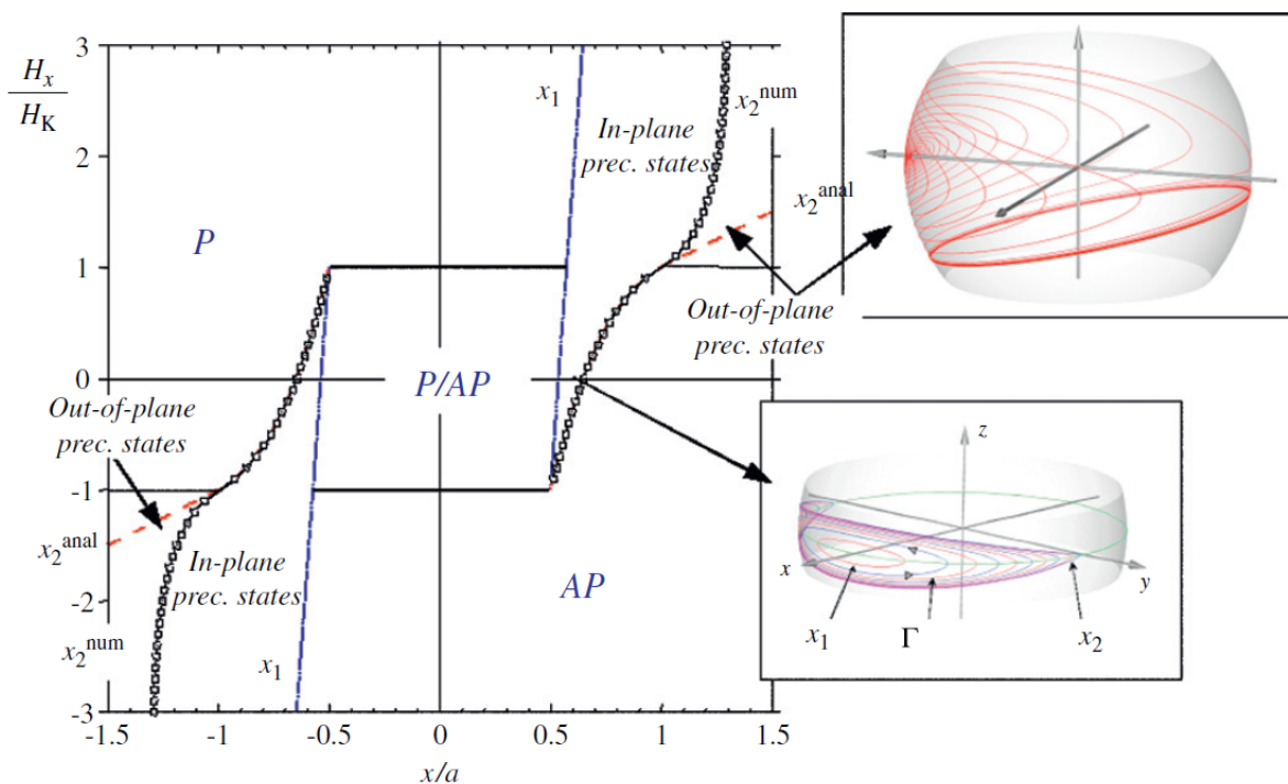
Figure 2.3: Extracted from ref [90] . State diagram of magnetisation oscillations driven by an in-plane polarised current and an in-plane field; normalised field versus normalised current. The sign convention for the current is opposite to our convention.
