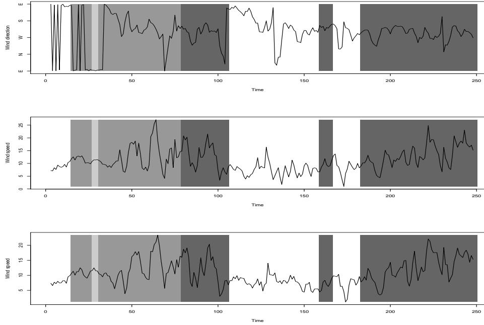
Figure 1.4: Top and central panels: wind direction and speed at a western location ( 48^{\circ}N, 10.5^{\circ}W ), bottom panel: wind speed at an eastern location ( 48^{\circ}N, 6.75^{\circ}W ). Weather regimes in grey, from the lighter to the darker: BL, AR, NAO+, NAO-.
