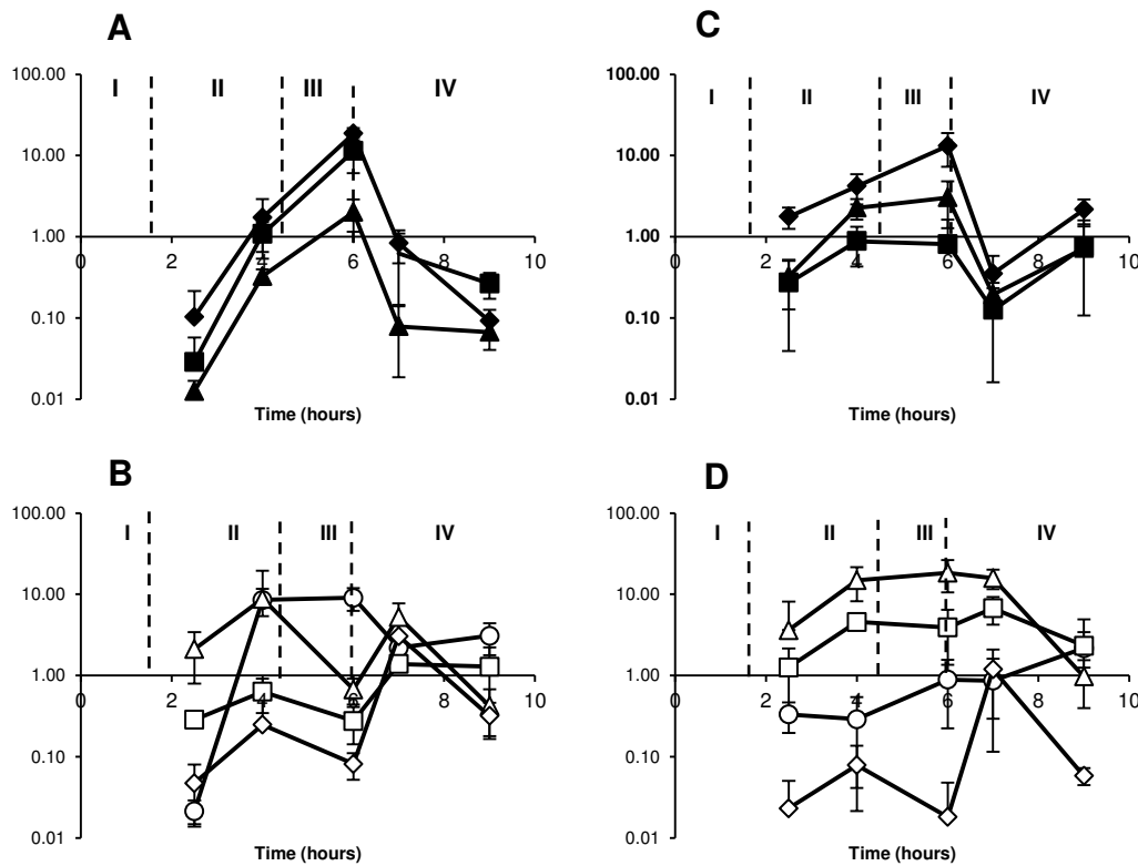
Figure 2: Kinetics of genes expression involved in sporulation initiation: spo0A (close diamond symbols), spo0B (close square symbols), spo0F (close triangle symbols), kinA (open round symbols), kinB 1 (open square symbols), KinB 2 (open triangle symbols) and kinB 3 (open diamond symbols) in aerobiosis (A and B) and anaerobiosis (C and D). S1 was used as reference (S1=1).
