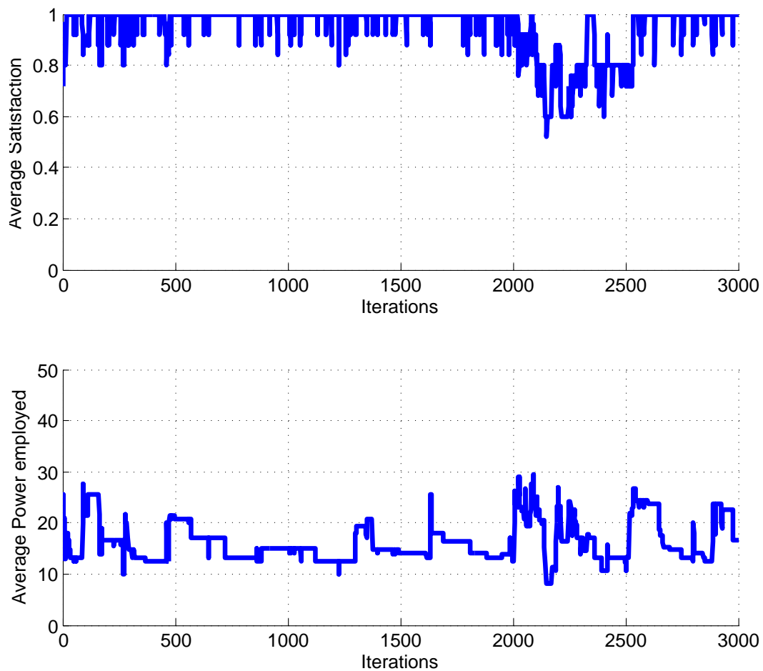
FIGURE 4.12: Achieved AS and APC as a function of the TE iterations for a the mobility scenario using the standard TE learning algorithm.
