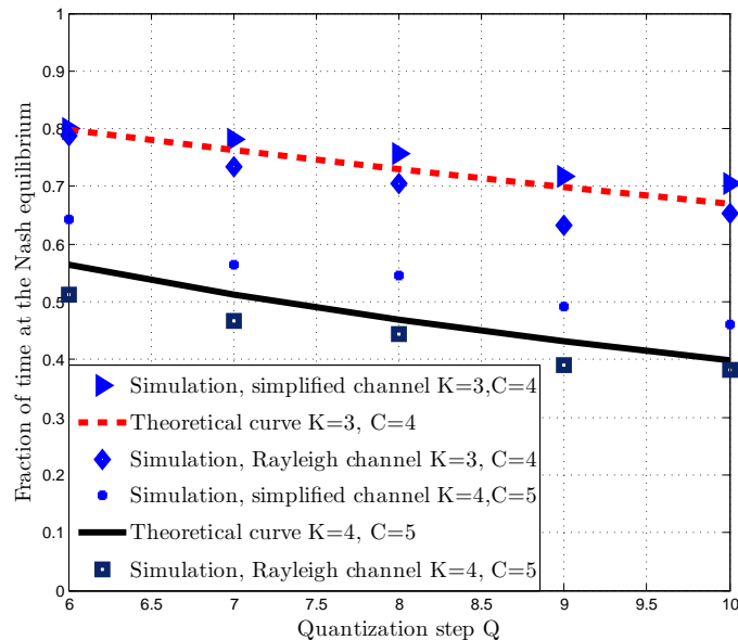
FIGURE 4.3: Fraction of time the system is at an NE, with the TE learning algorithm, \varepsilon = 0.01 and uniform probability distribution over the action set. Theoretical results are represented by the continuous lines, simulation results are represented by the markers for two sets of data and different channels: Rayleigh and the model in (4.3).
