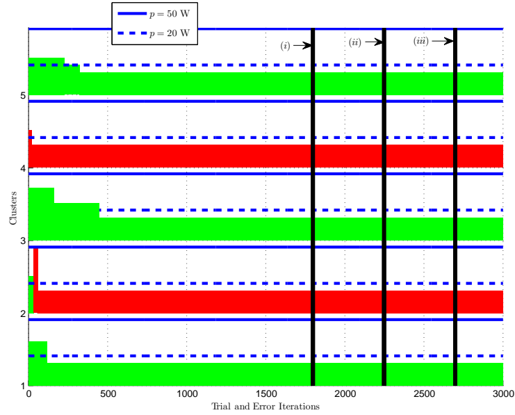
FIGURE 4.22: Progress of the channels for the ETE learning algorithm in a mobility scenario. To each color corresponds a channel, the dimension of the line represents the power level chosen for the communication. On the y -axis, the cluster in mobility is represented by the number 3.
