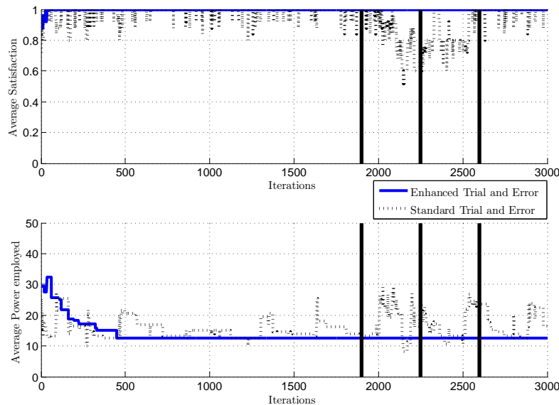
FIGURE 4.21: Achieved AS and APC for both TE and ETE. The black vertical lines indicate, approximately, the moment when the moving cluster is close enough to create interference to the others ( t = 1875 ), when it is aligned with the others ( t = 2250 ) and when it begins to be far enough ( t = 2575 ).
