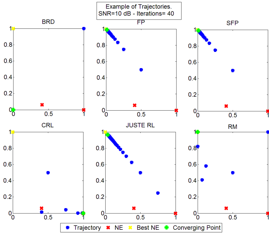
FIGURE 4.6: Example of trajectories. BRD bounces between unstable solution; FP and SFP converge close to the best NE; RL converges to a low performing NE, JUSTE-RL converges close to the best NE, RM converges close to the best NE.
