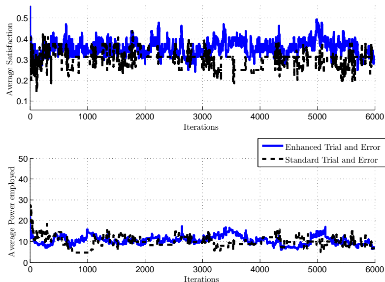
FIGURE 4.18: AS and APC in a static scenario with Rayleigh fading. The simulation parameters are the following: \Gamma = 10 dB, C = 5 , 6000 iterations. The blue continuous line represents the ETE's AS (upper plot) and APC (lower plot), while the black dashed line the TE's AS (upper plot) and APC (lower plot).
