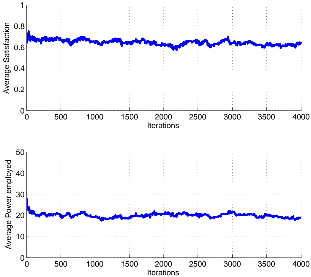
FIGURE 4.10: Achieved AS and APC as a function of the TE iterations for a square static scenario, with SINR-based feedback.
