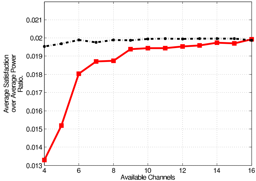
FIGURE 4.25: Performance comparison between TE and the GBDCA in terms of average number of constraints satisfied over average used power. The dashed line is the performance of TE and the continuous line the one of GBDCA .
