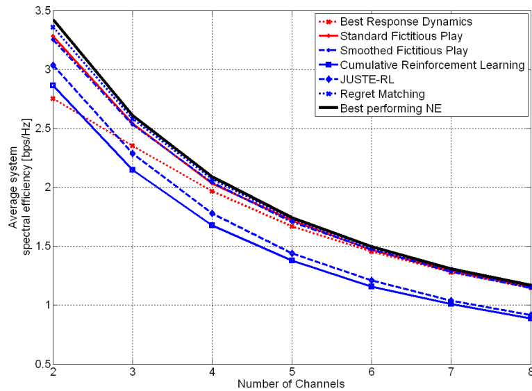
FIGURE 4.9: Average system spectral efficiency as a function of the number of channels, with SINR=10dB and 40 iterations.
