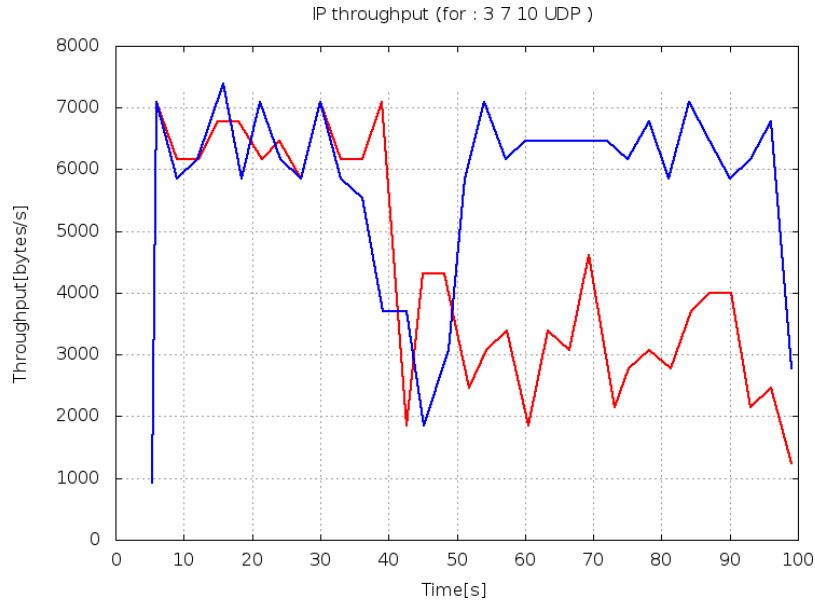
FIGURE 4.29: IP throughput at node 10 received from node 7.
