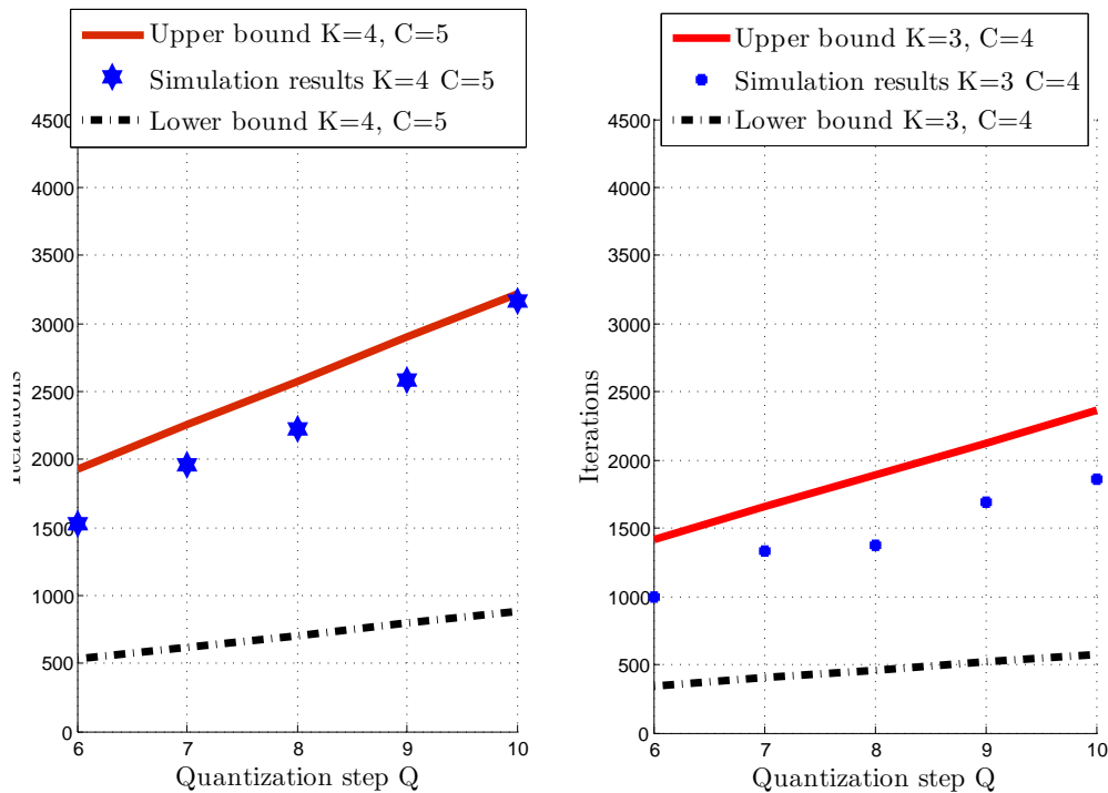
FIGURE 4.4: Number of iterations needed for the TE learning algorithm to visit an NE for the first time, with \varepsilon = 0.01 and uniform probability distribution on the actions set. The continuous lines represent (4.8), the dashed lines represent (4.9).
