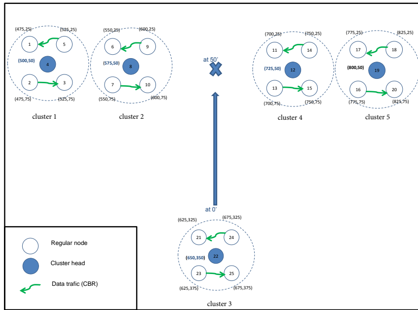
FIGURE 4.27: Scenario description used in the CORASMA simulator (distances in meter).
