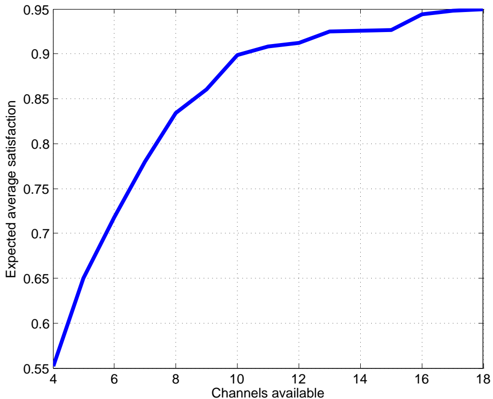
FIGURE 4.11: Expected satisfaction versus available channels. This plot has been realized assuming a square field as the one described in 3.2.
