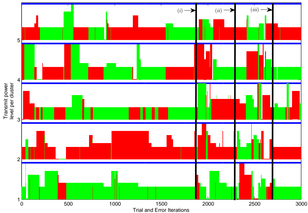
FIGURE 4.13: Channel-power allocation as a function of the TE iterations for the mobility scenario with two channels. Each color represents a different channel, and the heights of the graph the transmit power level. Clusters 1, 2, 4, 5 are static, cluster 3 is in mobility. (i) beginning of the interference from the 3rd cluster, (ii) Five clusters are aligned, (iii) end of interference from the 3rd cluster. The blue solid lines represent P_{\text{MAX}} = 50\text{W} .
