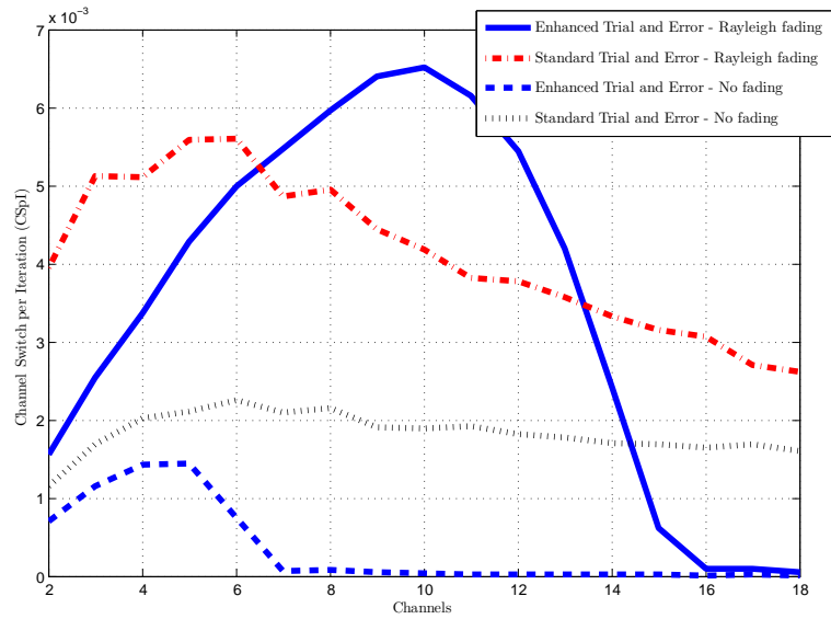
FIGURE 4.20: Channel switch per iteration as a function of the available channels for both ETE and TE learning algorithms in fading and non-fading environment.
