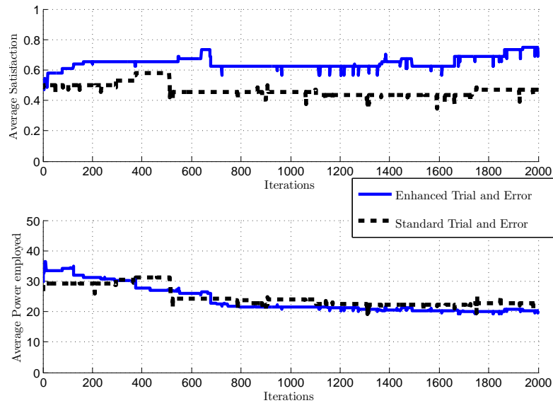
FIGURE 4.17: AS and APC in a static scenario in presence of block fading channels. The simulation parameters are the following: \Gamma = 10 dB, C = 5 , 2000 iterations. The blue continuous line represents the ETE's AS (upper plot) and APC (lower plot), while the black dashed line the TE's AS (upper plot) and APC (lower plot).
