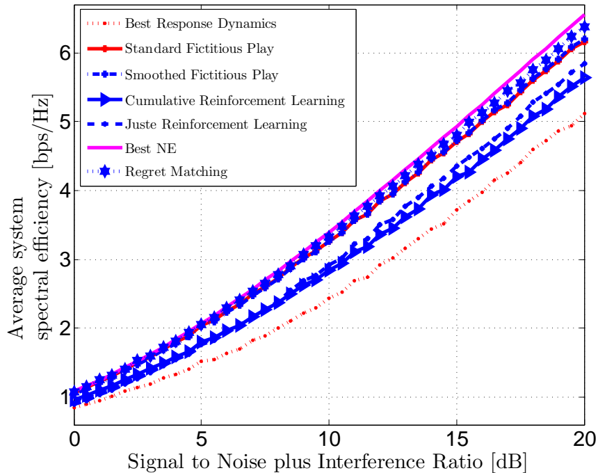
FIGURE 4.5: Average system spectral efficiency [bps/Hz] as a function of SINR with 40 iterations for the 2 players and 2 channel case.
