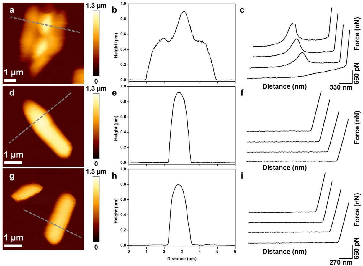
Figure 1. Imaging of K. pneumoniae ATCC 700603 cells. (a) Height image of K. pneumoniae ATCC 700603 cells under native conditions, (d) treated with colistin at 0.5\times MIC (0.25 mg/L) or (g) treated with colistin at 0.75\times MIC (0.375 mg/L). (b, e and h) cross-sections recorded along the dashed lines respectively on a, d and g. (c, f and i) representative extend force curves recorded on small areas on top of cells presented respectively in a, d and g. In each condition, force curves were recorded on 5 cells coming from 3 independent cultures (total of 5120 force curves per condition).
