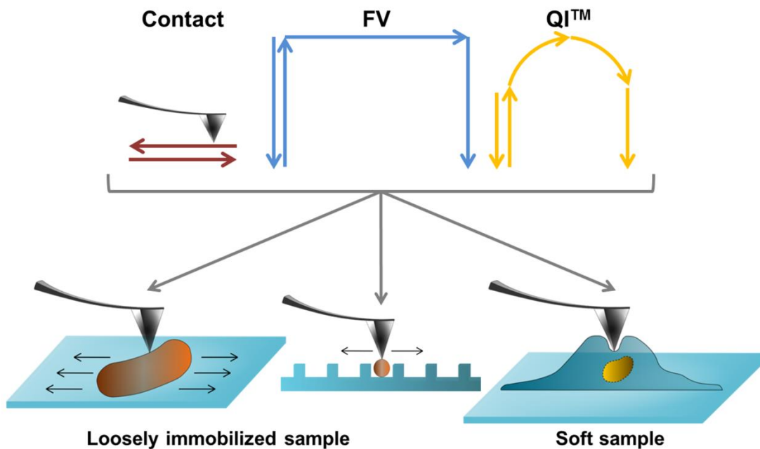
Figure 8. AFM modes comparison. For each mode, contact, Force-Volume (FV) and Quantitative Imaging TM (QI TM ) mode, the movement of the AFM tip is represented. These modes were applied to different kinds of samples: loosely immobilized samples and soft samples. QI TM is the best suited for these kind of samples. Reprinted from 66 .
