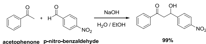
Scheme 4. Aldolization of p -nitro-benzaldehyde with acetophenone.
