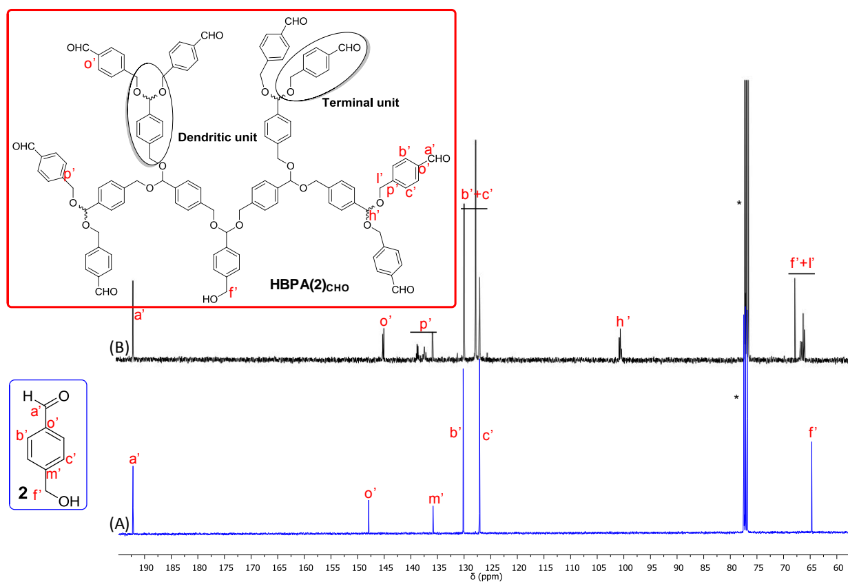
Figure 15. ^{13}\text{C} NMR spectrum (100 MHz; \text{CDCl}_3 ) of (B) hyperbranched polyacetal \text{HBPA}(2)_{\text{CHO}} (entry 4 in Table 1) and (A) monomer 2 (*).
