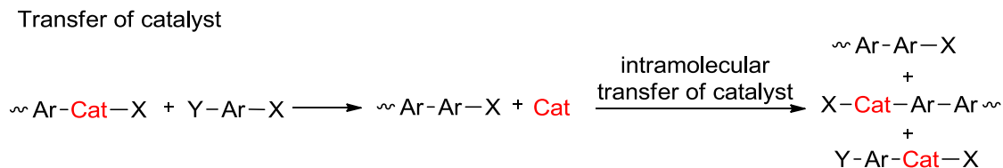
Scheme 6.9 Chain-growth polymerization by transferring catalyst intramolecularly.
