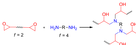
Scheme 4.13 Epoxy resin curing from a diepoxide ( f = 2 ) and a diamine ( f = 4 ).
