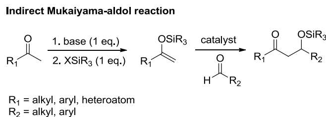
Scheme 5. Indirect Mukaiyama aldolization.
