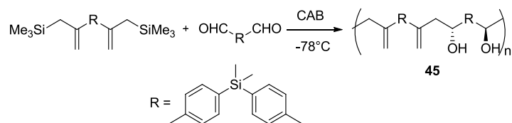
Scheme 5.19 Polymer 45 synthesized via asymmetric Hosomi-Sakurai allylation in presence of catalyst CAB at -78^\circ\text{C} .
