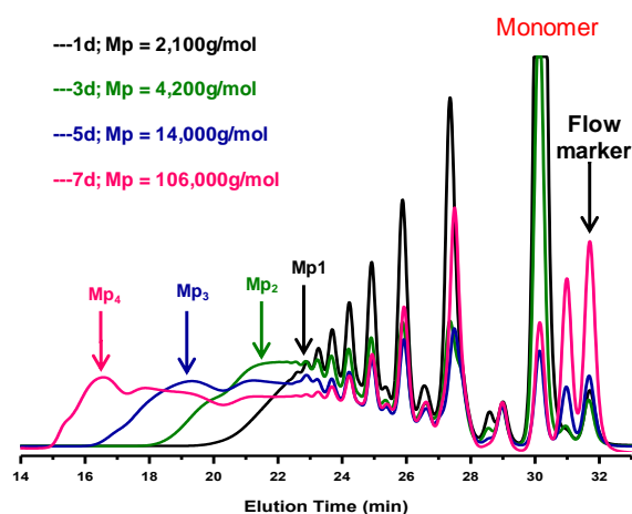
Figure 12. SEC traces (UV detection in THF; relative to PS standards) of hyperbranched polyacetals HBPA(2) CHO obtained from monomer 2 at different intervals (entry 5, Table 1).
