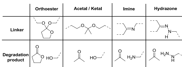
Figure 1. Examples of acid-degradable bonds and their degradation products.
