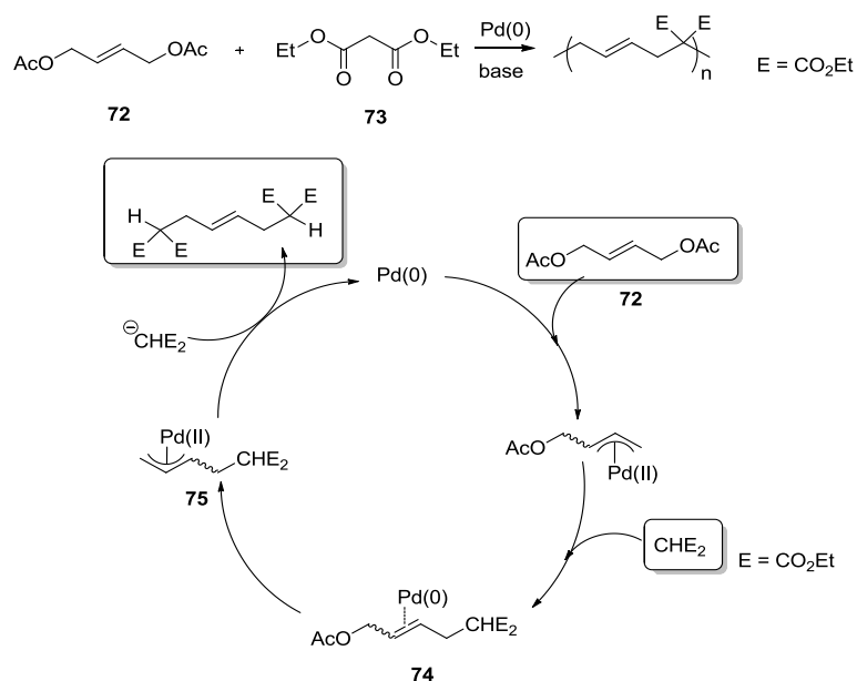
Scheme 6.4 Nonstoichiometric polymerization of 1,4-diacetoxybut-2-ene ( 72 ) and diethyl malonate ( 73 ) catalyzed by palladium in presence of base.
