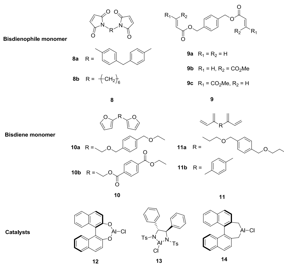
Scheme 5.11 Monomers and catalysts investigated in asymmetric Diels-Alder polymerization.
