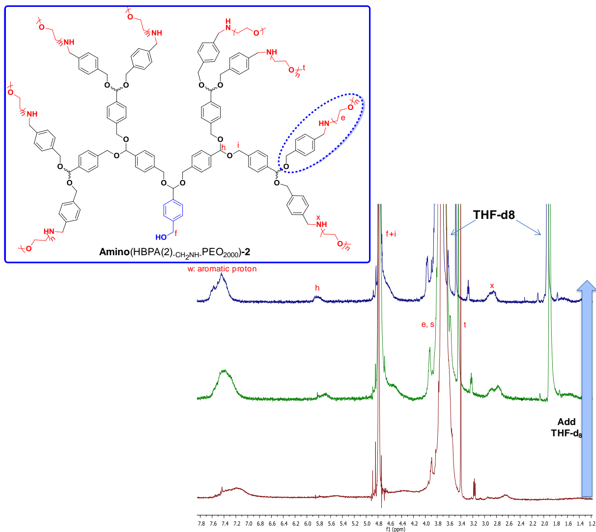
Figure 29. 1 H NMR spectra of hyperbranched polyacetal-PEO 2000 Amino(HBPA(2)-CH 2 NH-PEO 2000 )-2 (400 MHz) in D 2 O with increased amounts of THF-d 8 .
