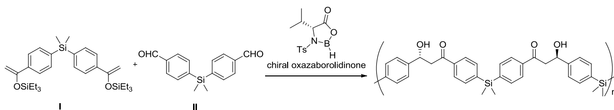
Scheme 15. Asymmetric Mukaiyama aldol polyaddition of dialdehyde II and bis(silyl enol ether)
