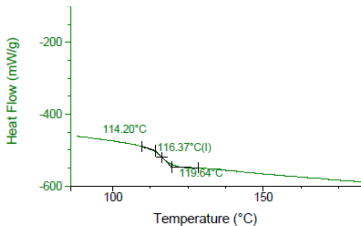
Figure 26. DSC thermograms of polybenzoin PBz-3 at a heating rate of 10 °C min -1
