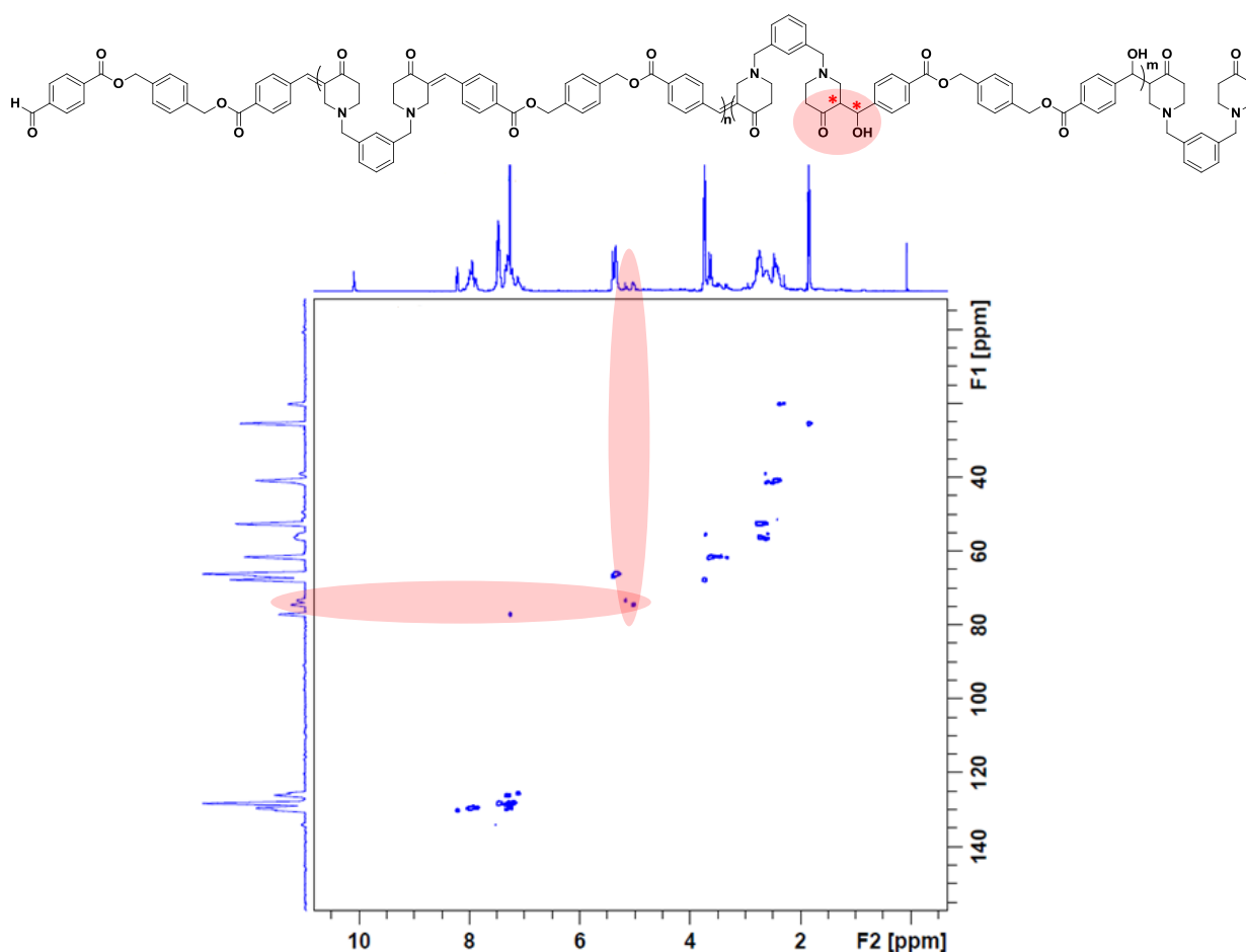
Figure 9. 2D NMR spectrum ( \text{CDCl}_3 ) of polyaldol obtained from the polymerization of bis-piperidinone 5 and bis-aldehyde 9 (entry 6, Table 1).
