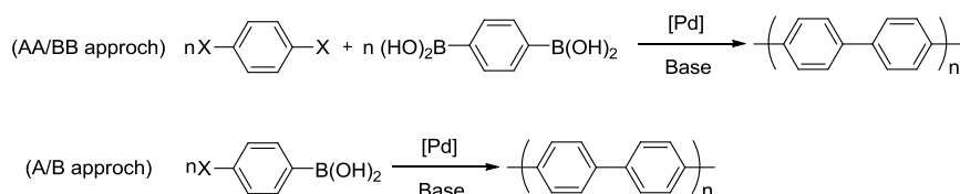
Scheme 5.35 PPP synthesized from Suzuki-Miyaura polymerization.
