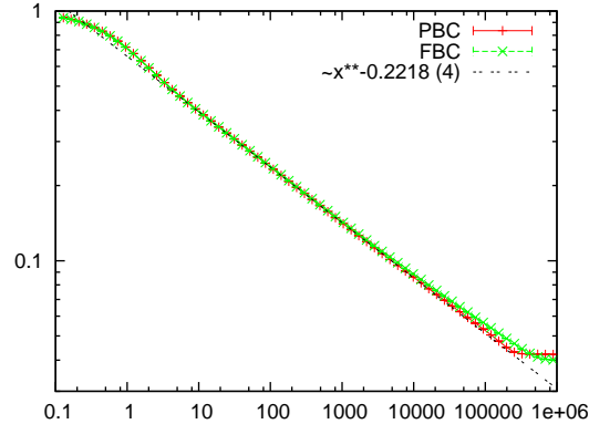
Figure 2.21 – The persistence \mathcal{P}(t, L = 1024) vs. t for the ferromagnetic 2dIM on the square lattice with PBC and FBC (red and green data, respectively, see the key) quenched at t = 0 from a 1/T \rightarrow 0 initial state to T = 0 . The dotted (grey) line corresponds to the best fit found over the interval t \in [100 : 10000] with a power law for the PBC case.
