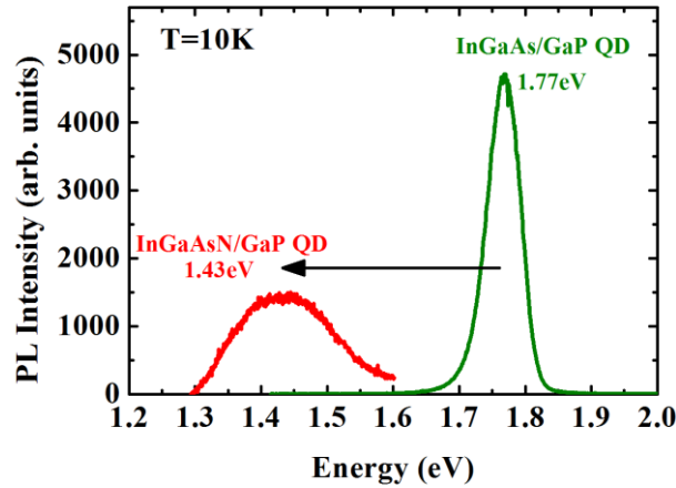
Fig. 4-42: Low temperature PL spectrum of InGaAs/GaP QD (green line) and InGaAsN/GaP QD (red line).
