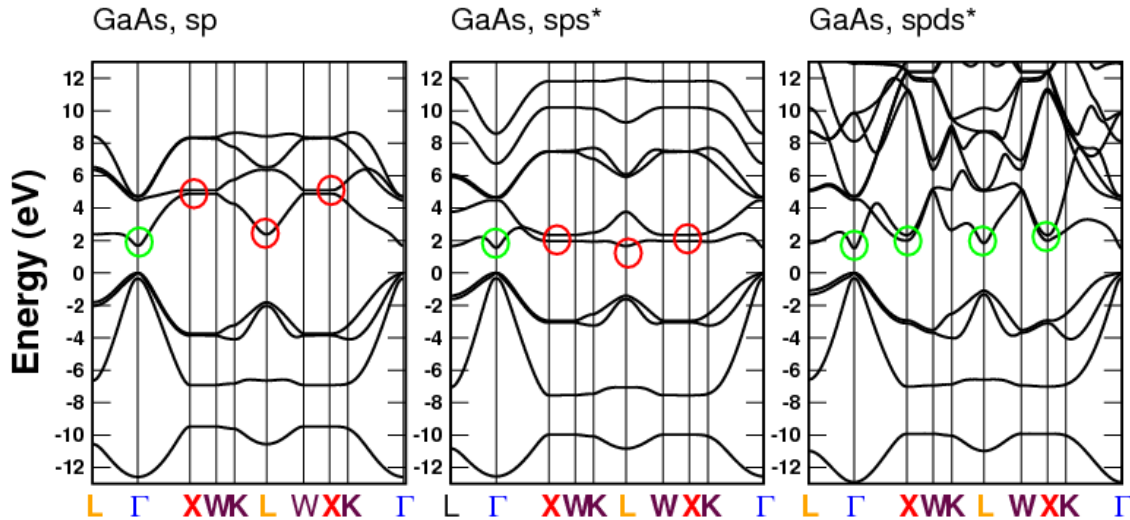
Fig. 2-10: Comparison of GaAs TB band structures obtained for various basis sizes: (a) sp^3 , (b) sp^3s^* , (c) sp^3d^5s^* . Green and red circles indicate the correct and incorrect energy-band dispersion.
