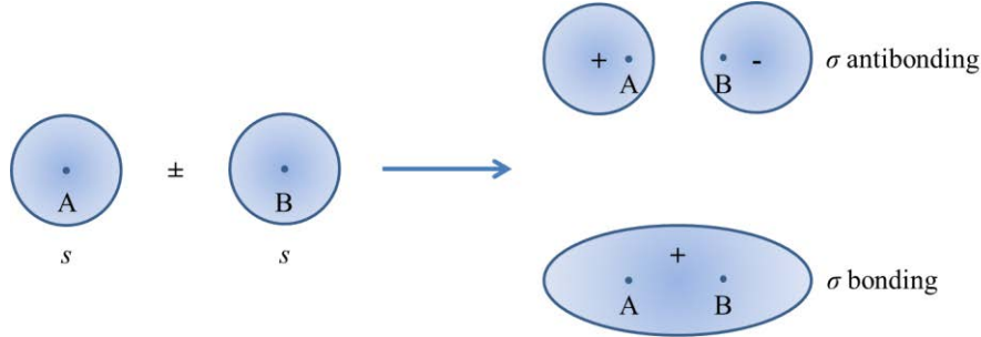
Fig. 2-9: Overlap of two s atomic orbitals to form \sigma molecular orbitals.
