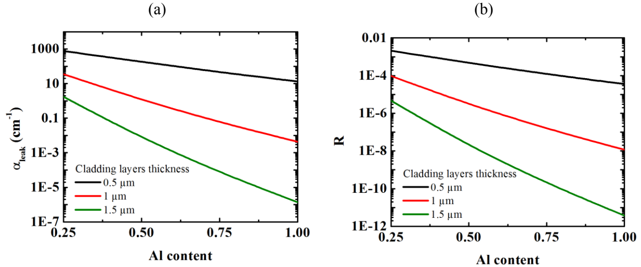
Fig. 3-45: (a) Leakage of the optical mode in the substrate and (b) ratio between the intensity of the optical mode at the interface AlGaP/air and the maximum of intensity as a function of Al content and cladding layers thickness.
