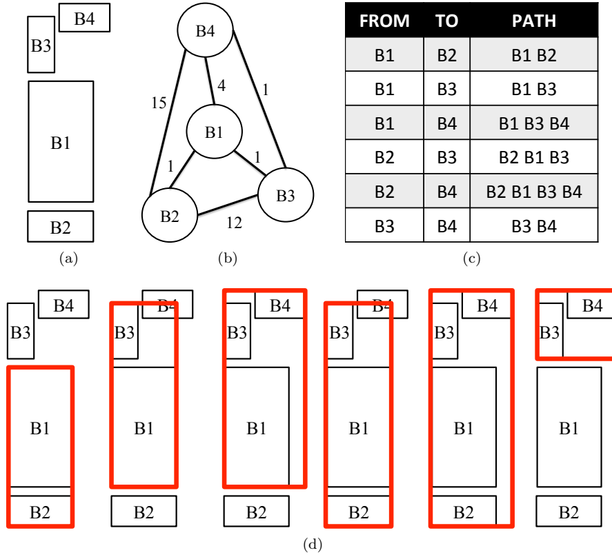
Figure 3.19 An example of the algorithm in charge of creating derived blobs (objects) for a split pattern: starting from the detected blobs in (a), the algorithm creates the graph in (b) and finds the shortest paths in (c). The output of the algorithm is in (d).
