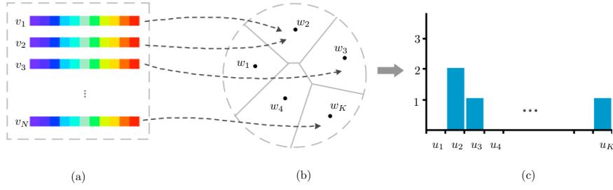
Figure 4.2 Second-level feature vectors construction. The interval to be classified is segmented into N frames of 32 milliseconds that are represented as first-level feature vectors (a). For each vector v_i the codebook is searched for the nearest aural word w_j (b). Then a histogram of the occurrences of the aural words is computed (c). In the example, the vectors v_1 and v_2 have w_2 as the nearest aural word in the codebook. Thus, the second bin of the histogram has a value equal to 2. In the same way, aural word w_3 has only one close vector, resulting in a value equal to 1 for the third bin of the histogram. Aural words w_1 and w_4 , instead, have no occurrences.
