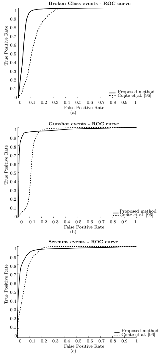
Figure 5.35 Comparison of the performance of the proposed method with respect to the method of Conte et al. [96] in terms of ROC curves for the broken glass (a), gunshot (b) and scream (c) events. Note that the proposed method (solid line) clearly outperforms [96] (dashed line).
