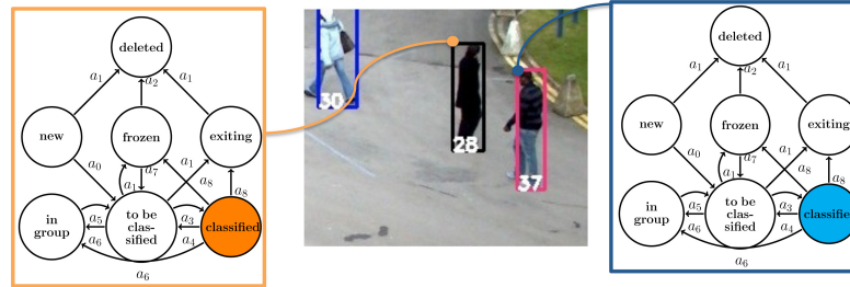
Figure 3.12 Evolution of the states of the FSA of each object along a short frame sequence (part 1). The second part is in Figure 3.13.
