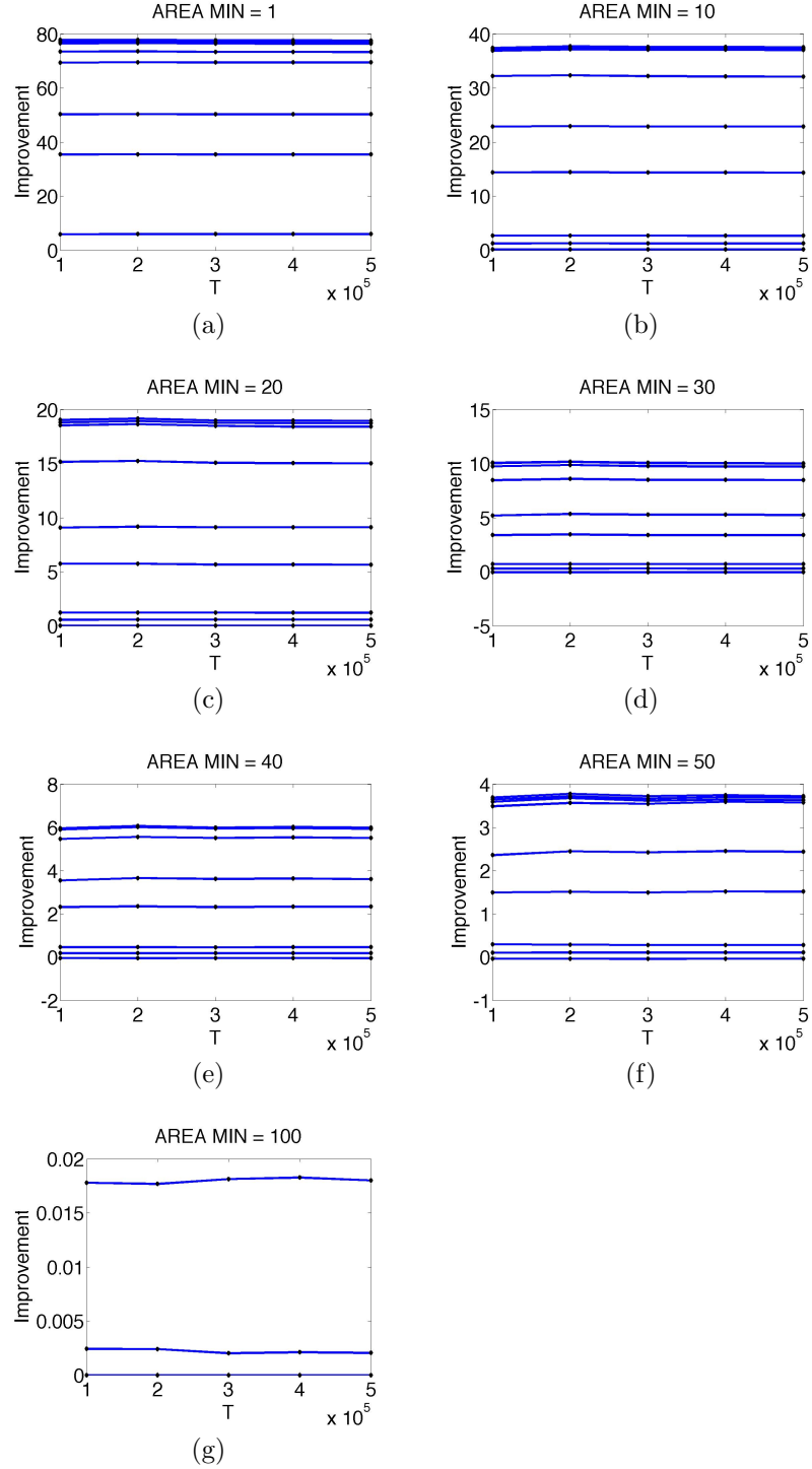
Figure 5.29 Improvement of the proposed method if compared with the available Postgis solution by varying the segmentation conditions (Area Min) and the query cube dimension D_c .
