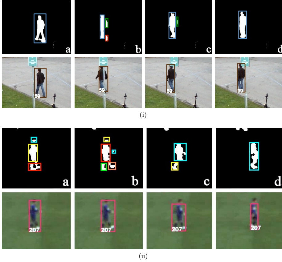
Figure 5.11 The output of the proposed method on two sequences from the PETS (i) and the ISSIA Soccer (ii) datasets, both containing a split; the first and the second row respectively represent the input and the output of the method.
