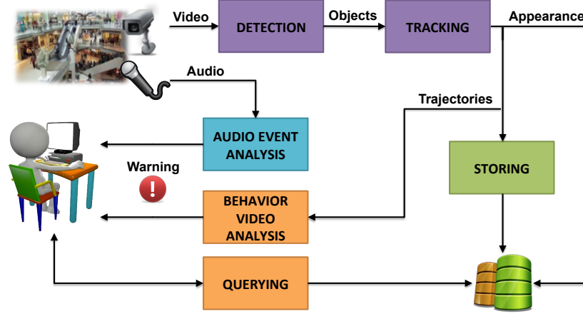
Figure 1.2 Architecture of the proposed system.
