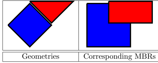
Figure 3.32 The geometries do not intersect, while the corresponding MBRs do it.
