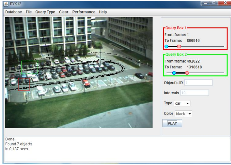
Figure 5.25 A snapshot of the GUI.
