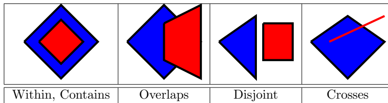
Figure 3.31 Some of the basic spatial operations allowed by spatial databases.
