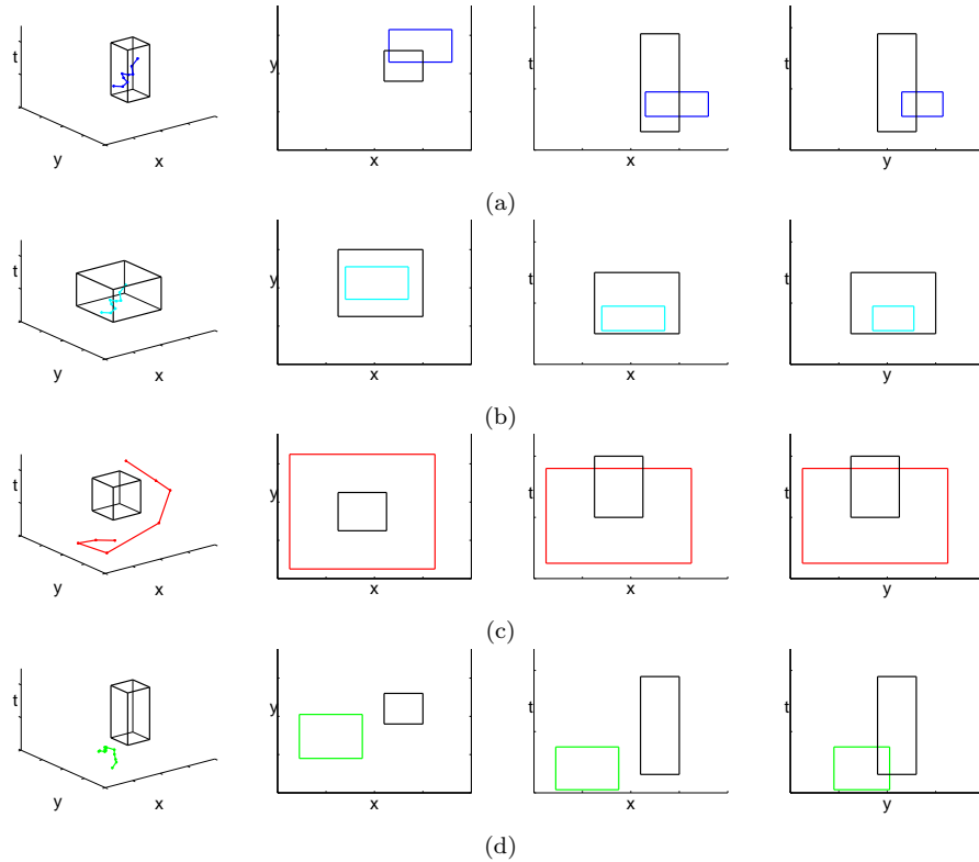
Figure 3.35 Each row shows a trajectory and a query box, together with the corresponding projections on the 2D planes. In (a) the trajectory intersect the query box; in (b) it is completely contained in the query box; in (c) the trajectories does not intersect the query box although all the 2D projections do it; in (d) the trajectory does not intersect the query box.
