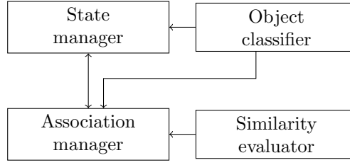
Figure 3.4 An overview of the proposed tracking system.
