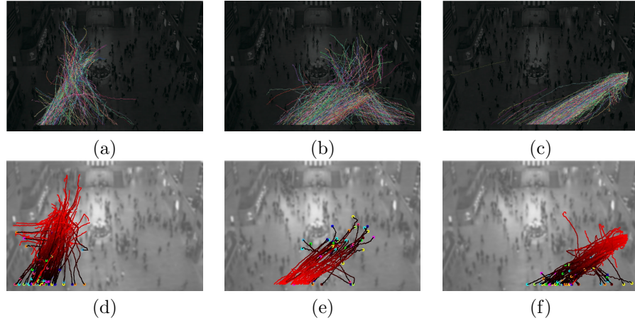
Figure 5.20 MIT2: in first row the clusters belong to the following methods: (a) Spectral Clustering [140], (b) HDP [141] and MDA mode [135]. These figures have been provided by the authors of [135]. In second row (d,e,f) the corresponding clusters obtained by the proposed method are depicted.
