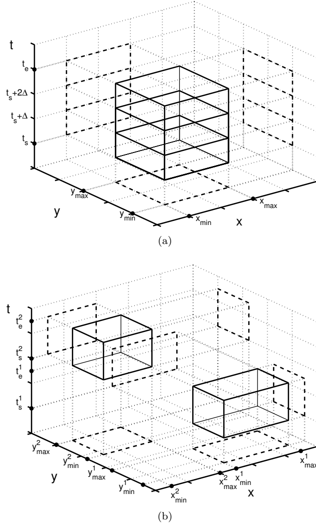
Figure 3.44 Geometric interpretation of a Flow-DRSQ (a), and of a 2-DRSQ (b).
