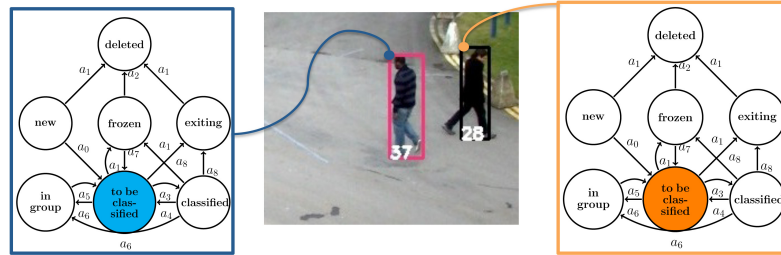
Figure 3.13 Evolution of the states of the FSA of each object along a short frame sequence (part 2). The first part is in Figure 3.12.
