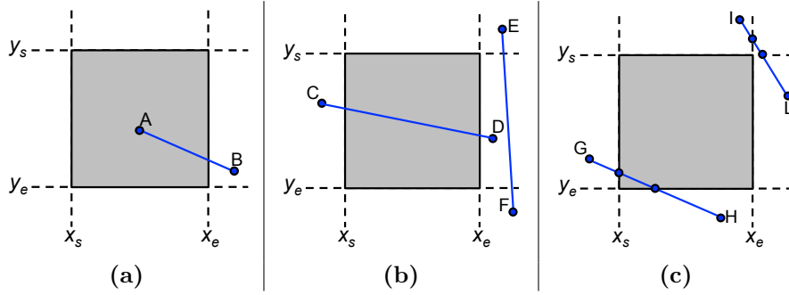
Figure 3.34 The Cohen Sutherland clipping algorithm at work: in (a) and (b) the segment can be trivially analyzed, while in (c) a further processing is needed.
