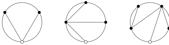
Figure 1.4: Examples of dissection diagrams of respective degrees 2, 3, 4. The polygons are drawn as circles. Every polygon has a distinguished vertex, which is called the root and is depicted as a white dot.
