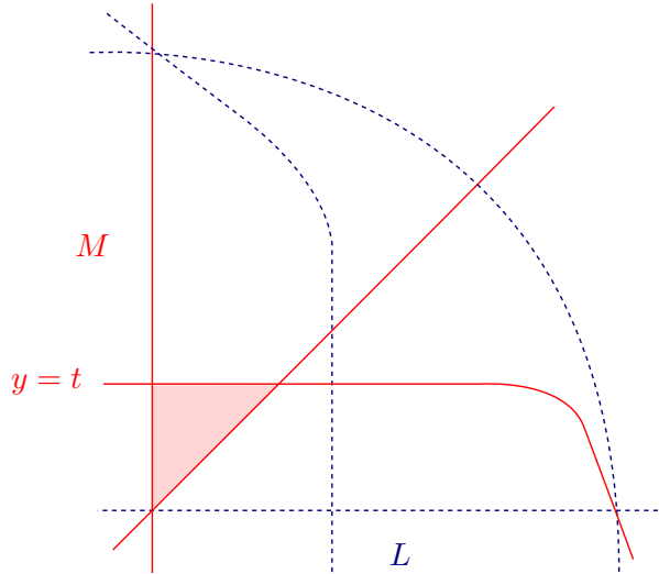
Figure 1.2: The example of \text{Li}_2(t)
