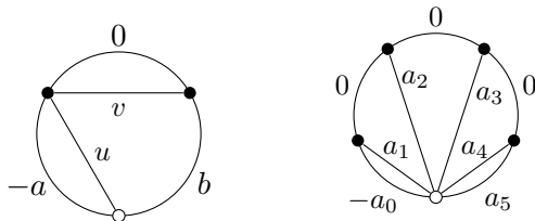
Figure 1.5: Decorated dissection diagrams. On the right, a decorated corolla.
