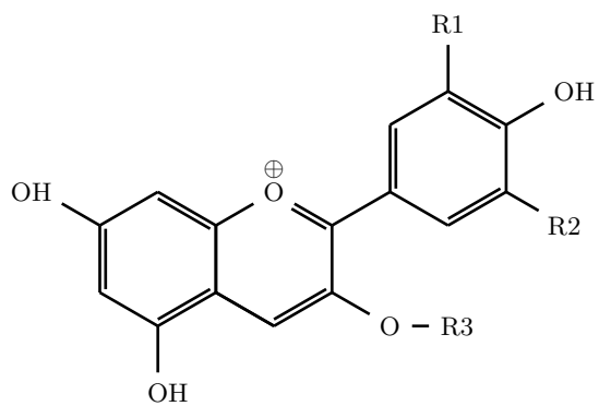
Figure 10. Anthocyane
