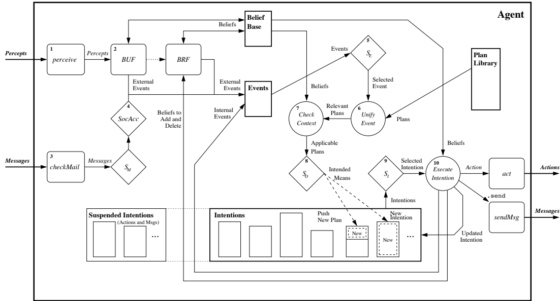
Figure 8.1 – The execution cycle of the AgentSpeak Architecture
