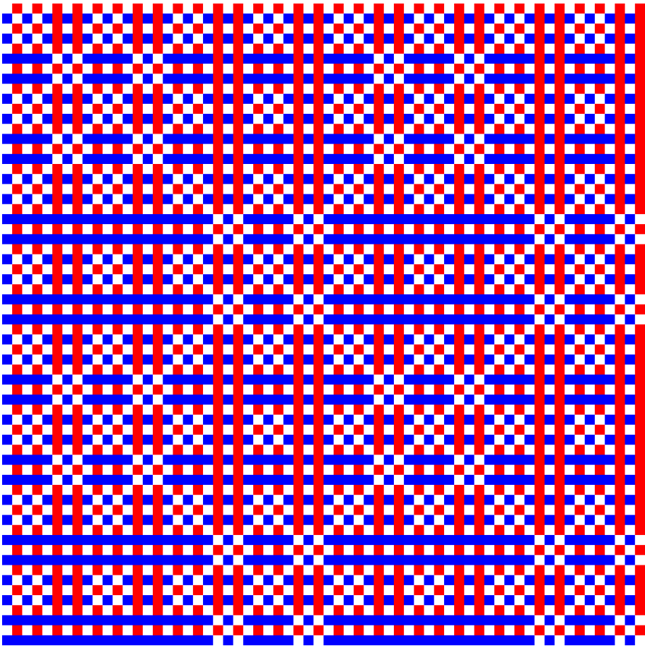
Fig. 9: Detail of \mathcal{A}_8
