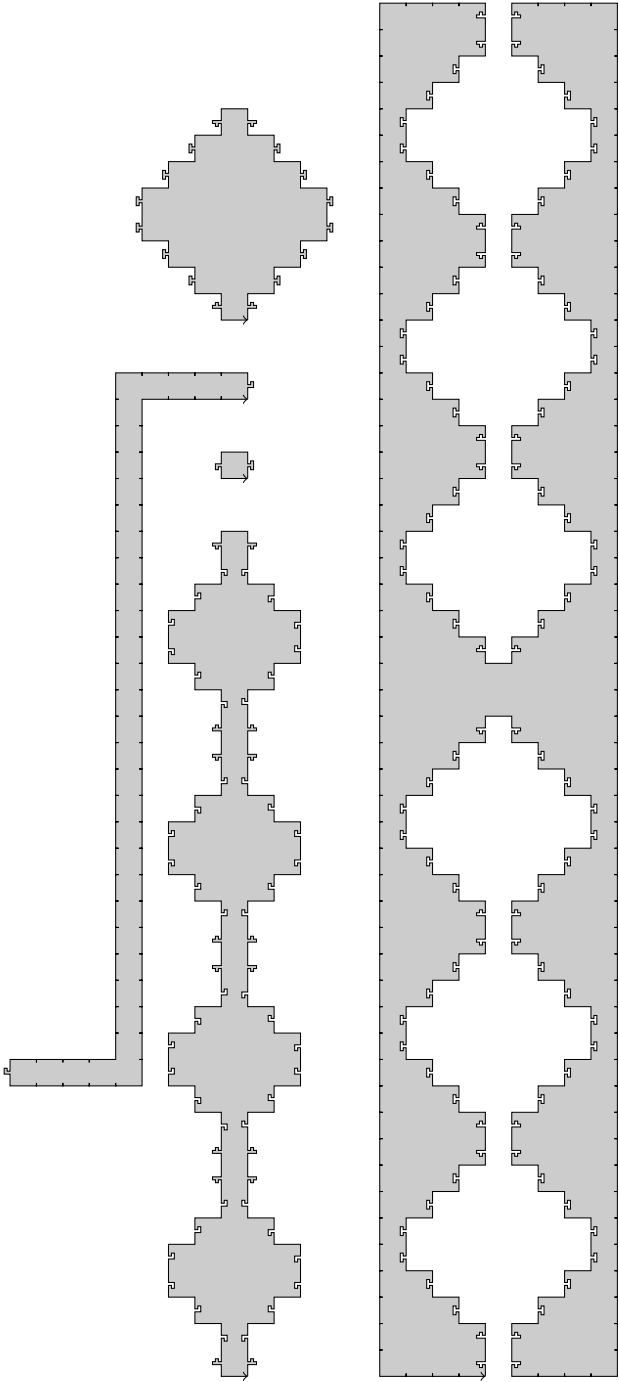
Fig. 3: Tiles (rotated to fit in page) From left to right and bottom to top : meat , tooth , wire , filler , jaw Notice that here N = 4 and k = 3 to fit the page (in the text k > 4 ).
