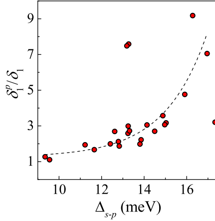
Figure 6.4: The ratio \delta_1^P/\delta_1 as a function of the energy separation \Delta E_{s-p} . Dashed line is a guide to the eye.
