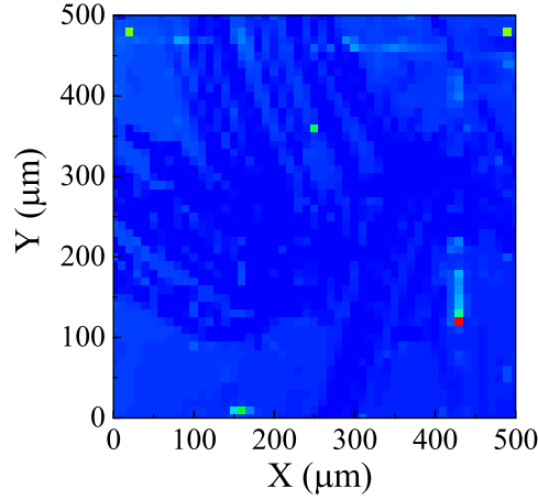
Figure 3.5: The micro-PL map of the emission from the QDs in the energy range: 1.58-1.70 eV. The mapping step was the same in both direction and equal 10 \mu\text{m} . The map was measured using the setup presented on part (b) in Fig. 4.1.
