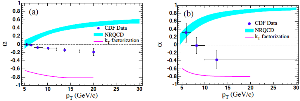
Figure 1.5. p_T dependence of the prompt polarizations in p\bar{p} collisions at \sqrt{s}=1.96 TeV for (a) J/\psi and (b) \psi(2S) . The band correspond to the LO NRQCD prediction [33], while the line represent the k_T factorization model [32]. From [34].
