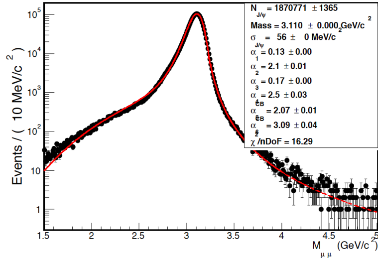
Figure 6.2. Fit to the J/\psi MC invariant mass spectra with the NA60 function.
