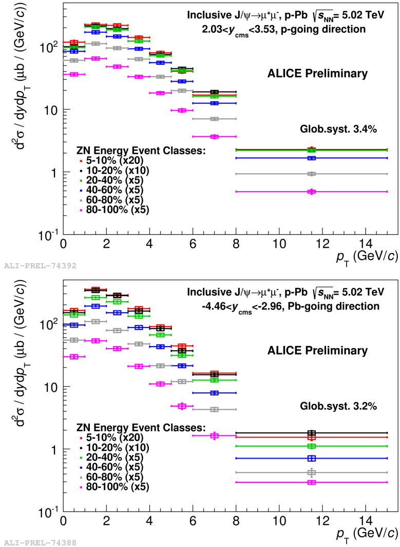
Figure 8.8. d^2\sigma_{\text{pPb}}^{J/\psi}/dydp_T as a function of p_T for different ZN event activity classes in p-Pb (top) and Pb-p (bottom). From [228].
