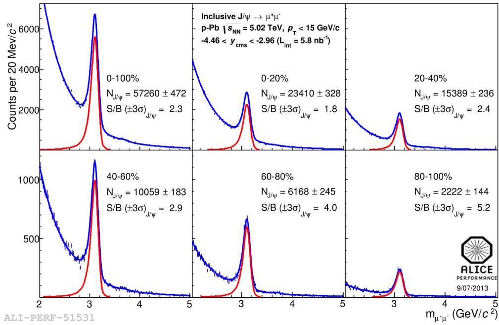
Figure A.6. Examples of the signal extraction in Pb-p with Pol2×Exp + NA60CB2 fit in different V0A event activity classes, integrated over p_T and y .
