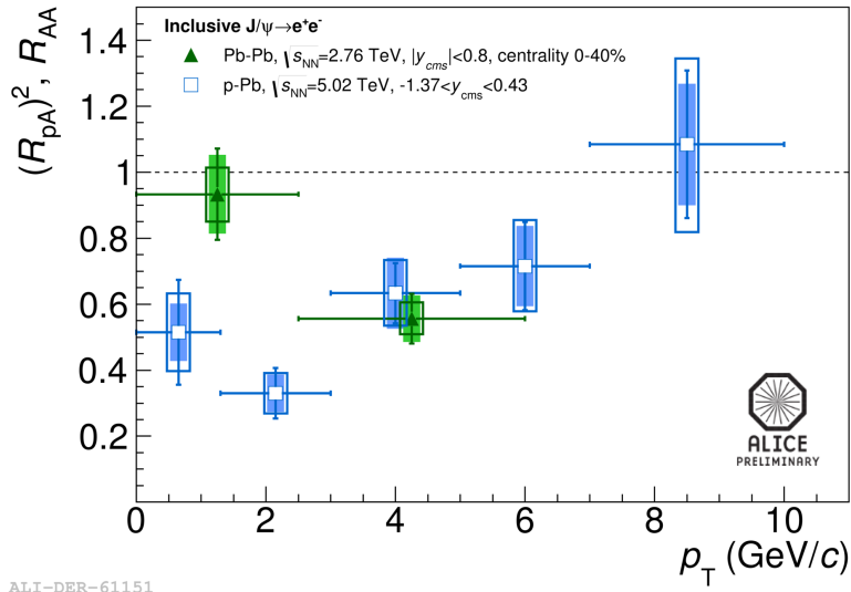
Figure 8.26. R_{\text{Pb-Pb}} and \left(R_{\text{pPb}}^{\text{midy}}\right)^2 vs p_T . The bars correspond to statistical uncertainties, shaded areas represent the partially correlated and the open boxes stand for the uncorrelated systematic uncertainties. From [226].
