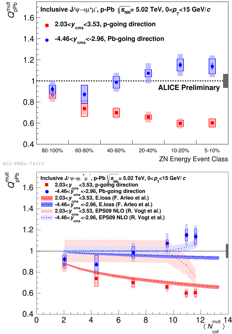
Figure 8.15. Q_{pPb}^{\text{mult}} for the J/\psi as a function of the ZN event activity (top, from [228]) and of the \langle N_{\text{coll}}^{\text{mult}} \rangle (bottom) for forward (red) and backward (blue) rapidity. Vertical errors represent the statistical uncertainties, shaded boxes around the points the partially correlated uncertainties and open boxes around the points the uncorrelated uncertainties. Grey box at unity is the global uncertainty. The theoretical predictions in the right panel are from the private communications with the authors of the papers on EPS09 LO [229] (striped bands) and coherent parton energy loss model [225] (shaded bands). The dashed lines in the theoretical bands correspond to the central values, the bands are the corresponding uncertainties.
