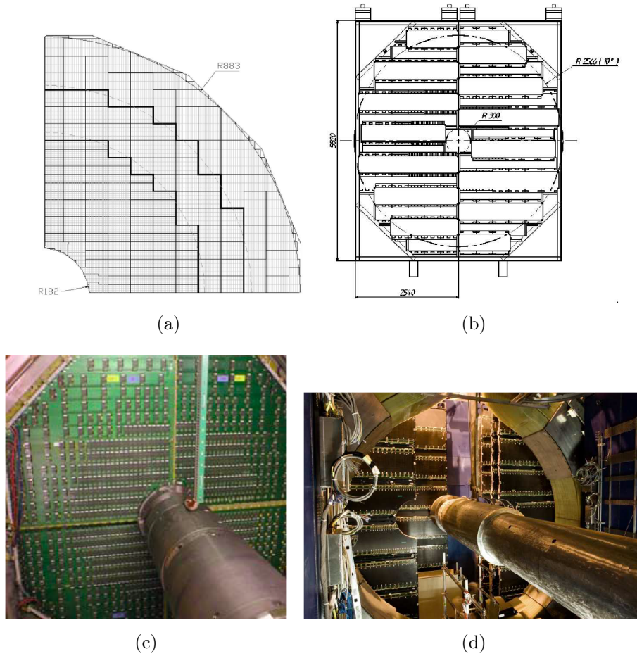
Figure 4.8. (a): The cathode plane layout of Station 1. From [50]. (b): Segmentation of a station with a slat architecture. From [60]. (c): A photograph of TRK2. From [175]. (d): An overview of a station with a slat architecture. From [50].
