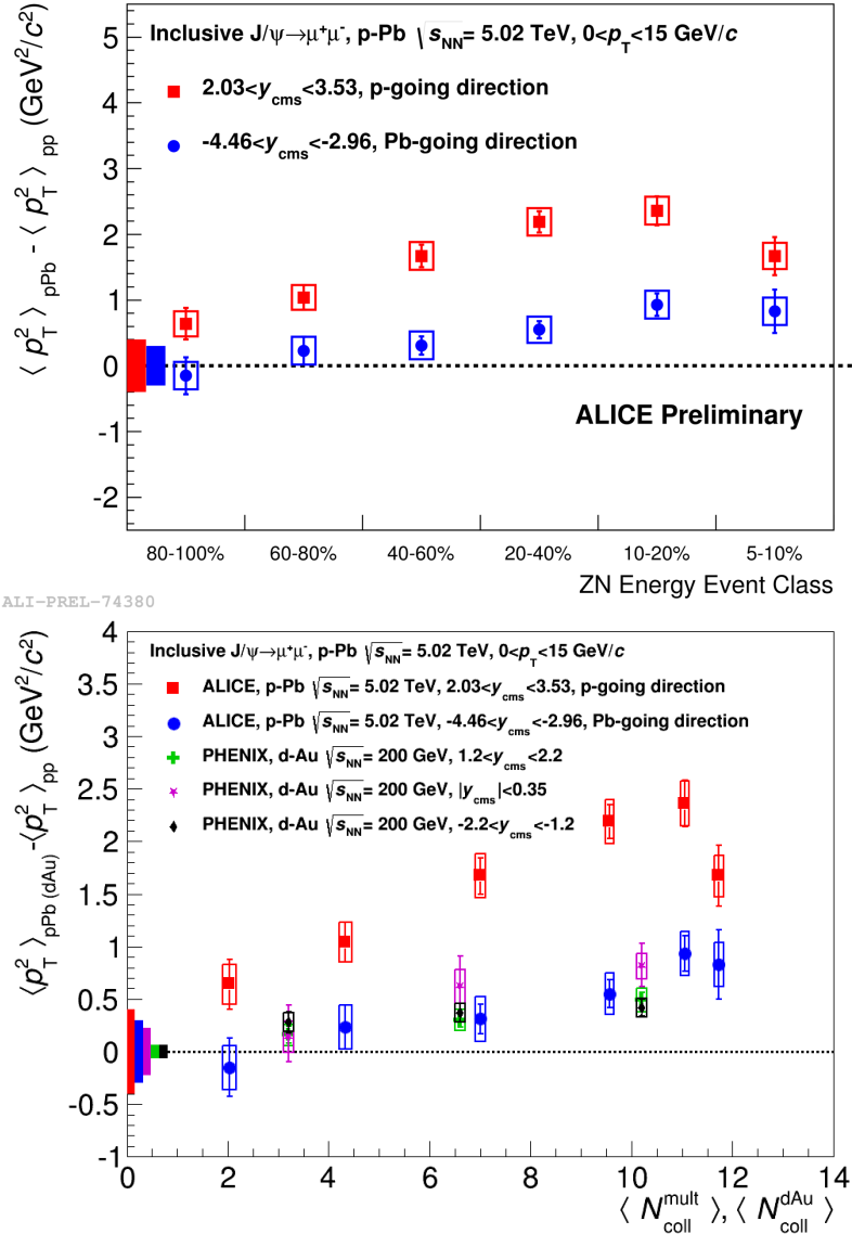
Figure 8.13. Top: The ZN event activity dependence of \Delta \langle p_T^2 \rangle_{\text{pPb}}^{J/\psi} . Bottom: \Delta \langle p_T^2 \rangle_{\text{pPb}}^{J/\psi} ALICE results as a function of N_{\text{coll}}^{\text{mult}} at \sqrt{s_{\text{NN}}} = 5.02 TeV compared to the \Delta \langle p_T^2 \rangle_{\text{dAu}}^{J/\psi} PHENIX results [139] vs N_{\text{coll}} for d-Au collisions at \sqrt{s_{\text{NN}}} = 200 GeV. Data points are shown in colors: red (ALICE, forward y ), blue (ALICE, backward y ), green (PHENIX, forward y ), purple (ALICE, mid- y ), black (PHENIX, backward y ). The color boxes around zero represent the uncertainties of \langle p_T^2 \rangle_{\text{pp}}^{J/\psi} for the results with the same color. From [228].
