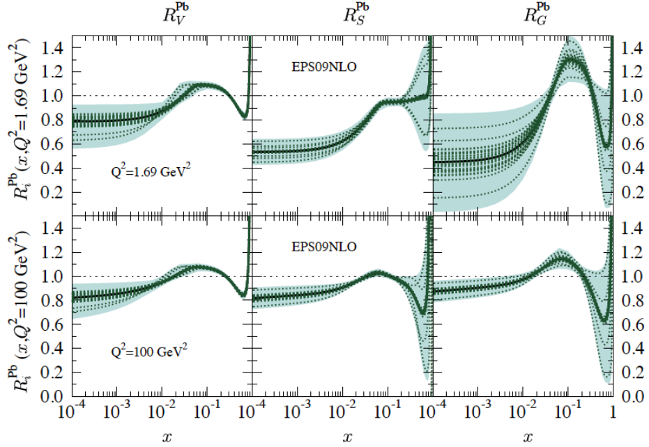
Figure 3.5. The nuclear modifications R_V, R_S, R_G for lead at the initial scale Q_0^2 = 1.69 \text{ GeV}^2 and Q_0^2 = 100 \text{ GeV}^2 . The thick black lines indicate the best-fit results, while the dotted green curves denote the error sets. The shaded bands are estimated from the experimental uncertainties of the fitted data. From [102].
