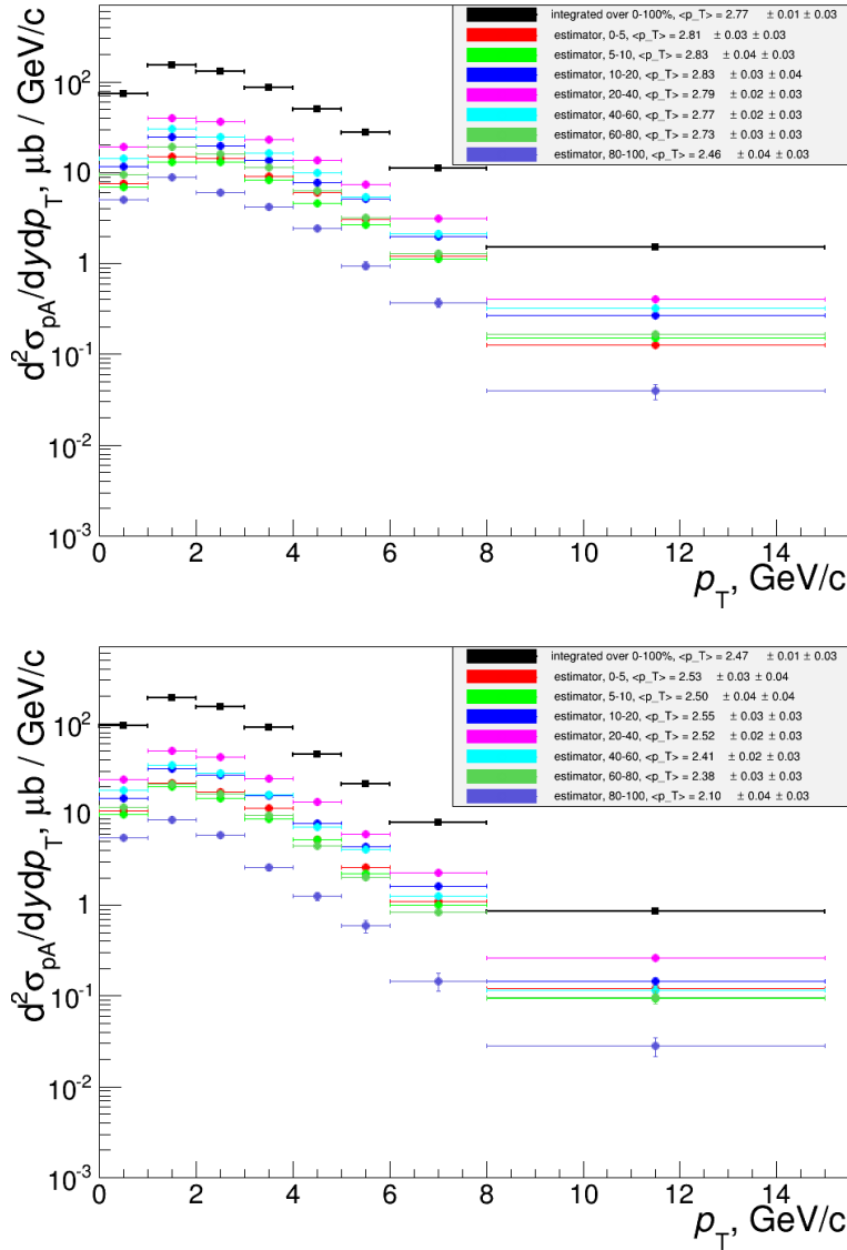
Figure 7.12. d^2\sigma_{pPb}/dydp_T as a function of p_T for different V0A event activity classes in p-Pb (top) and Pb-p (bottom), with SPD pile-up cut: n = 5 , d = 6\text{mm}
