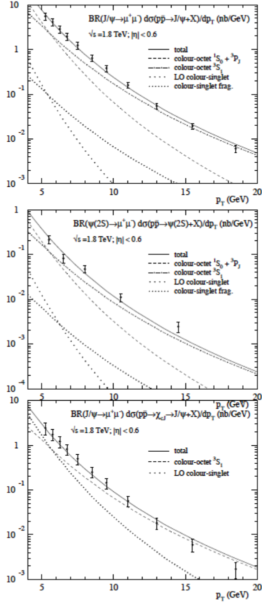
Figure 1.3. Top panel: Differential cross sections for the direct J/\psi production in \text{pp} \rightarrow J/\psi + X at the Tevatron ( \sqrt{s} = 1.8 TeV, pseudorapidity cut |\eta| < 0.6 ) compared to experimental data from CDF as a function of p_T . Middle panel: the same for the prompt \psi(2S) . Bottom panel: the same for the prompt J/\psi from decay of \chi_c . Dotted lines are the CSM contributions, the solid lines are the NRQCD factorization fits, other lines represent individual color-octet contributions to the fits. p_T is given in natural units. From [30].
