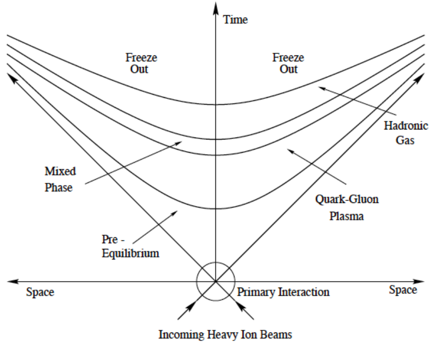
Figure 2.1. The space-time evolution of a heavy-ion collision, describing the formation of a QGP and the phase transition to ordinary matter. From [65].
