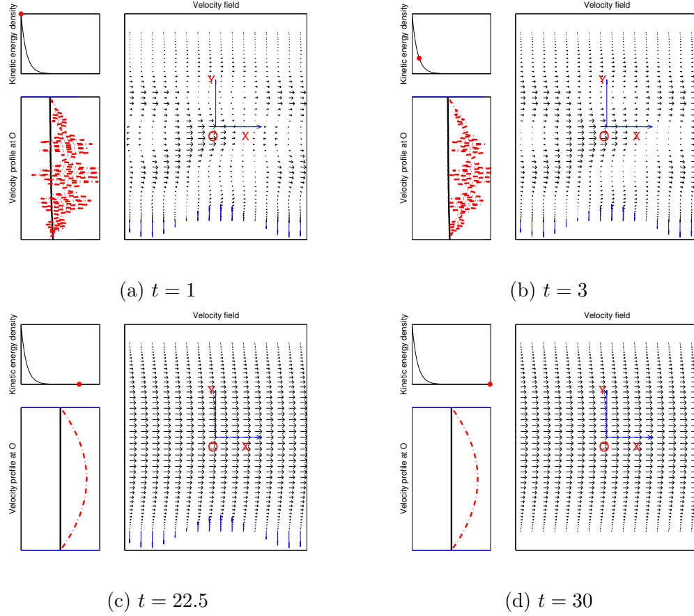
Figure 8.4: Shape of the flow perturbation in the controlled flow.
