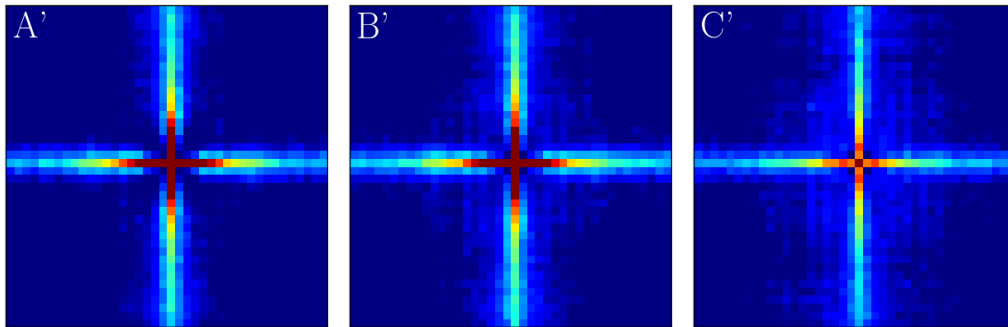
Figure 17.4: Colour maps of the plastic correlator \mathcal{C}_2 obtained with the FE-based model at \dot{\gamma} = 7 \cdot 10^{-4} for \langle\gamma_y\rangle = 0.05 and \langle\gamma_c\rangle = 0.015 . The time lags are (A') \Delta t = 0.5 , (B') \Delta t = 20 , (C') \Delta t = 60 . System size: 41 \times 41 macro-elements. Dark blue regions are anticorrelated, while dark red ones are strongly correlated. Note that an upper threshold has been imposed; without it, short-range correlations, at the centre, completely outshine the rest of the picture.
