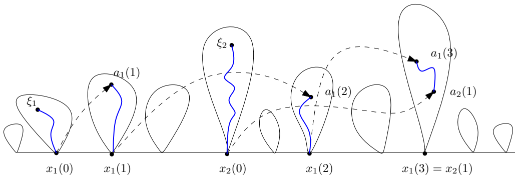
Figure 5.4 – An example with \mathcal{S}(1, 2) = 3 , \mathcal{S}(2, 1) = 1 and \text{mg}(1, 2) = 4 . The dashed lines indicate the point identifications for the root of the relevant subtrees.
