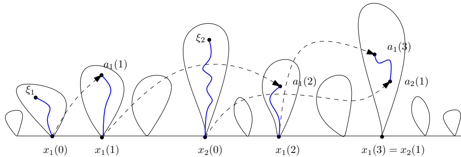
Figure 4.5 – An example with \mathcal{S}(1, 2) = 3 , \mathcal{S}(2, 1) = 1 and \text{mg}(1, 2) = 4 . The dashed lines indicate the identifications where the root of the relevant subtrees are sent to. The blue lines represent the location of the path between \xi_1 and \xi_2 before the transformation.
