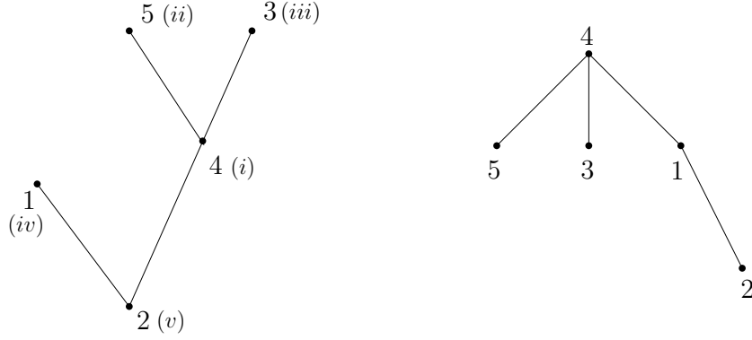
Figure 1.7 – On the left, a cutting of T^n where the roman numerals represent the order in which the vertices are removed. On the right, the corresponding \text{cut}(T^n) .
