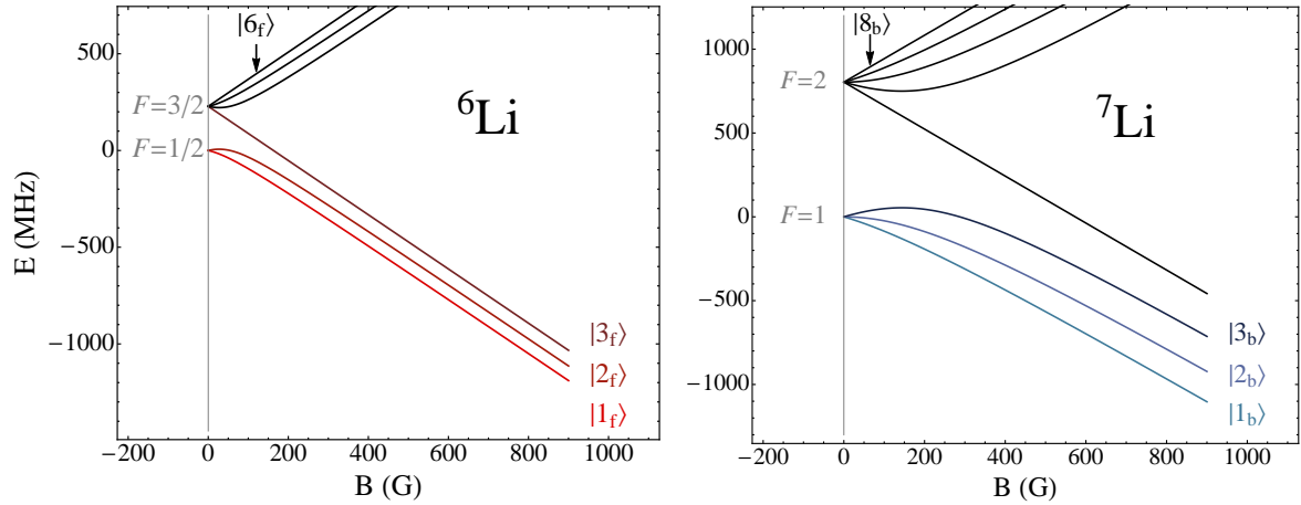
Figure 2.2: Magnetic field dependence of the energy levels of {}^6\text{Li} (left) and {}^7\text{Li} (right). The energy reference is taken to be the energy of the F = 1/2 , F = 1 manifolds at a zero field. For simplicity the states are labeled here |1_s\rangle , |2_s\rangle , ... and the index s indicates the isotope (b for {}^7\text{Li} and f for {}^6\text{Li} ). At low field, |1_f\rangle connects to |F = 1/2, m_F = 1/2\rangle and |6_f\rangle to |F = 3/2, m_F = 3/2\rangle for {}^6\text{Li} and for {}^7\text{Li} : |1_b\rangle connects to |F = 1, m_F = 1\rangle and |8_b\rangle to |F = 2, m_F = 2\rangle . During the magnetic trapping stages, the atoms are polarized in |6_f\rangle and |8_b\rangle . At the beginning of the optical trapping stage, they are transferred to the absolute ground states |1_f\rangle and |1_b\rangle by a radio-frequency rapid adiabatic passage.
