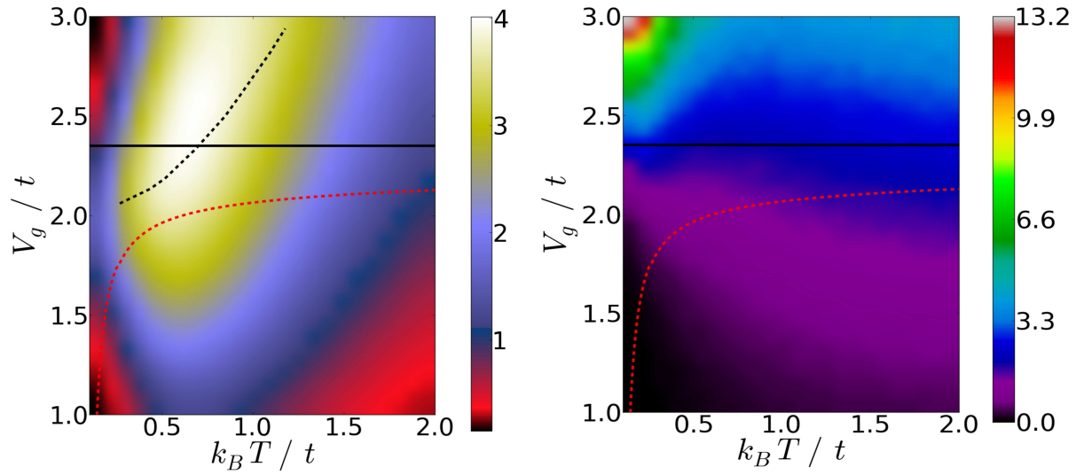
Figure 5.3: Rescaled power factor Q/M in unit of k_B^2/\hbar \approx 1.8 \times 10^{-12} W.K^{-2} (left panel) and electrical figure of merit Z_e T (right panel) as a function of k_B T and V_g (both in unit of t ). Data are shown in the large M limit ( M = 150 ) where both quantities have converged. Increasing V_g allows to scan the impurity band from the inside (below the horizontal full lines) to the outside (above). The black dashed line in the left panel indicates the contour along which S_0 = 2k_B/e , and lies within the region of maximal power factor (see text). The red dashed line in both panels is the Mott temperature (see Eq. (4.3) and Fig. 4.3), separating the Nearest Neighbor Hopping from the Variable Range Hopping regimes. Parameters: W = t, \gamma_e = \gamma_{ep} = t and L = 450 .
