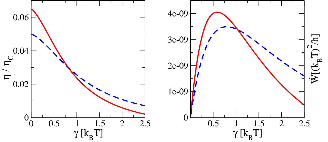
Figure 6.6: Left panel: Efficiency \eta , normalized over the Carnot limit, as a function of the coupling energy \gamma . Right panel: Output power \dot{W} extracted from the system, as a function of the coupling energy \gamma . In both cases, the full red curves correspond to a three-terminals configuration with \gamma_2 = 0.5\gamma , while the dashed blue curve refer to the two-terminals case ( \gamma_2 = 0 ). Parameters: E_d - \mu = 2.0 k_B T , \Delta\mu_1 = -\Delta\mu_2 = -10^{-4} k_B T , \Delta T_1 = 10^{-3} T , and \Delta T_2 = 0 .
