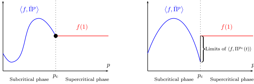
Figure 6.2: A schematic representation of the long time behaviour of \langle f, \Pi^p(t) \rangle according to Proposition 6.3.4. On the left-hand figure, \lim_{p \uparrow p_c} \langle f, \Pi^p \rangle = f(1) , so that \lim_{t \rightarrow +\infty} \langle f, \Pi^{p_c}(t) \rangle exists and its value is represented by the black dot. On the right-hand figure, \lim_{p \uparrow p_c} \langle f, \Pi^p \rangle \neq f(1) and the limit points of \langle f, \Pi^{p_c}(t) \rangle are located inside the gap between \lim_{p \uparrow p_c} \langle f, \Pi^p \rangle = \langle f, \Pi^{p_c} \rangle and f(1) .
