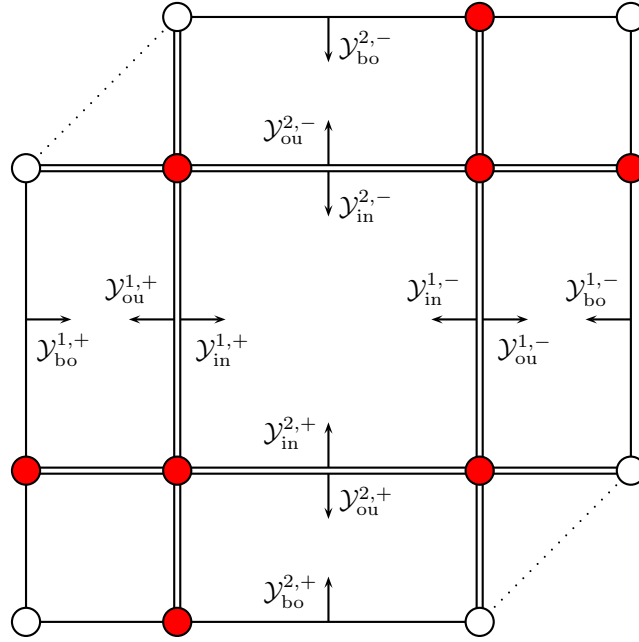
Figure 3.6: The solid lines represent the elementary sections \{\mathcal{Y}_\star^{i,\epsilon} : (i, \epsilon, \star) \in \Pi\} . Arrows stand for the sign of the normal component of the velocity of configurations in a given elementary section. White dots are excluded from \mathcal{X}_{\text{nd}} , while red dots correspond to the set \mathcal{N} .
