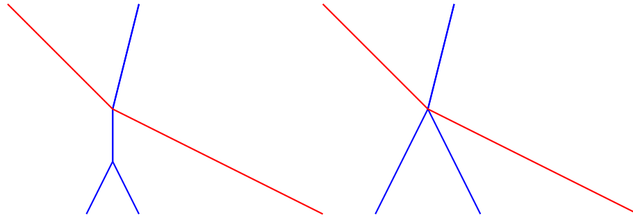
Figure 9.2: The left-hand side of the picture shows the trajectory of the MSPD started at a good configuration , since self-interaction space-time points are separated from collisions. On the contrary, the right-hand side of the picture shows the trajectory of the MSPD started at a configuration that cannot be good, since two distinct clusters of the same type have a self-interaction at the same time as they collide with a cluster of another type.
