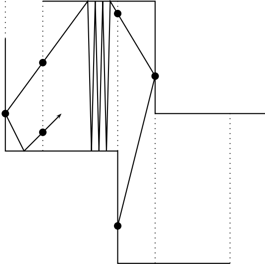
Figure 3.5: The boundaries of the bands are drawn in dotted lines. An example of a trajectory of the unfolded process is drawn in solid line. Each dot stands for an observation time. Between two consecutive observation times, the horizontal and vertical components evolve independently.
