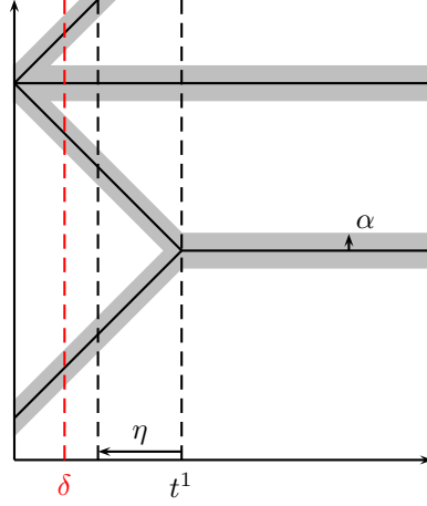
Figure 8.4: If some particles share the same initial position but instantaneously split into several clusters, \delta is fixed in (0, t^1 \wedge T) and \eta, \alpha are taken small enough for (8.8) to hold.
