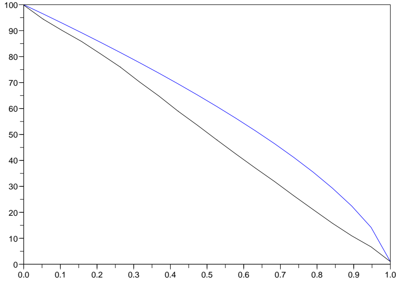
Figure 2.5: Experimental profile of \mathcal{T} for N = 20 molecules, in the weak interaction regime a = 0.001 . The theoretical profile (2.9) is plotted in blue. The experimentally observed profile is plotted in black and is linear.
