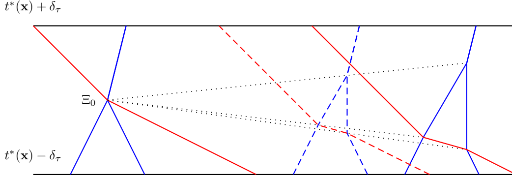
Figure 9.5: The trajectory of the MSPD started at \mathbf{x} is plotted on the left-hand side of the figure, while the trajectory of the MSPD started at \mathbf{y} is plotted on the right-hand side. The trajectory of the process \Phi' is plotted in dashed lines. Each linear part is parallel to the corresponding part in the trajectory of the MSPD started at \mathbf{y} . The black lines represent the horizontal sides of the box.
