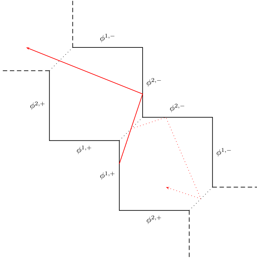
Figure 3.4: A part of the unfolded billiard table \tilde{\Omega} . The update densities associated with each thermalised wall are indicated. The reminiscent oblique facets are drawn in dotted line, but are no longer seen by the unfolded process. A trajectory of the unfolded process is plotted in red, the corresponding original trajectory is plotted in dotted line.
