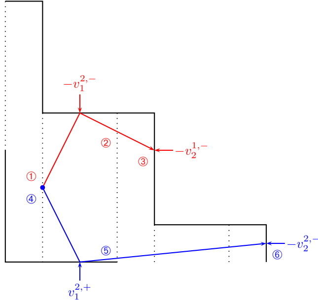
Figure 3.10: The possible cases for Y_{n_0} \in \mathcal{Y}_{\text{in}}^{1,+} . The red trajectory describes the case p^2 > 0 , while the blue trajectory describes the case p^2 < 0 . The circled digits indicate the situation dealt with: in situations ① and ④, \gamma \geq \eta_{\text{bo}}^{1,+} and N = n_0 . In situations ② and ⑤, \gamma < \eta_{\text{bo}}^{1,+} , \gamma' \geq \theta and N = n_0 + 1 . In situations ③ and ⑥, \gamma < \eta_{\text{bo}}^{1,+} , \gamma' < \theta and N = n_0 + 2 in the red case, N = n_0 + 4 in the blue case.
