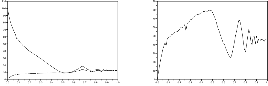
Figure 2.4: Left-hand: experimental values of \langle p_1^2 \rangle and \langle p_2^2 \rangle for T_L = 100 , T_R = 1 and a ranging from 0 to 1. When a grows to 1/2 (moderate interactions), the steady state temperatures of both molecules equilibrate. For a \geq 1/2 (strong interactions), the common temperature of the molecules exhibits an unexpected oscillatory behaviour. Right-hand: experimental value of the current j^2 for T_L = 100 , T_R = 1 and a ranging from 0 to 1. In the moderate interaction regime, the intensity of the current increases. In the strong interaction regime, the same oscillatory behaviour as for the temperatures is observed.
