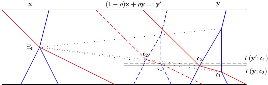
Figure 9.6: The configurations \mathbf{y} and \mathbf{y}' := (1 - \rho)\mathbf{x} + \rho\mathbf{y} are both good configurations and they are locally homothetic to \mathbf{x} . In their collision graph, \mathbf{c}_1 \rightarrow \mathbf{c}_2 ; however, for the choice of \rho on the figure, then T(\mathbf{y}'; \mathbf{c}_1) > T(\mathbf{y}; \mathbf{c}_2) , therefore Condition (LHM-3a) is not satisfied by the pair \mathbf{y}, \mathbf{y}' .
