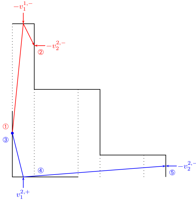
Figure 3.9: The possible cases for Y_{n_0} \in \mathcal{Y}_{\text{bo}}^{1,+} . The red trajectory describes the case p^2 > 0 , while the blue trajectory describes the case p^2 < 0 . The circled digits indicate the situation dealt with: in situations ① and ③, \gamma \geq \eta_{\text{bo}}^{1,+} and N = 0 . In situation ②, \gamma < \eta_{\text{bo}}^{1,+} and N = 1 . In situation ④, \gamma < \eta_{\text{bo}}^{1,+} , \gamma' \geq \theta and N = 1 . In situation ⑤, \gamma < \eta_{\text{bo}}^{1,+} , \gamma' < \theta and N = 5 .
