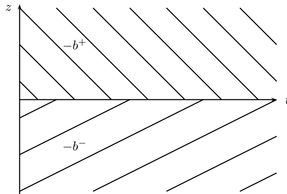
Figure 8.1: The characteristics of the conservation law in the diverging/diverging case. On the half line z = 0 , the value of u is a linear interpolation of the values given by the upward characteristic and the downward characteristic.
