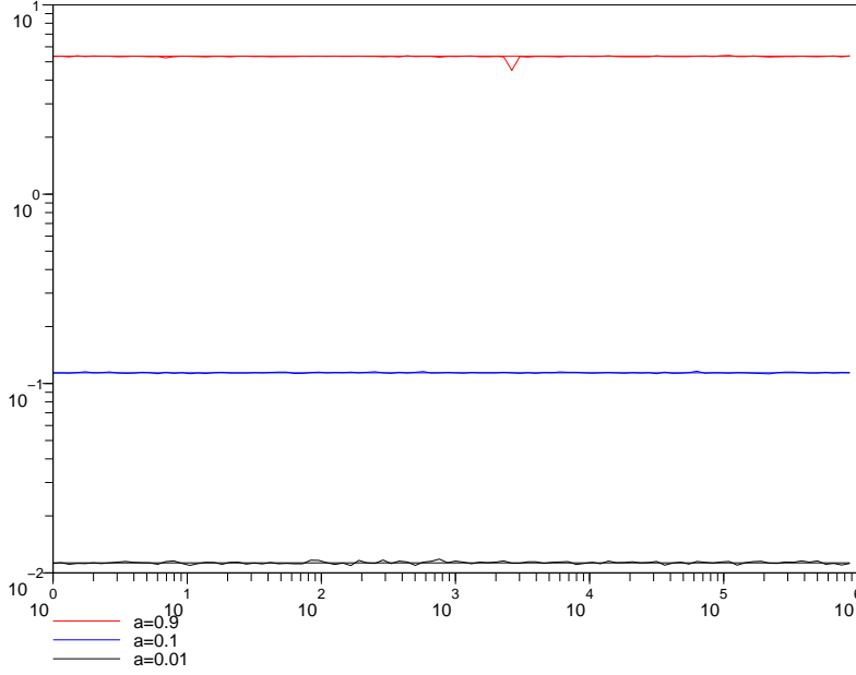
Figure 2.2: Frequency of collisions for a two-molecule system: for three values of a , namely a = 0.01 (weak interactions), a = 0.1 (moderate interactions) and a = 0.9 (strong interactions), the experimentally observed ratio \nu_{1,2}^2(a, T)/\sqrt{T} is plotted for T ranging from 1 to 10^6 . The theoretically expected value 2a/(\sqrt{\pi}(1-a^2)) of this ratio is superposed to the experimental results.
