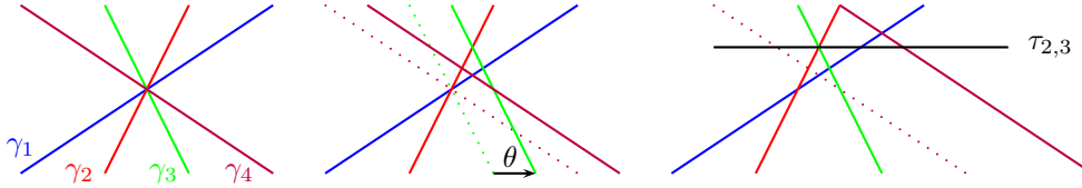
Figure 9.10: Blowing up the non-binary collisions: the left-hand figure represents a collision involving four clusters \gamma_1, \dots, \gamma_4 . In the central figure, the clusters \gamma_3 and \gamma_4 are shifted on the right of a distance \theta . In the right-hand figure, the cluster \gamma_4 is shifted on the right in order to ensure that its first collision with one of the three other clusters occurs after \tau_{2,3} , therefore after all the collisions between the clusters \gamma_1, \gamma_2 and \gamma_3 . The minimal shift distance remains proportional to \theta .
