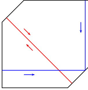
Figure 3.2: Two periodic orbits, corresponding to initial configuration such that one of the velocity components is null (blue trajectory) or 1 - a < q^1 + q^2 < 1 + a and p^1 + p^2 = 0 (red trajectory).
