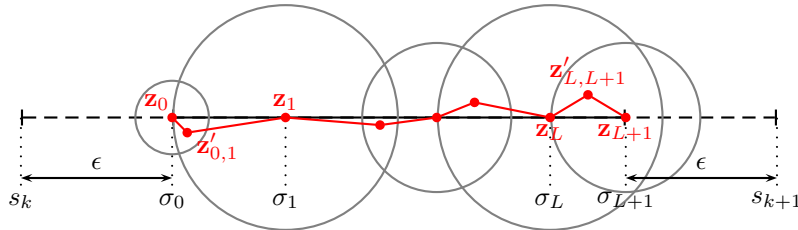
Figure 9.7 – The segment S_k is drawn in dashed line, while the segment S_k^\epsilon is drawn in solid line. Gray circles stand for the open balls B_1(\mathbf{z}_l, \kappa(\mathbf{z}_l)) . The points \mathbf{z}'_{0,1}, \dots, \mathbf{z}'_{L,L+1} are chosen in the dense set \mathcal{G} in order to ensure that the difference between the length of the red path and the length (s_{k+1} - s_k - 2\epsilon)\|\mathbf{x} - \mathbf{y}\| of S_k^\epsilon be smaller than \eta .
