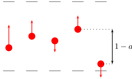
Figure 2.1 – The deterministic Complete Exchange Model, with N = 5 molecules.
