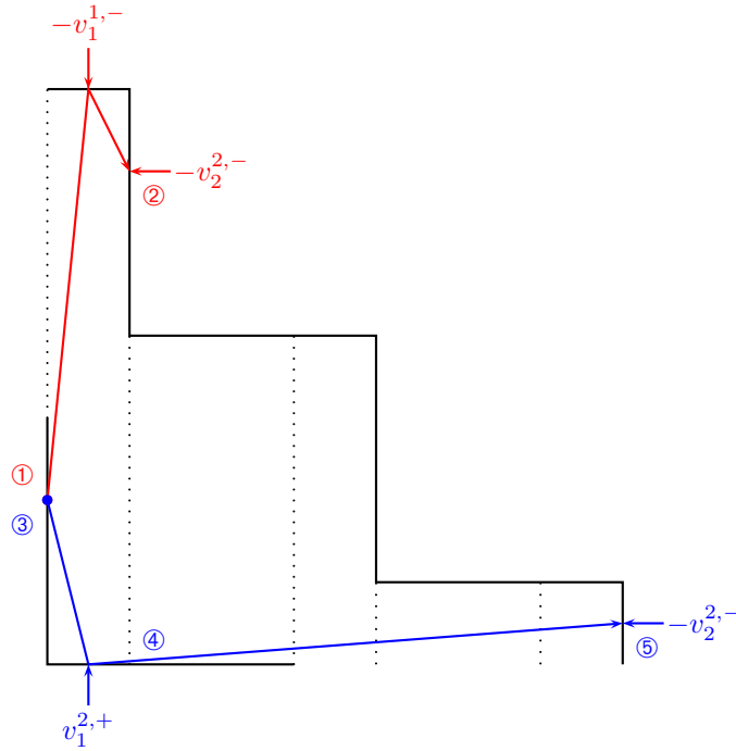
Figure 3.9 – The possible cases for Y_{n_0} \in \mathcal{Y}_{\text{bo}}^{1,+} . The red trajectory describes the case p^2 > 0 , while the blue trajectory describes the case p^2 < 0 . The circled digits indicate the situation dealt with: in situations ① and ③, \gamma \geq \eta_{\text{bo}}^{1,+} and N = 0 . In situation ②, \gamma < \eta_{\text{bo}}^{1,+} and N = 1 . In situation ④, \gamma < \eta_{\text{bo}}^{1,+} , \gamma' \geq \theta and N = 1 . In situation ⑤, \gamma < \eta_{\text{bo}}^{1,+} , \gamma' < \theta and N = 5 .
