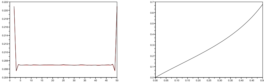
Figure 2.3 – Left-hand figure: for a chain of N = 50 molecules and a moderate interaction parameter a = 0.2 , the theoretical values of C_{i,i+1}^N(a)/\sqrt{\pi} along the chain is plotted in red. The superposed black graph corresponds to experimental observations of the ratio \nu_{i,i+1}^N(a, T)/\sqrt{T} at a fixed temperature T = 1 . Right-hand figure: theoretical value of C(a)/\sqrt{\pi} for a ranging from 0 to 1/2 . For small values of the interaction parameter, C(a) exhibits a linear growth with respect to a .
