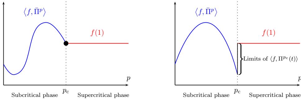
Figure 6.2 – A schematic representation of the long time behaviour of \langle f, \Pi^p(t) \rangle according to Proposition 6.3.4. On the left-hand figure, \lim_{p \uparrow p_c} \langle f, \Pi^p \rangle = f(1) , so that \lim_{t \rightarrow +\infty} \langle f, \Pi^{p_c}(t) \rangle exists and its value is represented by the black dot. On the right-hand figure, \lim_{p \uparrow p_c} \langle f, \Pi^p \rangle \neq f(1) and the limit points of \langle f, \Pi^{p_c}(t) \rangle are located inside the gap between \lim_{p \uparrow p_c} \langle f, \Pi^p \rangle = \langle f, \Pi^{p_c} \rangle and f(1) .
