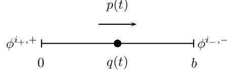
Figure 3.3 – The motion of a single molecule in the interval [0, b] .
