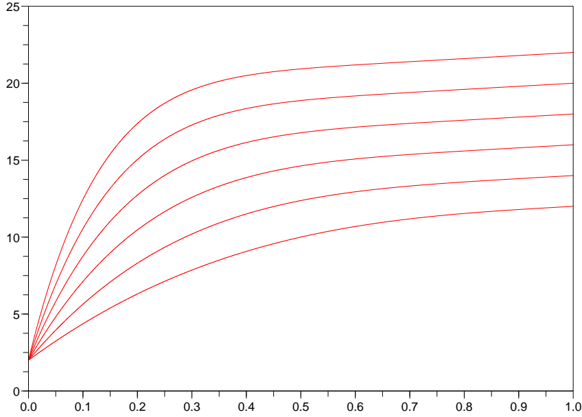
Figure 6.4 – The variance function \sigma^2 for g = 1 and \alpha taking integer values ranging from 3 (lowest curve) to 8 (highest curve).
