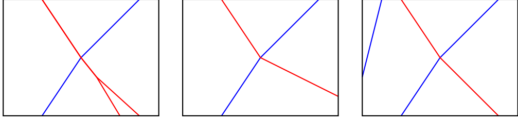
Figure 9.4 – The box on the left-hand figure contains a self-interaction at a distinct space-time point from the collision. On the central figure, a particle enters the box by a vertical side. The box on the right-hand figure is crossed by a particle that is not involved in the collision.
