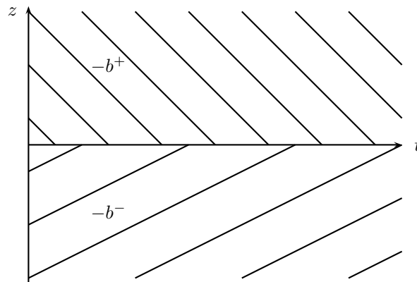
Figure 8.1 – The characteristics of the conservation law in the diverging/diverging case. On the half line z = 0 , the value of u is a linear interpolation of the values given by the upward characteristic and the downward characteristic.
