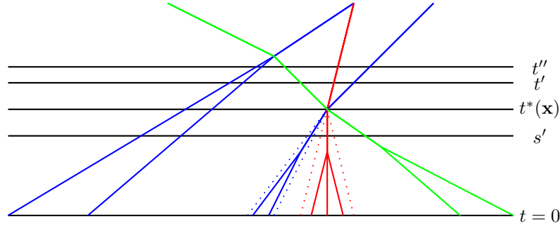
Figure 9.9 – The shrinking of particles having a self-interaction at time t^*(\mathbf{x}) allows to select s' < t^*(\mathbf{x}) such that there is no self-interaction on the time interval [s', t''] .
