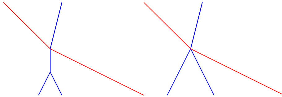
Figure 9.2 – The left-hand side of the picture shows the trajectory of the MSPD started at a good configuration , since self-interaction space-time points are separated from collisions. On the contrary, the right-hand side of the picture shows the trajectory of the MSPD started at a configuration that cannot be good, since two distinct clusters of the same type have a self-interaction at the same time as they collide with a cluster of another type.
