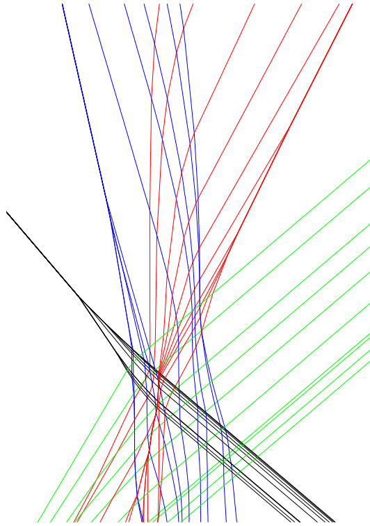
Figure 9.1 – A typical trajectory of the MSPD with d = 4 types and n = 10 particles per type. The horizontal coordinate refers to the physical positions of the particles, while the vertical coordinate describes the time. Each color is associated with a type of particle. Particles of the same type stick together at collisions, and the velocities may be modified at collisions with clusters of different types.
