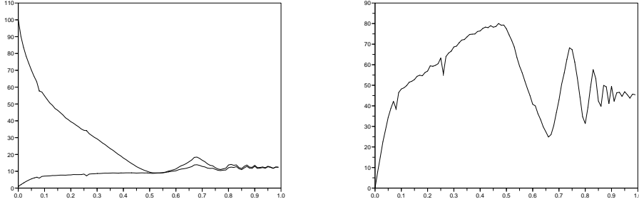
Figure 2.4 – Left-hand: experimental values of \langle p_1^2 \rangle and \langle p_2^2 \rangle for T_L = 100 , T_R = 1 and a ranging from 0 to 1. When a grows to 1/2 (moderate interactions), the steady state temperatures of both molecules equilibrate. For a \geq 1/2 (strong interactions), the common temperature of the molecules exhibits an unexpected oscillatory behaviour. Right-hand: experimental value of the current j^2 for T_L = 100 , T_R = 1 and a ranging from 0 to 1. In the moderate interaction regime, the intensity of the current increases. In the strong interaction regime, the same oscillatory behaviour as for the temperatures is observed.
