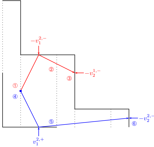
Figure 3.10 – The possible cases for Y_{n_0} \in \mathcal{Y}_{in}^{1,+} . The red trajectory describes the case p^2 > 0 , while the blue trajectory describes the case p^2 < 0 . The circled digits indicate the situation dealt with: in situations ① and ④, \gamma \geq \eta_{bo}^{1,+} and N = n_0 . In situations ② and ⑤, \gamma < \eta_{bo}^{1,+} , \gamma' \geq \theta and N = n_0 + 1 . In situations ③ and ⑥, \gamma < \eta_{bo}^{1,+} , \gamma' < \theta and N = n_0 + 2 in the red case, N = n_0 + 4 in the blue case.
