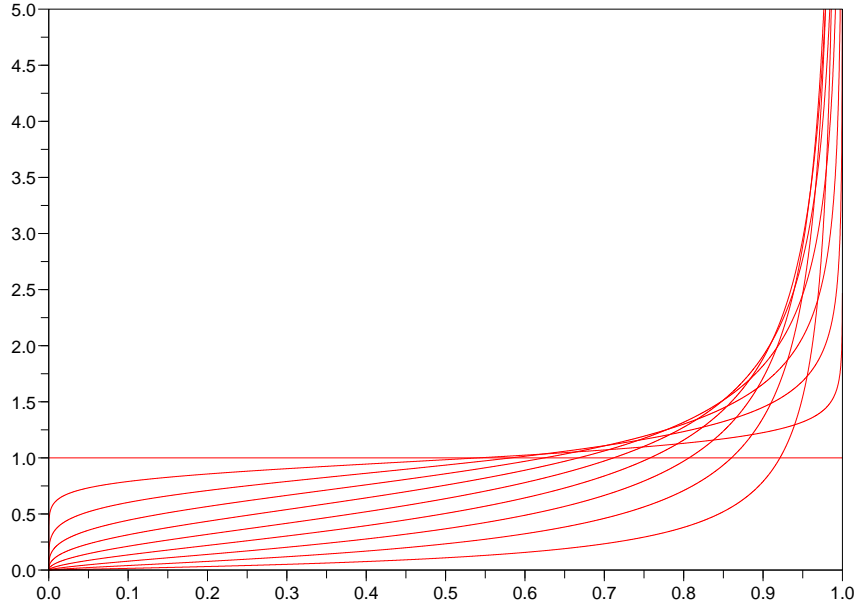
Figure 6.1 – The density of \bar{\Pi}^p for a constant variance function \sigma^2 and \gamma(u) = 1 - 2u . The diversity index p varies between 0 and p_c . The uniform density is recovered for p = 0 , while the mass concentrates on the point u = 1 when p approaches the critical diversity index p_c .
