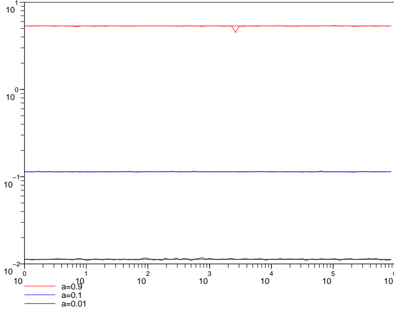
Figure 2.2 – Frequency of collisions for a two-molecule system: for three values of a , namely a = 0.01 (weak interactions), a = 0.1 (moderate interactions) and a = 0.9 (strong interactions), the experimentally observed ratio \nu_{1,2}^2(a, T)/\sqrt{T} is plotted for T ranging from 1 to 10^6 . The theoretically expected value 2a/(\sqrt{\pi}(1-a^2)) of this ratio is superposed to the experimental results.
