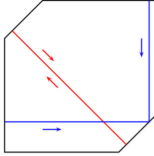
Figure 3.2 – Two periodic orbits, corresponding to initial configuration such that one of the velocity components is null (blue trajectory) or 1 - a < q^1 + q^2 < 1 + a and p^1 + p^2 = 0 (red trajectory).
