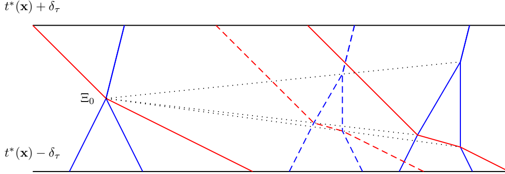
Figure 9.5 – The trajectory of the MSPD started at \mathbf{x} is plotted on the left-hand side of the figure, while the trajectory of the MSPD started at \mathbf{y} is plotted on the right-hand side. The trajectory of the process \Phi' is plotted in dashed lines. Each linear part is parallel to the corresponding part in the trajectory of the MSPD started at \mathbf{y} . The black lines represent the horizontal sides of the box.
