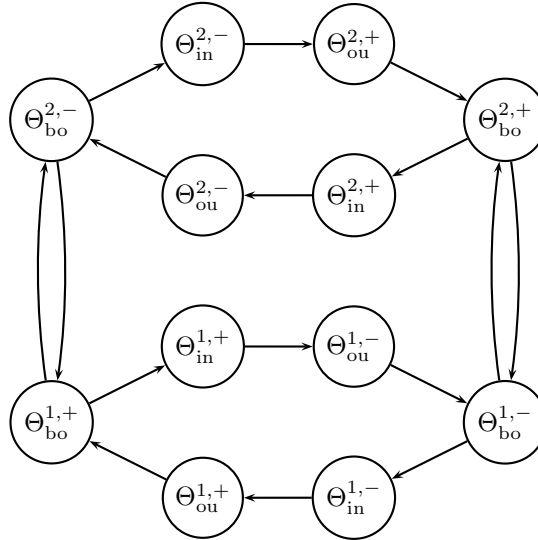
Figure 3.8 – The reduced graph. Each edge is associated with the positive weight \alpha((i, \epsilon, \star) \rightarrow (i', \epsilon', \star')) .
