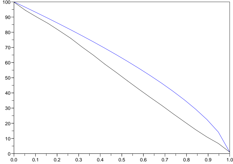
Figure 2.5 – Experimental profile of \mathcal{T} for N = 20 molecules, in the weak interaction regime a = 0.001 . The theoretical profile (2.9) is plotted in blue. The experimentally observed profile is plotted in black and is linear.
