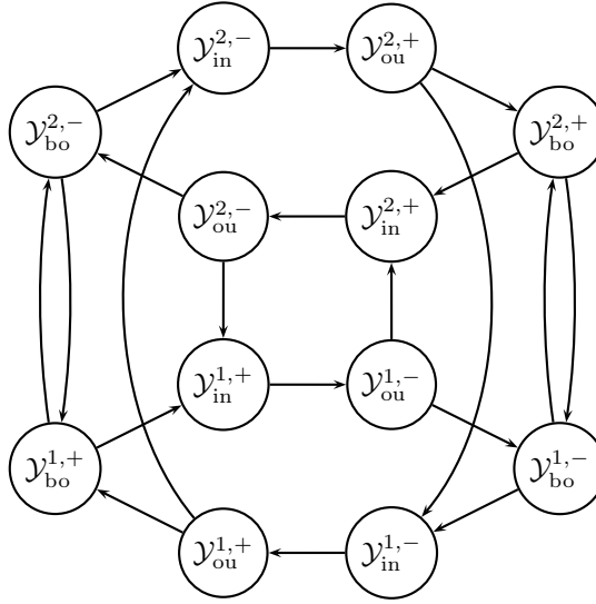
Figure 3.7 – The representation of the Markov kernel Q(y;\cdot) when the states are aggregated into elementary sections.
