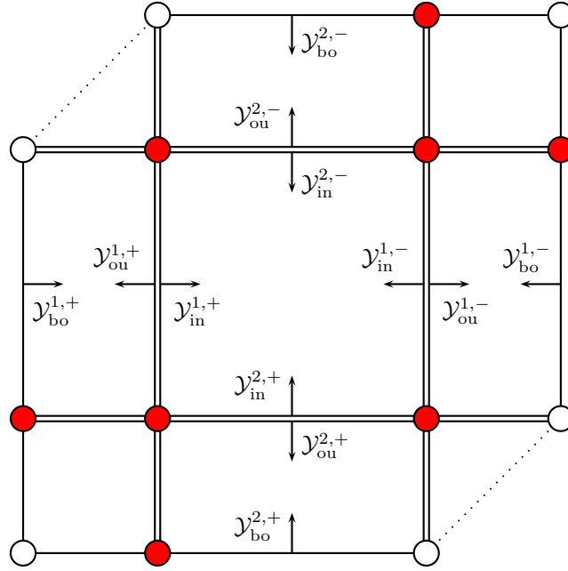
Figure 3.6 – The solid lines represent the elementary sections \{\mathcal{Y}_\star^{i,\epsilon} : (i, \epsilon, \star) \in \Pi\} . Arrows stand for the sign of the normal component of the velocity of configurations in a given elementary section. White dots are excluded from \mathcal{X}_{\text{nd}} , while red dots correspond to the set \mathcal{N} .
