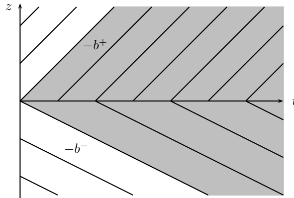
Figure 8.2 – The characteristics in the converging/converging case. In the gray area, the value of u is constant.
