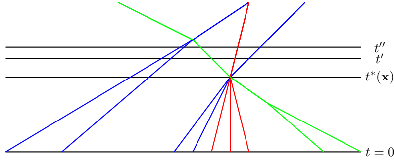
Figure 9.8 – The choices of t' and t'' to ensure that, on the time interval (t^*(\mathbf{x}), t''] , there is neither self-interaction nor collision in the MSPD started at \mathbf{x} .
