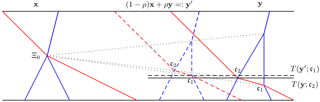
Figure 9.6 – The configurations \mathbf{y} and \mathbf{y}' := (1 - \rho)\mathbf{x} + \rho\mathbf{y} are both good configurations and they are locally homothetic to \mathbf{x} . In their collision graph, \mathbf{c}_1 \rightarrow \mathbf{c}_2 ; however, for the choice of \rho on the figure, then T(\mathbf{y}'; \mathbf{c}_1) > T(\mathbf{y}; \mathbf{c}_2) , therefore Condition (LHM-3a) is not satisfied by the pair \mathbf{y}, \mathbf{y}' .
