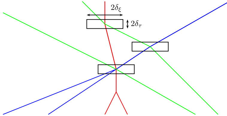
Figure 9.3 – An example of set of (\delta_\xi, \delta_\tau) -boxes around the points of I(\mathbf{x}) .
