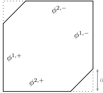
Figure 3.1 – The billiard table \bar{\Omega} . The update densities associated with each thermalised wall are indicated.
