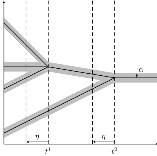
Figure 8.3 – A trajectory of the sticky particle dynamics \xi for n = 4 particles, with M = 2 collisions. The initial positions of the particles are pairwise distinct. For \eta > 0 such that 0 < t^1 - \eta < t^1 < t^2 - \eta , \alpha > 0 is chosen small enough for the set B_T(\xi, \alpha) to satisfy the condition (8.7). A path y in B_T(\xi, \alpha) is necessarily contained in the gray area.
