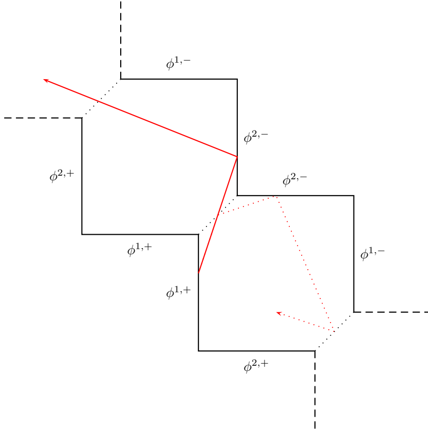
Figure 3.4 – A part of the unfolded billiard table \tilde{\Omega} . The update densities associated with each thermalised wall are indicated. The reminiscent oblique facets are drawn in dotted line, but are no longer seen by the unfolded process. A trajectory of the unfolded process is plotted in red, the corresponding original trajectory is plotted in dotted line.
