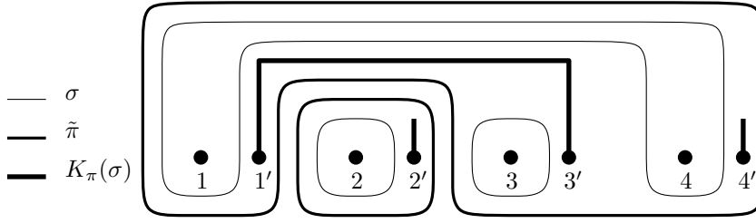
FIGURE 1. With \pi = \{\{1, 3, 4\}, \{2\}\} and \sigma = \{\{1, 4\}, \{2\}, \{3\}\} , we have K_\pi(\sigma) = \{\{1, 3\}, \{2\}, \{4\}\} .
