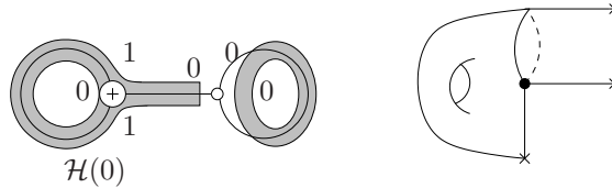
Figure 4.25: Configuration \mathcal{C}_2 of \mathcal{Q}(3, -1, -1, -1) containing cylinders, and its topological picture
