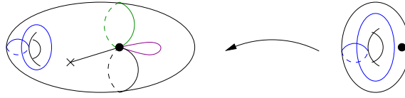
Figure 4.19: Family of curves associated to the configuration
