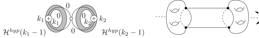
Figure 4.2: Configuration \mathcal{C}_1 for \mathcal{Q}^{\text{hyp}}(k_1^2, k_2^2)
