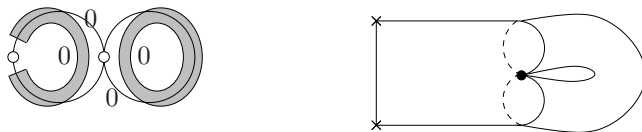
Figure 4.12: The only configuration of \mathcal{Q}(2, -1, -1) containing cylinders, and its topological picture
