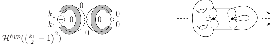
Figure 4.11: Additional configuration for \mathcal{Q}^{hyp}(2k_1 + 2, 2)
