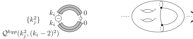
Figure 4.4: Configuration \mathcal{C}_2 for \mathcal{Q}^{hyp}(k_1^2, k_2^2)
