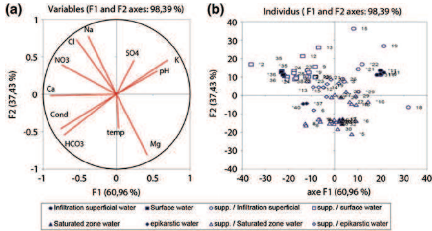
Fig. 3 Discriminant analysis (DFA) of the samples taken into the abutments and the drains of the dam and the lake. a Diagram of variables. b Diagram of individuals ( ^{\circ} 1: June 2002 campaign, 1: March 2004 campaign). N = 4 \times 4 , 59 supplementary elements
