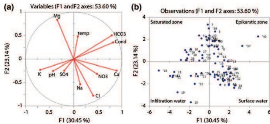
Fig. 2 Principal component analysis of the samples taken into the abutments and the drains of the dam and the lake. a Diagram variables. b Diagram of individuals (°1: June 2002 campaign, 1: March 2004 campaign)
