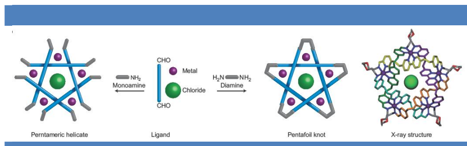
Figure 2 | One-pot synthesis of pentameric helicates (left) and a pentafoil knot (right) including X-ray crystallographic analysis that confirms the knotted topology. [9]
