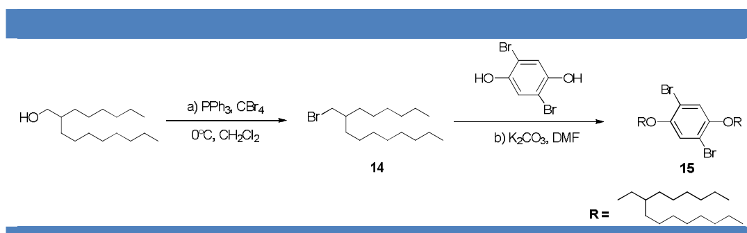
Scheme 7 | Synthesis of bis-ether 15 .
