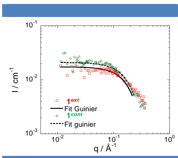
Figure 44 | SANS data for solutions of \mathbf{1}^{ext} and \mathbf{1}^{cont} (10 mM in 1:1 CDCl 3 /CD 3 CN at T=20°C). The dashed lines represent the best fits of the data obtained using a classical Guinier expression (eq. S14, see experimental part).
