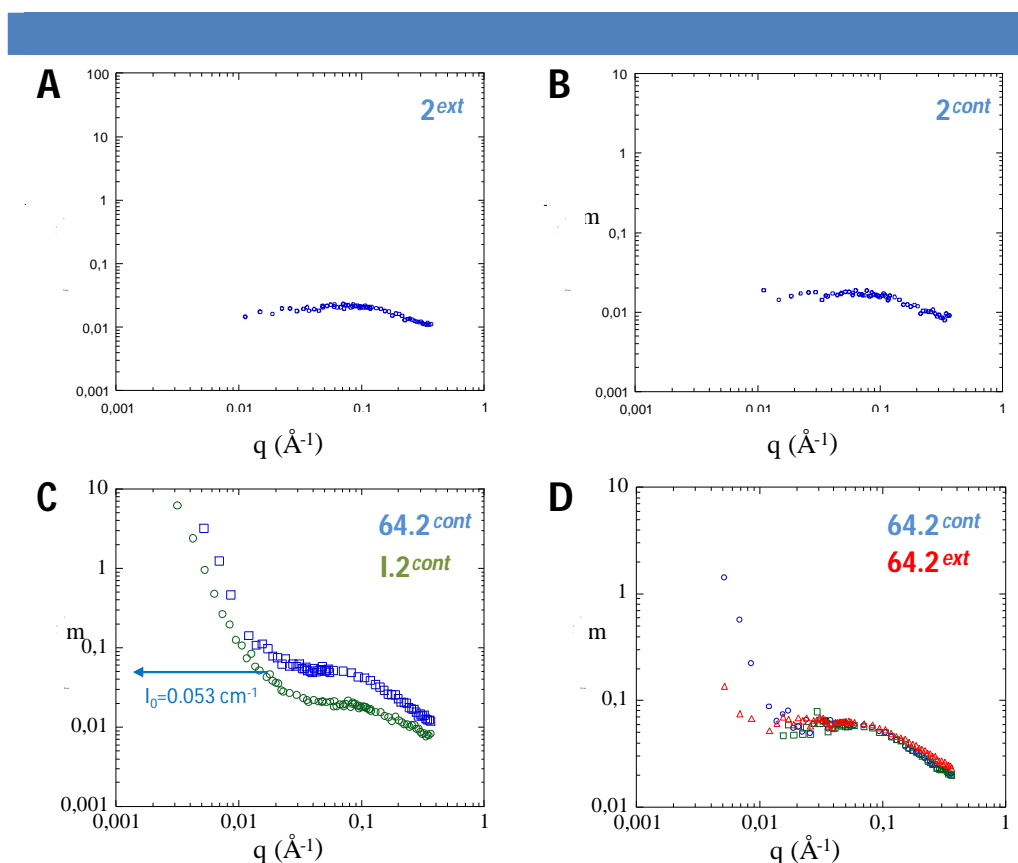
Figure 57 | SANS data of (A) monomer 2 ext , (B) monomer 2 cont , (C) H-bonding polymers [64•2] cont and [I•2] cont ; and (D) H-bonding polymers [64•2] cont and [64•2] ext (10 mM in 1:1 \text{CDCl}_3/\text{CD}_3\text{CN} at T=20^\circ\text{C} ).
