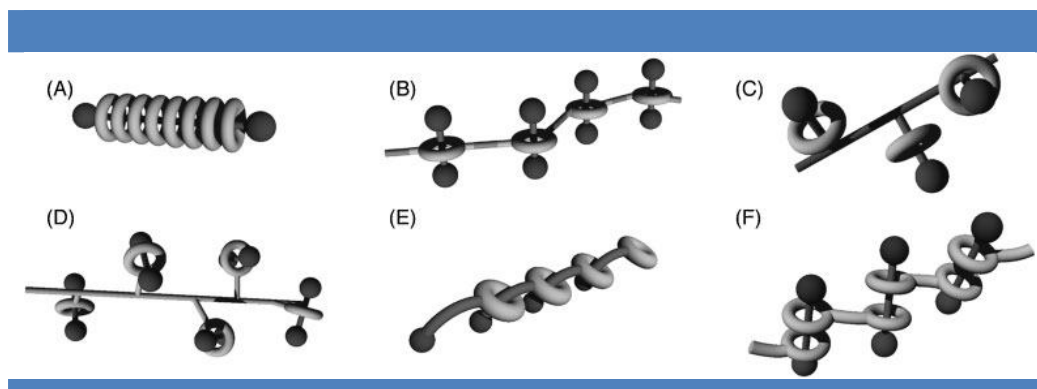
Figure 9 | Typical structures of polyrotaxanes. (A), (B) main chain-types, (C), (D) side chain-types, (E) daisy-chain type, and (F) poly[3]rotaxane. [26]
