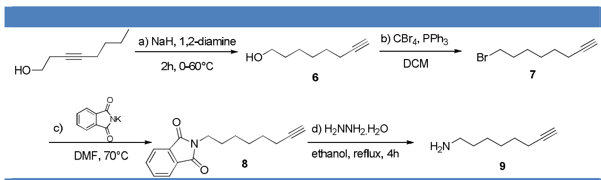
Scheme 4 | Synthesis of 8-aminooct-1-yne 9 . [64]
