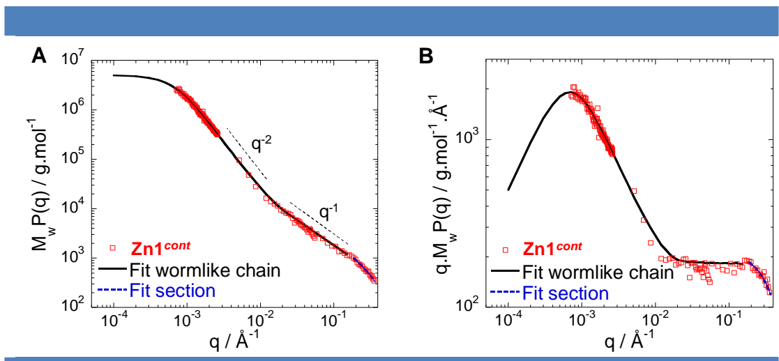
Figure 43 | (A) Log-Log plot of combined SLS and SANS measurements for a solution of Zn1 cont (10 mM in 1:1 CDCl 3 /CD 3 CN at T=20°C); (B) corresponding Holtzer plot. The continuous line represents the data fit by the wormlike chain model (eq. S10, see experimental part) and the dashed line represents the data fit at high- q by a Guinier expression for the form factor of the section (eq. S11, see experimental part).
