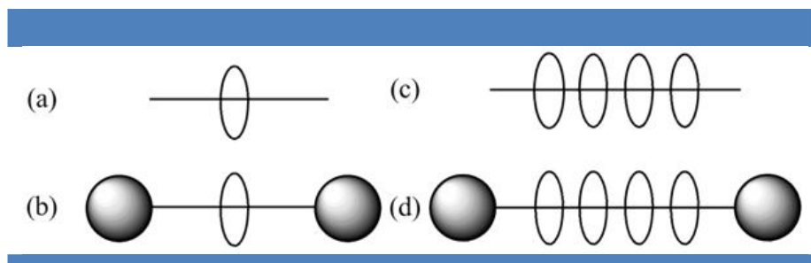
Figure 6 | A schematic representation of (a) a pseudorotaxane, (b) a [2] rotaxane, (c) a pseudopolyrotaxane, (d) a polyrotaxane. [19]
