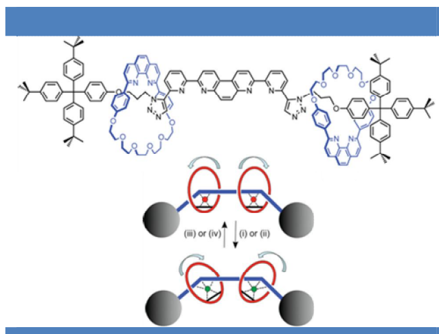
Figure 21 | (Cartoon representing the motions of the two binding macrocycles on a [3]rotaxane: (i) oxidation of Cu(I) to Cu(II), (ii) exchange of Cu(I) for \text{Zn}^{2+} , (iii) reduction of Cu(II) to Cu(I), (iv) exchange of \text{Zn}^{2+} for Cu(I). [55]
