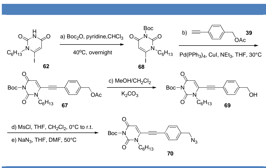
Scheme 32 | Synthesis of compound 70 .
