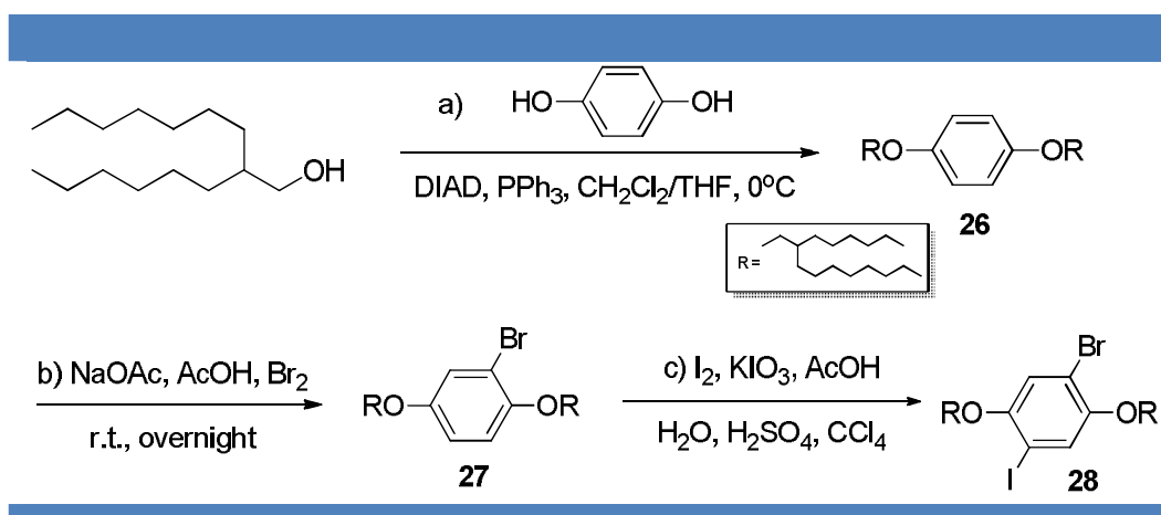
Scheme 15 | Synthesis of the mixed bromo-iodo derivative 28 .
