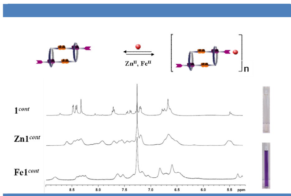
Figure 41 | Polymerisation of \mathbf{1}^{\text{cont}} with \text{Zn}(\text{II}) or \text{Fe}(\text{II}) ions.
