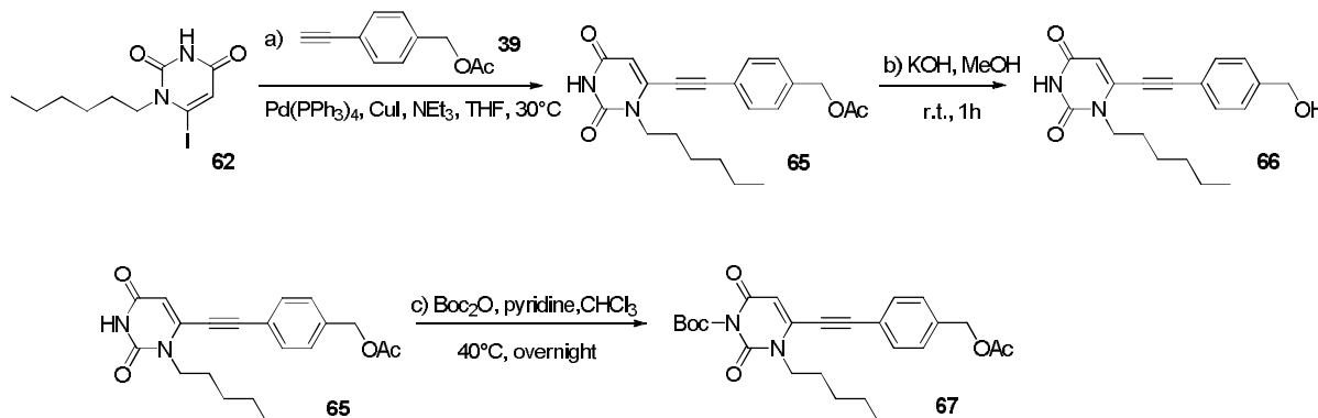
Scheme 31 | Synthesis of compound 67 .
