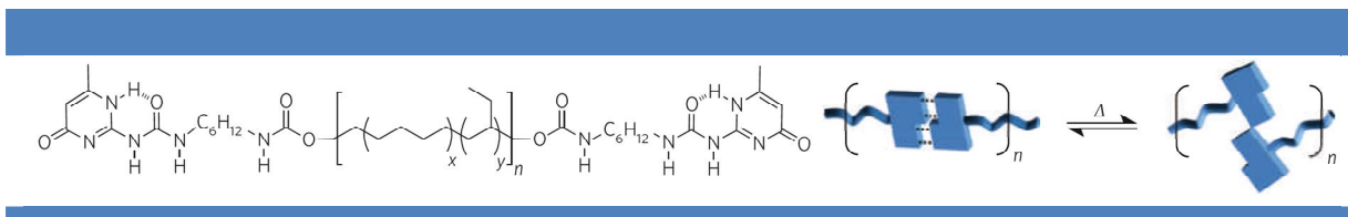
Figure 32 | The quadruple hydrogen-bonding unit UPy incorporated onto the chain ends of low-molecular-weight telechelic polymers as thermally responsive structurally dynamic polymers. [75]
