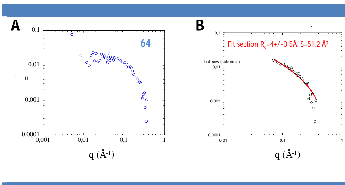
Figure 56 | SANS data (A) and corresponding fit (B) for a solution of 64 (10 mM in 1:1 \text{CDCl}_3/\text{CD}_3\text{CN} at T=20^\circ\text{C} ). The red line represents the best fit of the data obtained using a classical Guinier expression (eq. S14, see experimental part).
