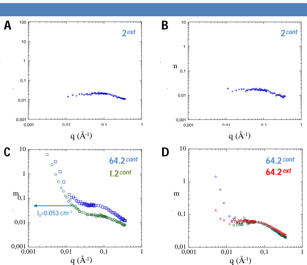
Figure 57 | SANS data of (A) monomer 2^{ext} , (B) monomer 2^{cont} , (C) H-bonding polymers [64 \cdot 2]^{cont} and [I \cdot 2]^{cont} ; and (D) H-bonding polymers [64 \cdot 2]^{cont} and [64 \cdot 2]^{ext} (10 mM in 1:1 CDCl_3/CD_3CN at T=20^\circ C ).
