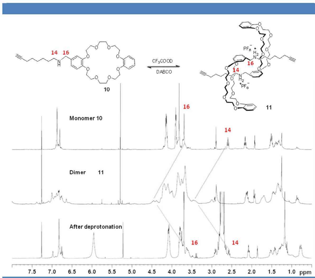
Figure 38 | Acid-base titration for the threading / unthreading of pseudorotaxane 11 .
